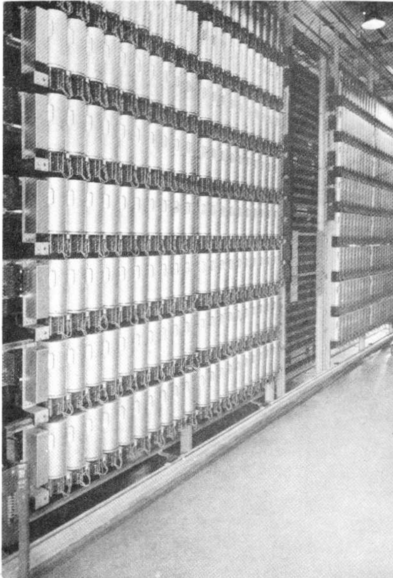
Figure 26 - Selector Frame
