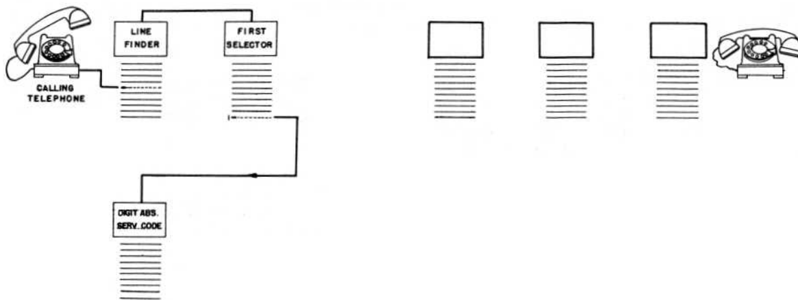
Sketch 9 Calling Subscriber Dials the Numerical Code (1793)
