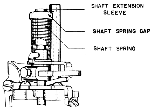
HELICAL TYPE SHAFT SPRING (NEW)
