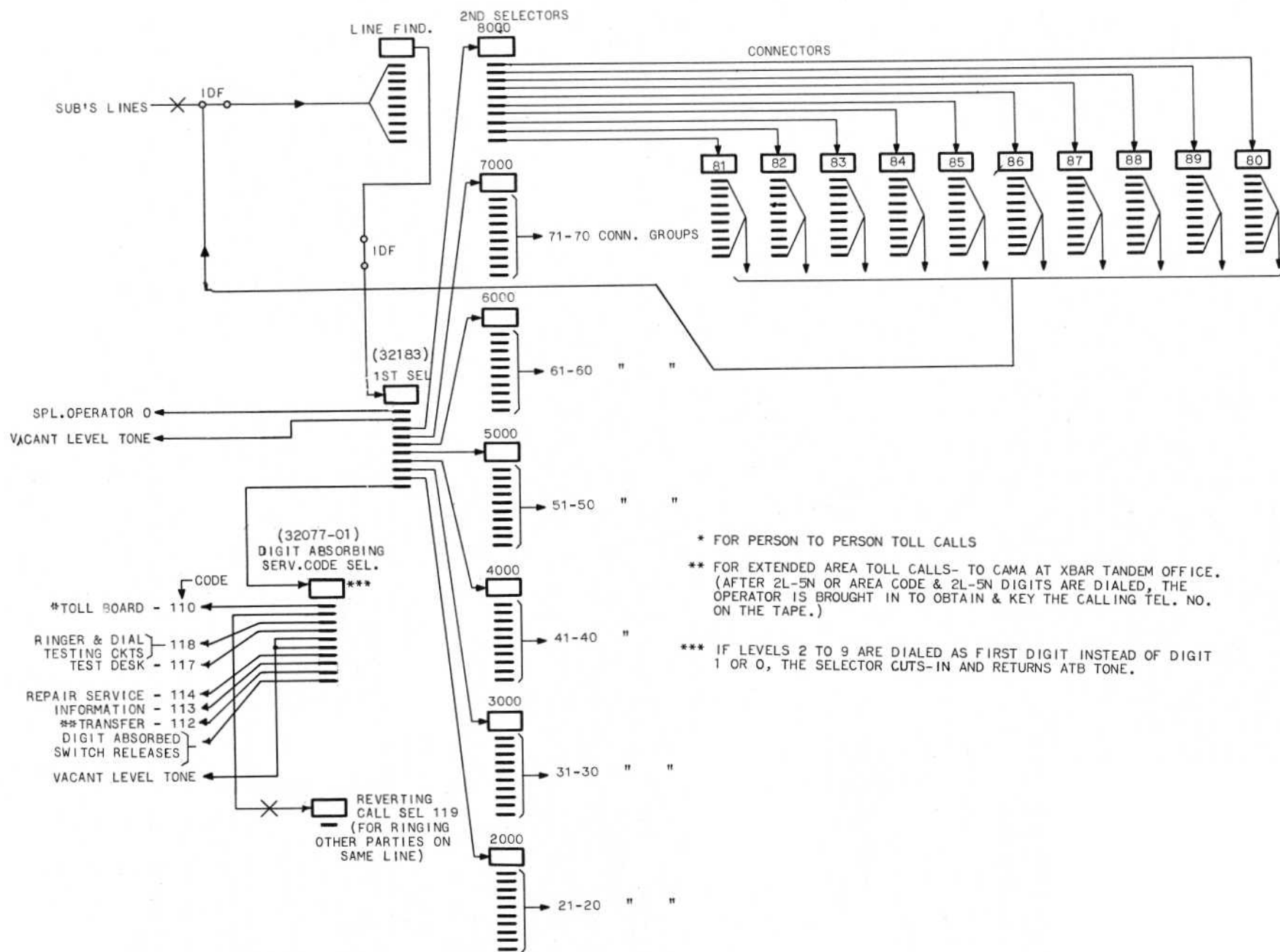
Figure E - Step-By-Step 4-Digit Office 7000 Lines Equipped
