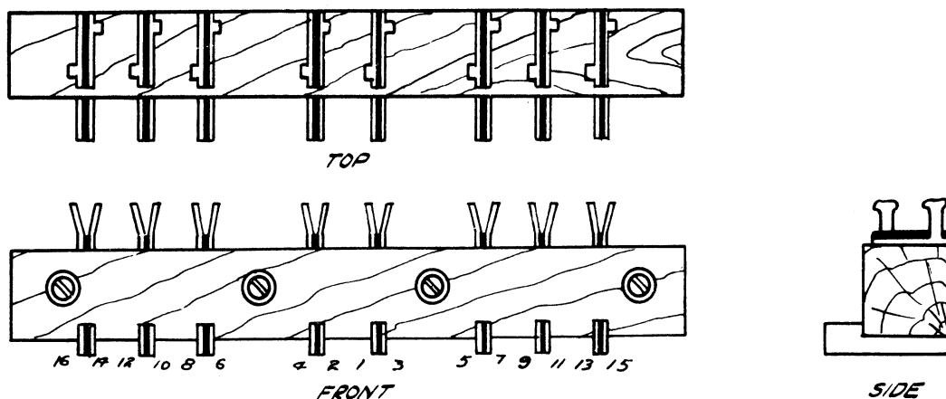
Figure 21 - Plug
