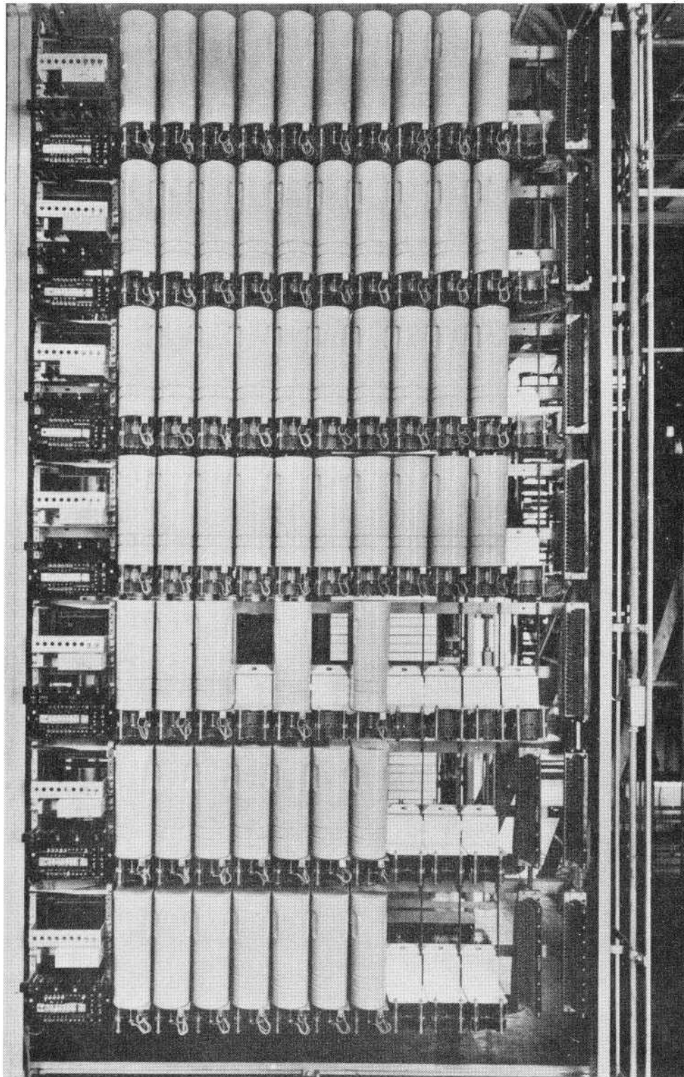
Figure 30 - Connector Frame
