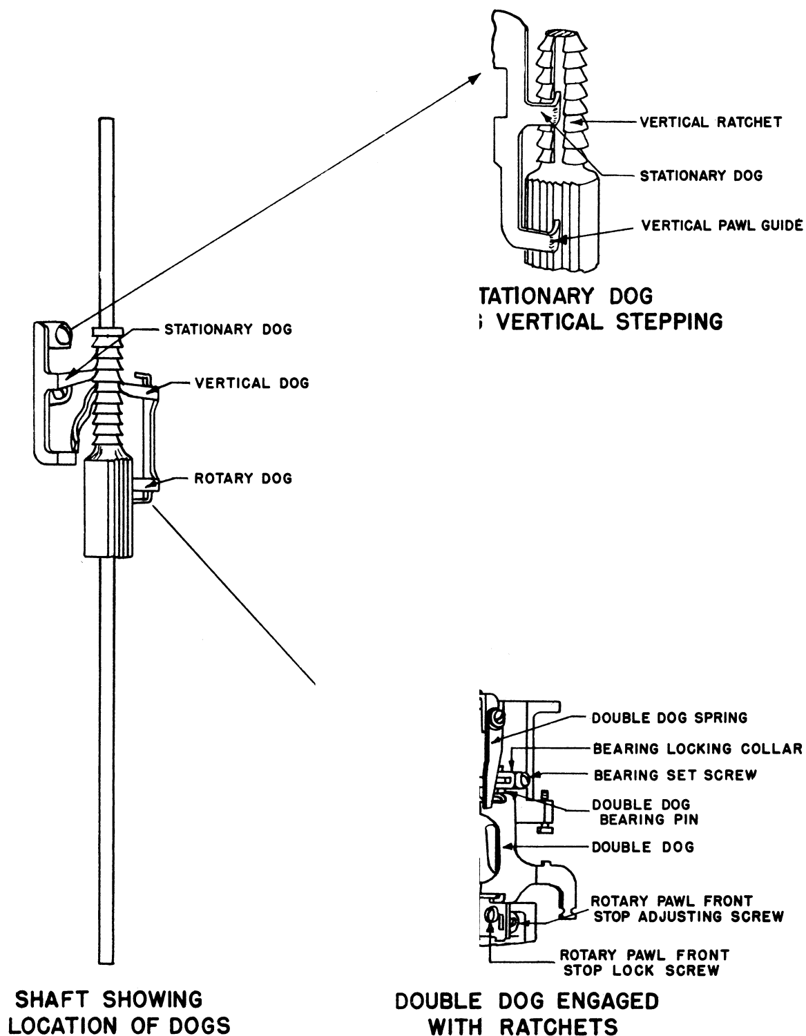
Figure 15 - Dogs
