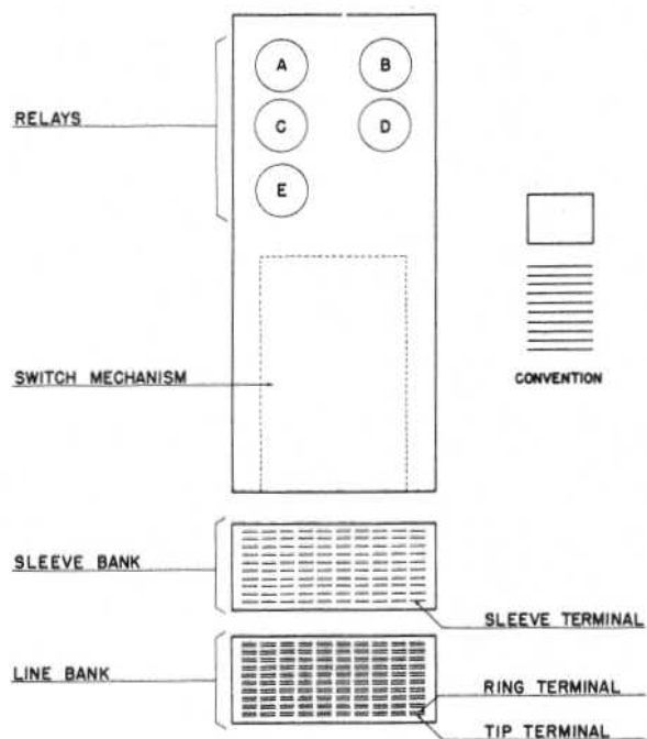
SELECTOR SWITCH
