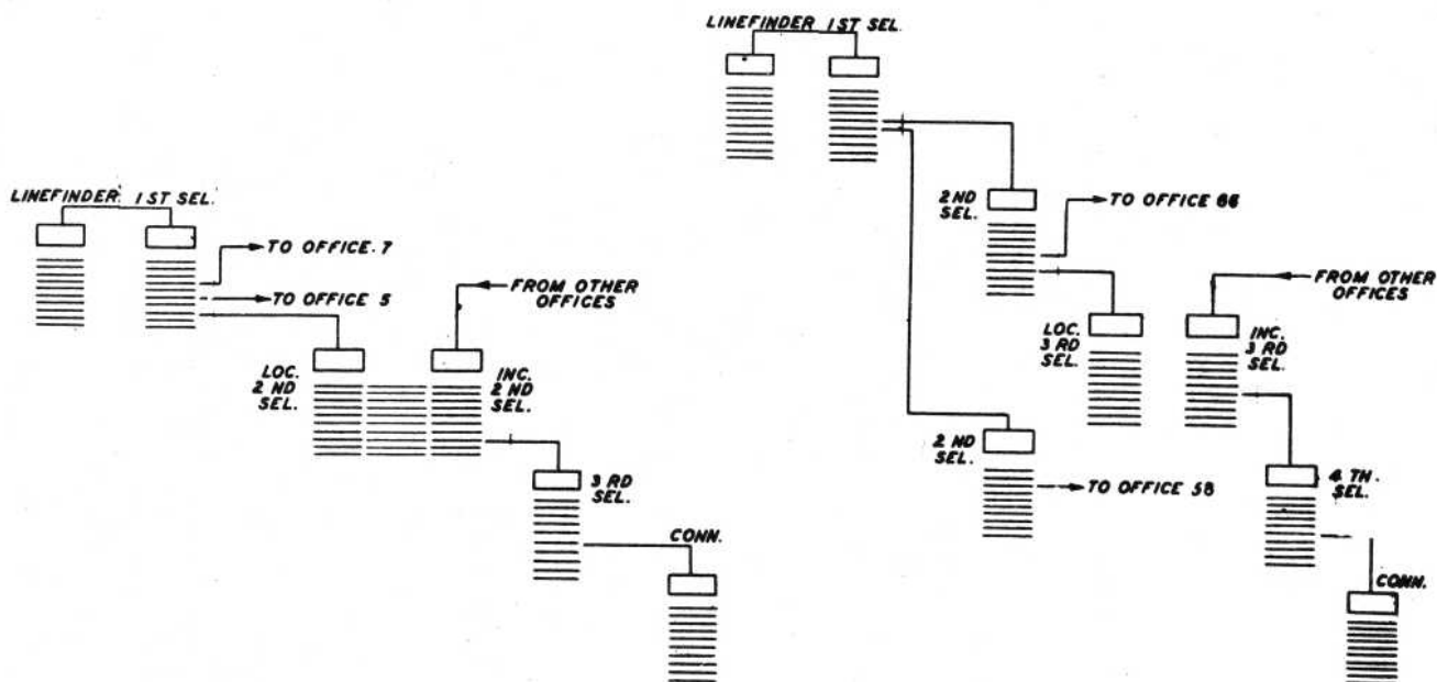
Figure H - "Step-By-Step System 6 Digit"
