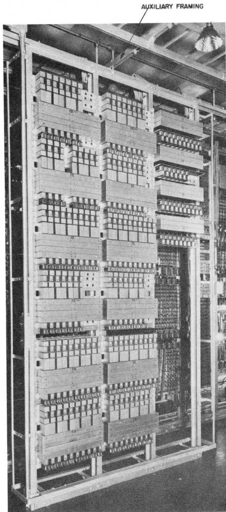
Figure 32 - Relay Racks
