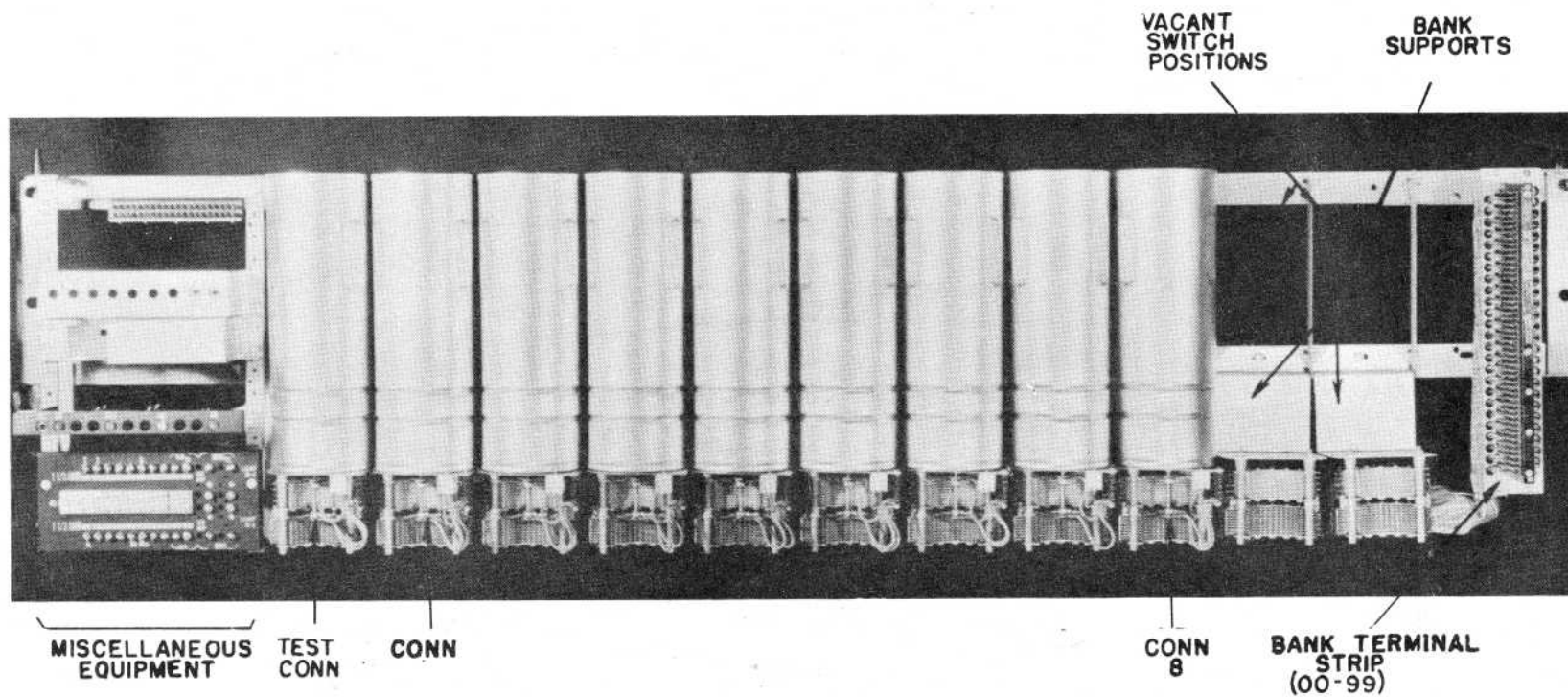
Figure 29 - Connector Shelf - 11 Switch
