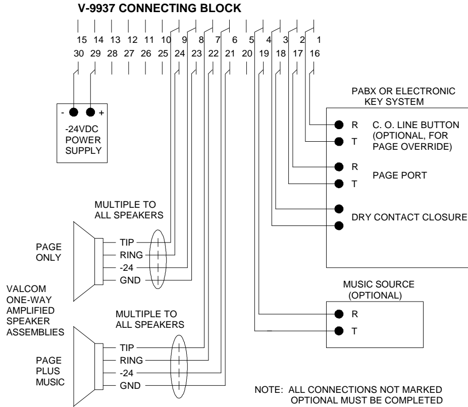
FIGURE 5 - WIRING CONNECTIONS FOR ARRANGEMENT 1
