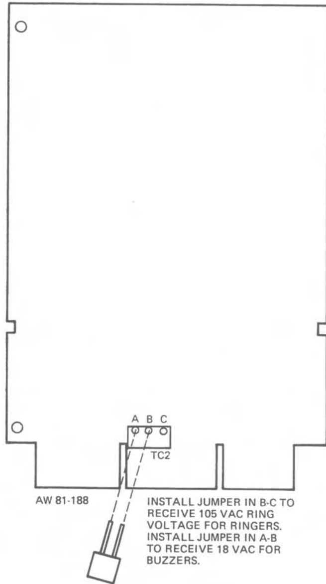
Figure 6: Interrupter Card
