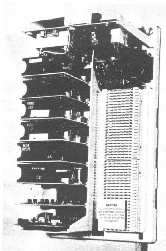
Figure 1: 601A Key Service Unit
