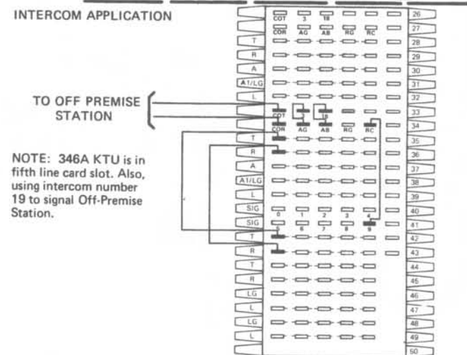
Figure 18: Connections to Add 346A Off-Premise Line
