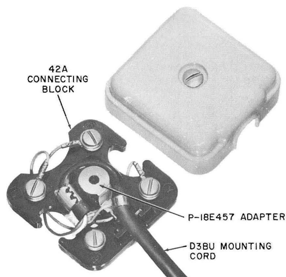
Fig. 6—42A Connecting Block with D3BU Mounting Cord
