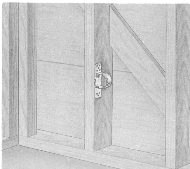
Fig. 14—Stud-Mounted 63A Bracket
