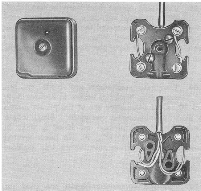
Fig. 1—42A Connecting Block
