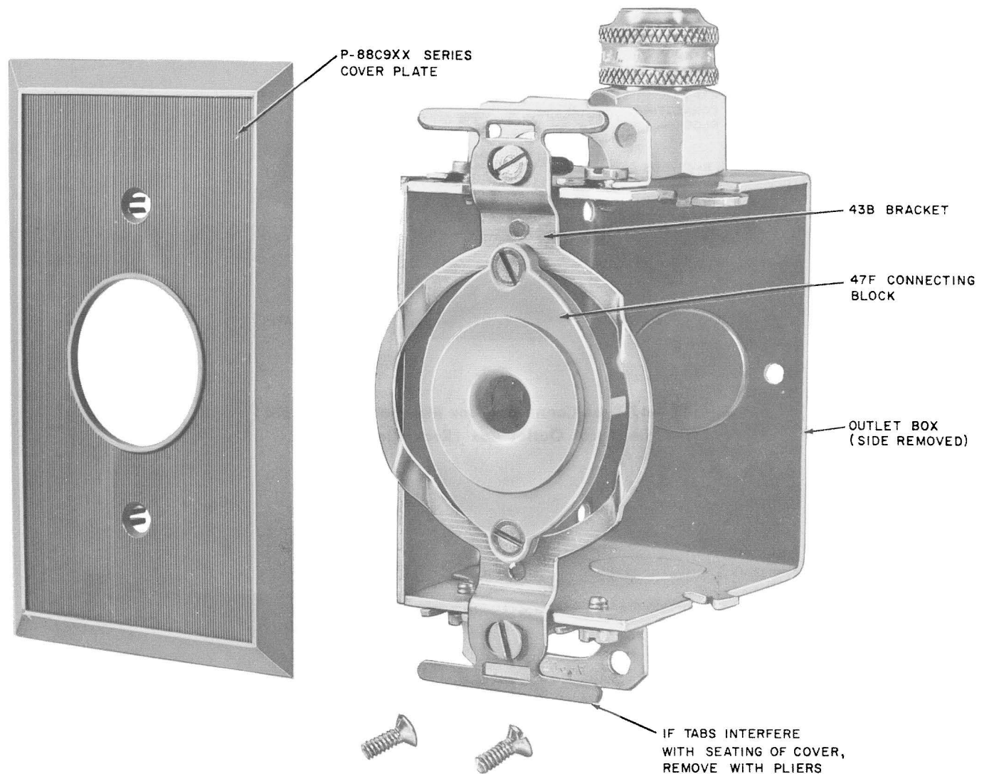
Fig. 11—47-Type Connecting Block Mounted in Standard Electrical Outlet Box (Front View)
