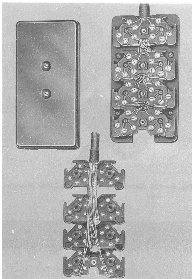
Fig. 8—Four 44A Connecting Blocks Mounted on a 168F Backboard and Equipped with a 101D Cover
