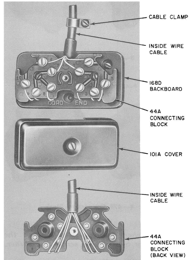
Fig. 2—1044A Connecting Block (44A Connecting Block and 101A Cover) with 168D Backboard
