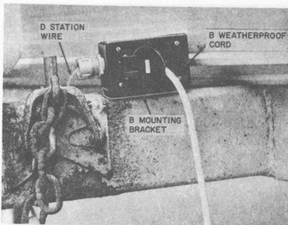
Fig. 17A—B Weatherproof Male Jack Mounted on Trailer Hitch
