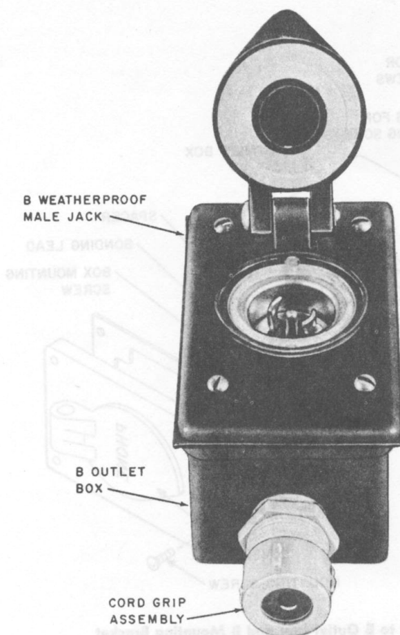
Fig. 7B—B Weatherproof Male Jack on B Outlet Box (Cover Open)
