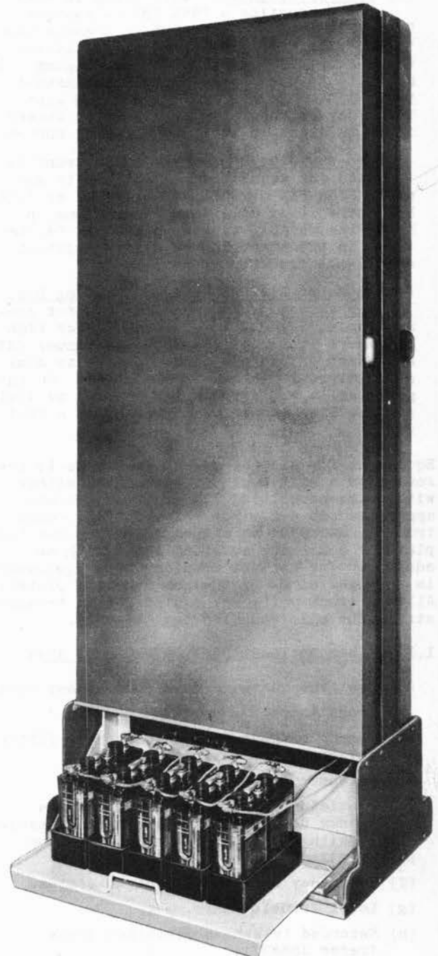
Fig. 4 - 755A PBX Showing Batteries in Position for Maintenance
