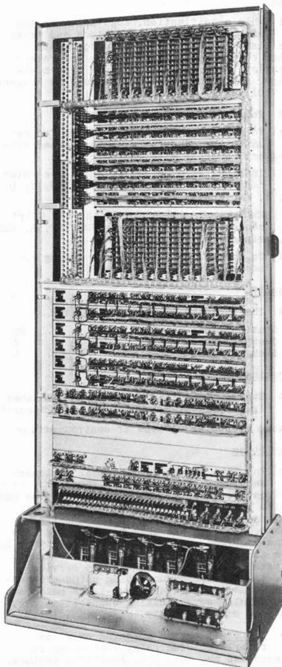
Fig. 3 - 755A PBX - Rear Casings Removed
