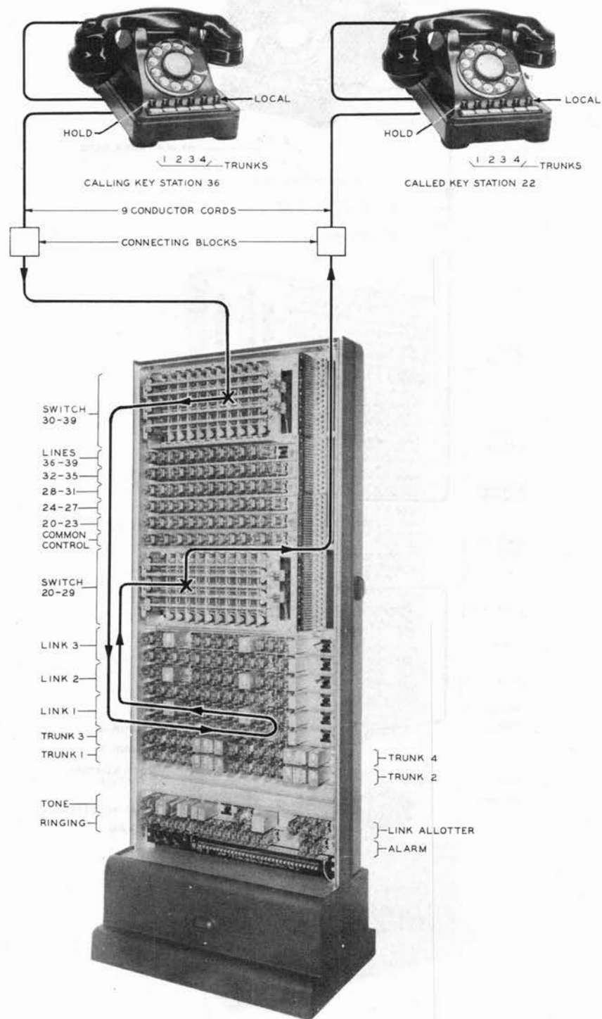
Fig. 5 - Local Station Calling Local Station
