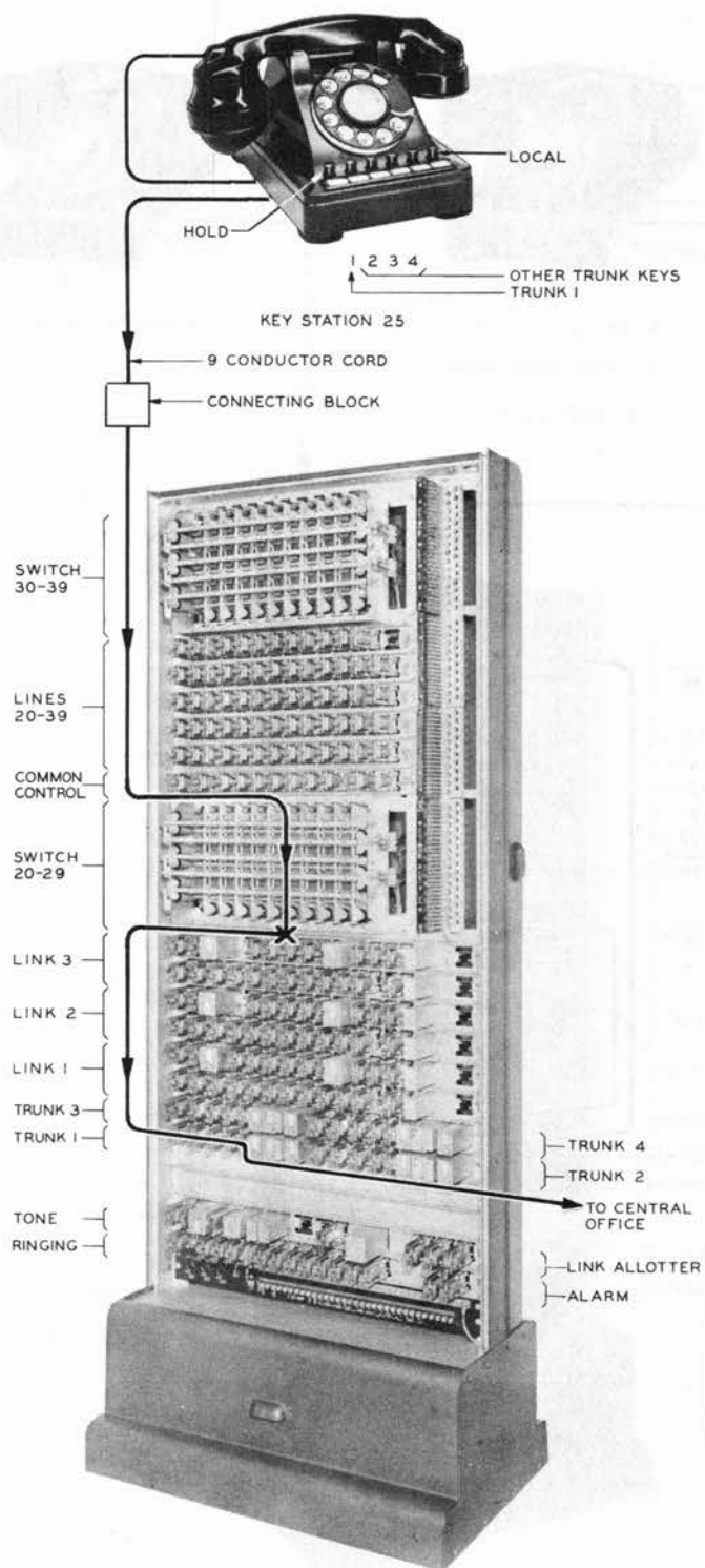
Fig. 6 - Key Station Calling Central Office
