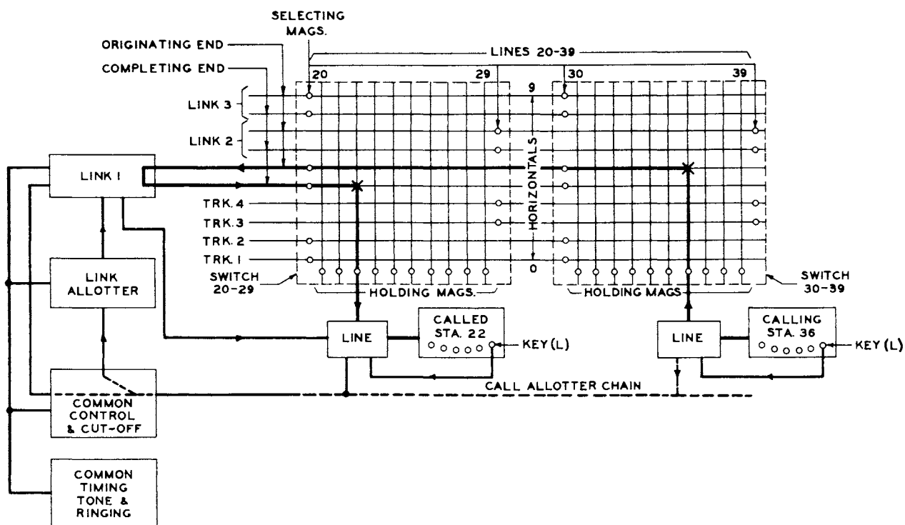
Fig. 8 - Block Diagram of Local Call
