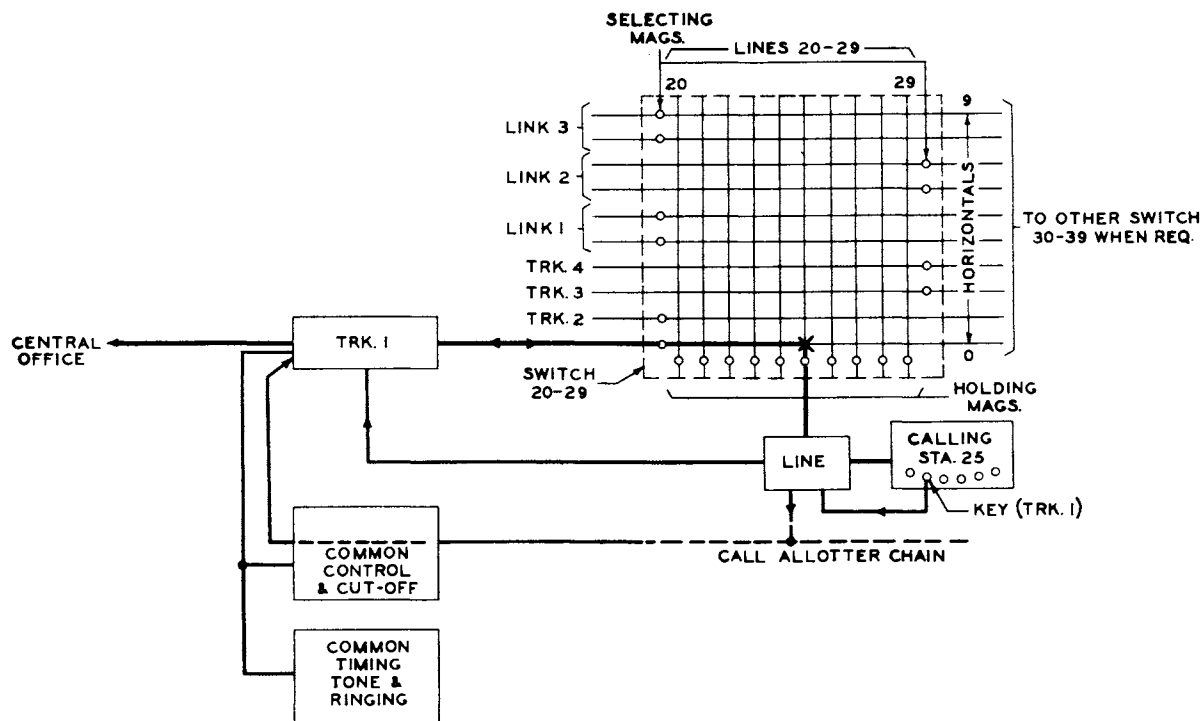
Fig. 9 - Block Diagram of Central Office Call
