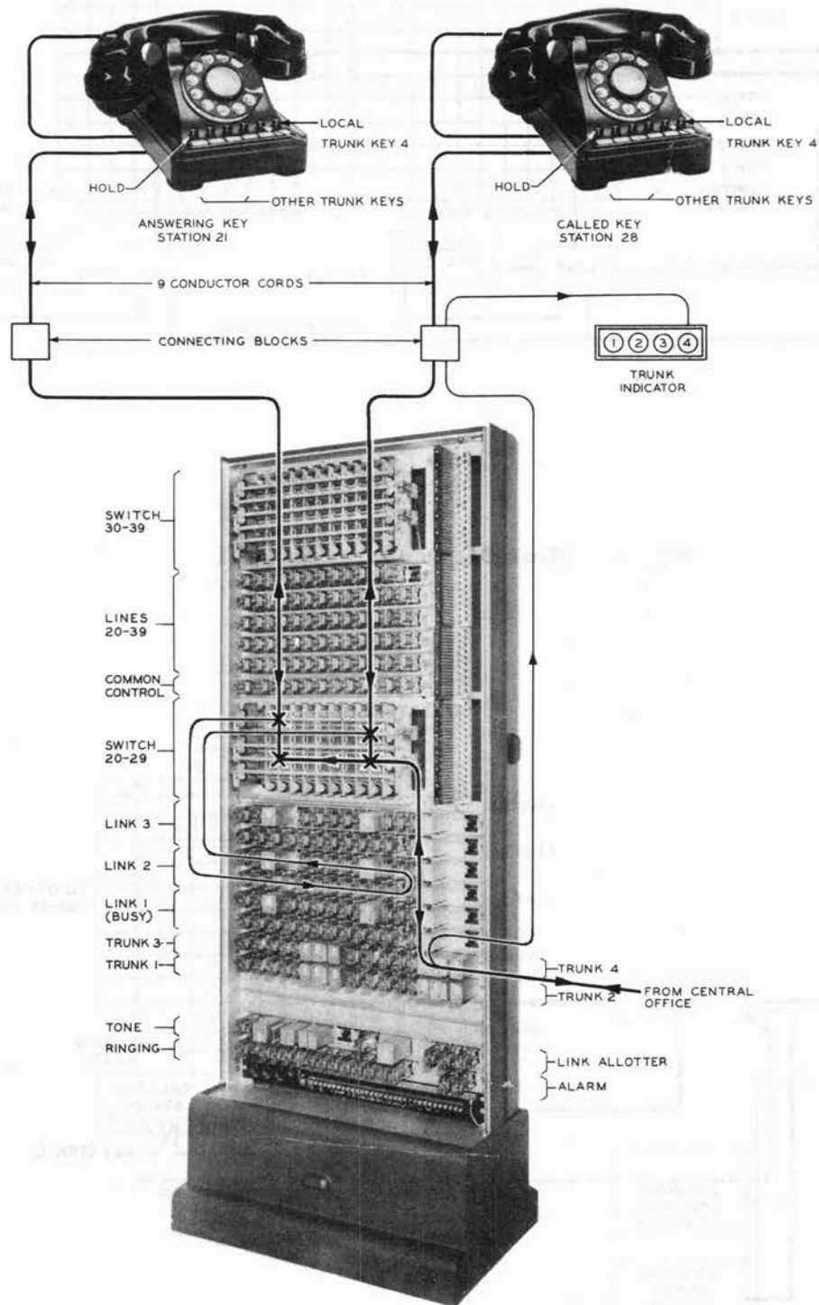
Fig. 7 - Central Office Calling Key Station
