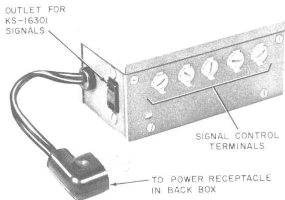
Fig. 6—Control Relay, KS-16301, List 15
