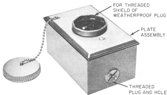
Fig. 2—Weatherproof Power Outlet KS-16301, List 18
