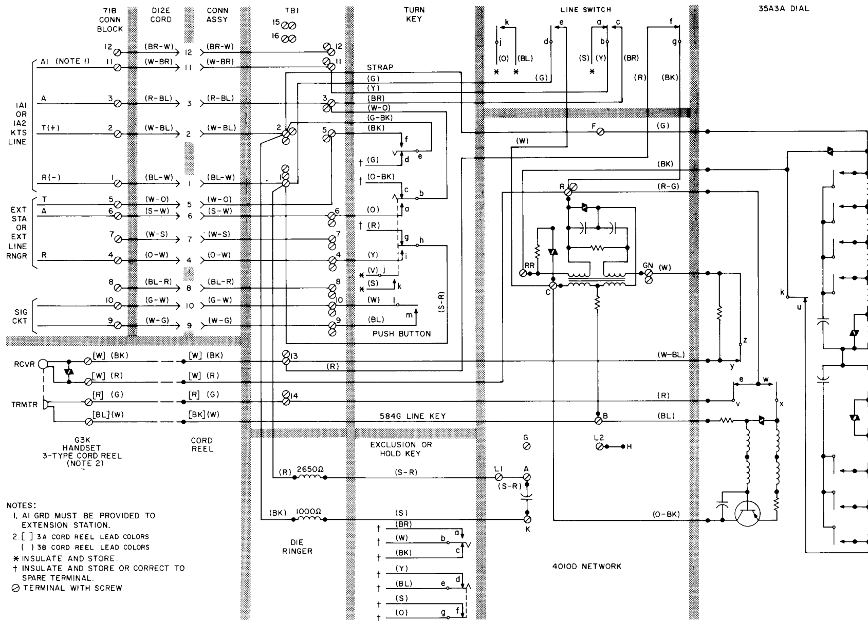
Fig. 7—2751-Type Telephone Set Connections, Wired For 1-Line Pickup, Signaling and Cutoff Feature
