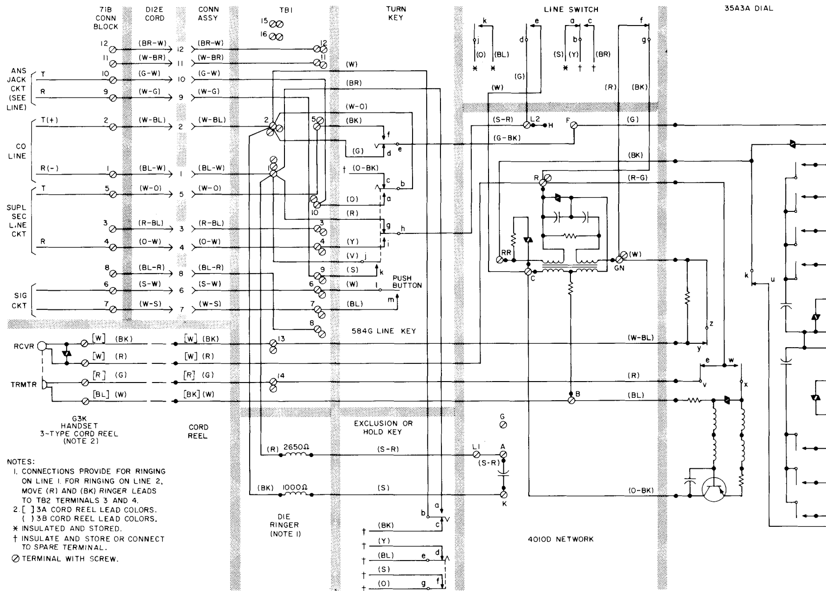
Fig. 6—2751-Type Telephone Set Connections, Wired For Secretarial Service, Signaling, and Hold (Nonkey System)
