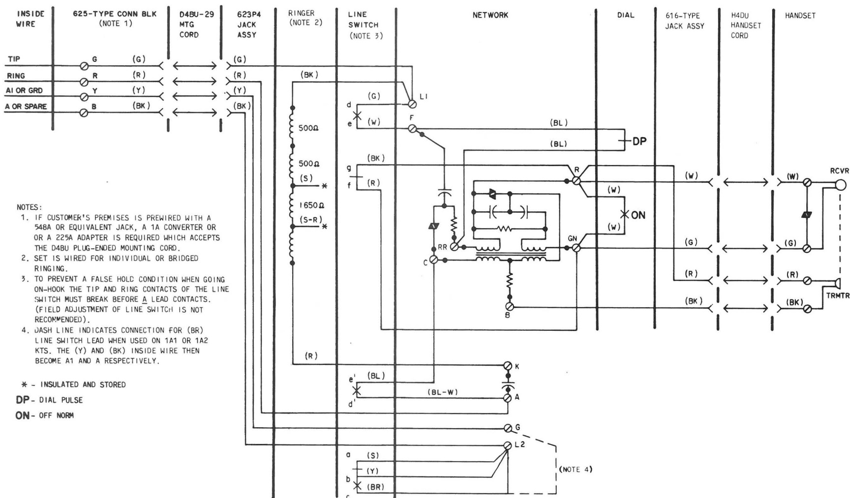
Fig. 4—CS881C102, CS881C103, or CS881C104 Telephone Set, Connections
