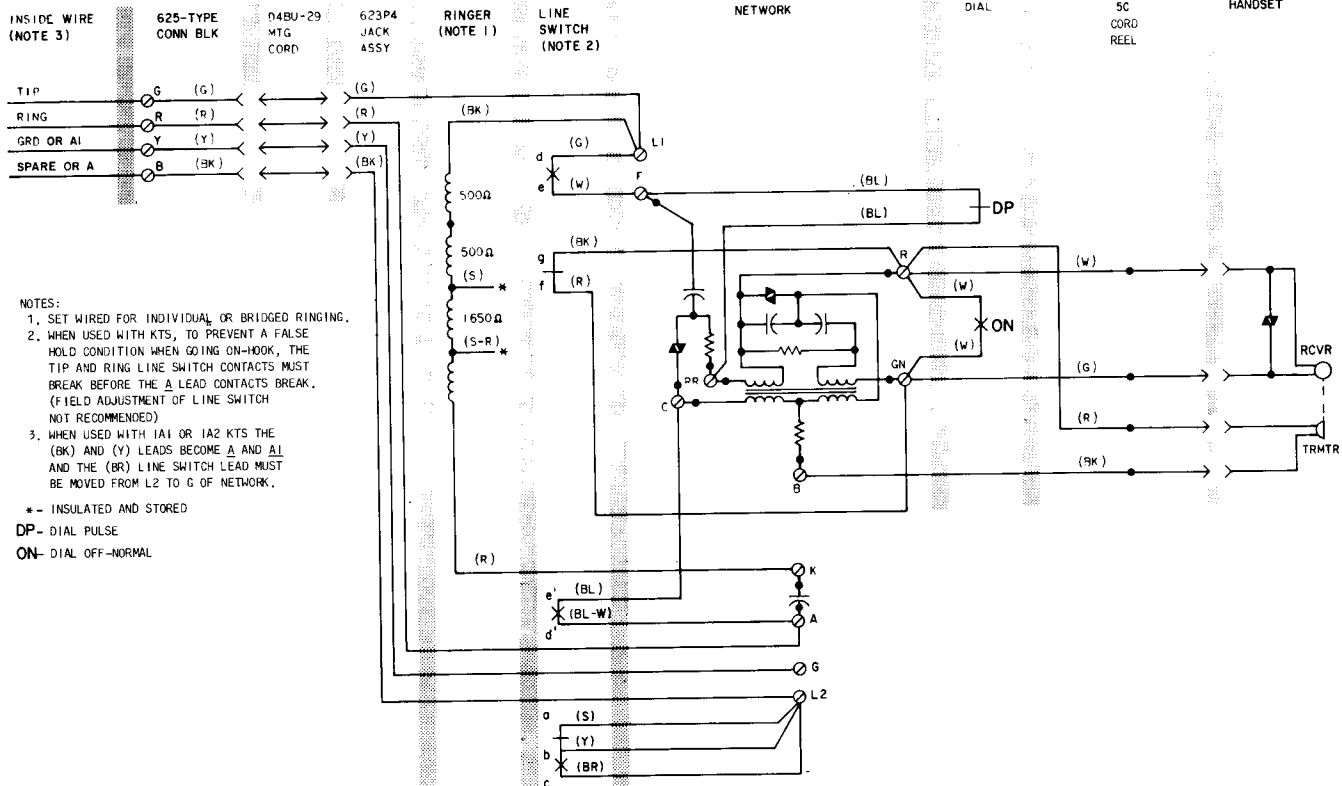
Fig. 2—911A1-03 Telephone Set, Connections
