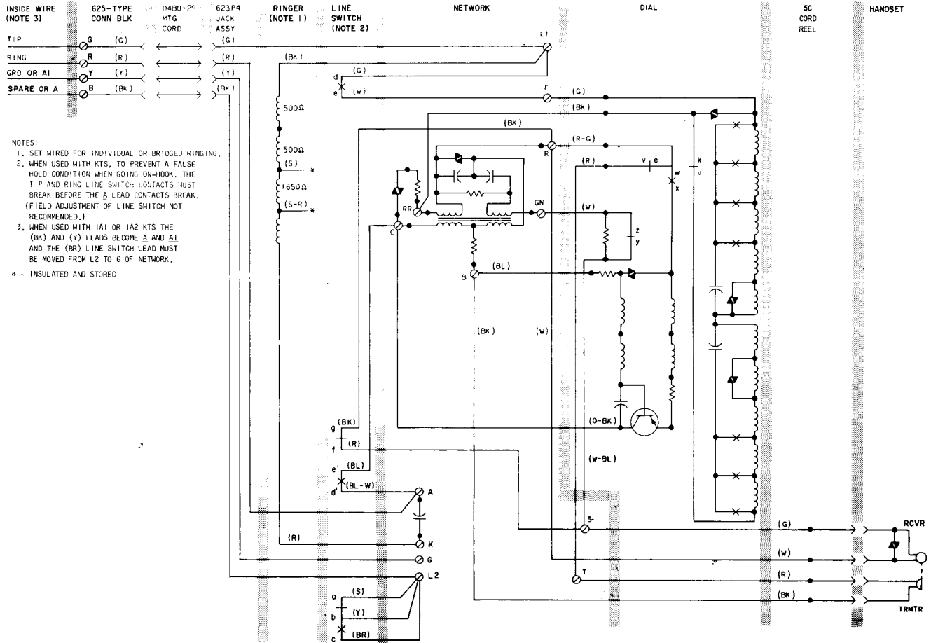
Fig. 3—2911A1-03 Telephone Set, Connections
