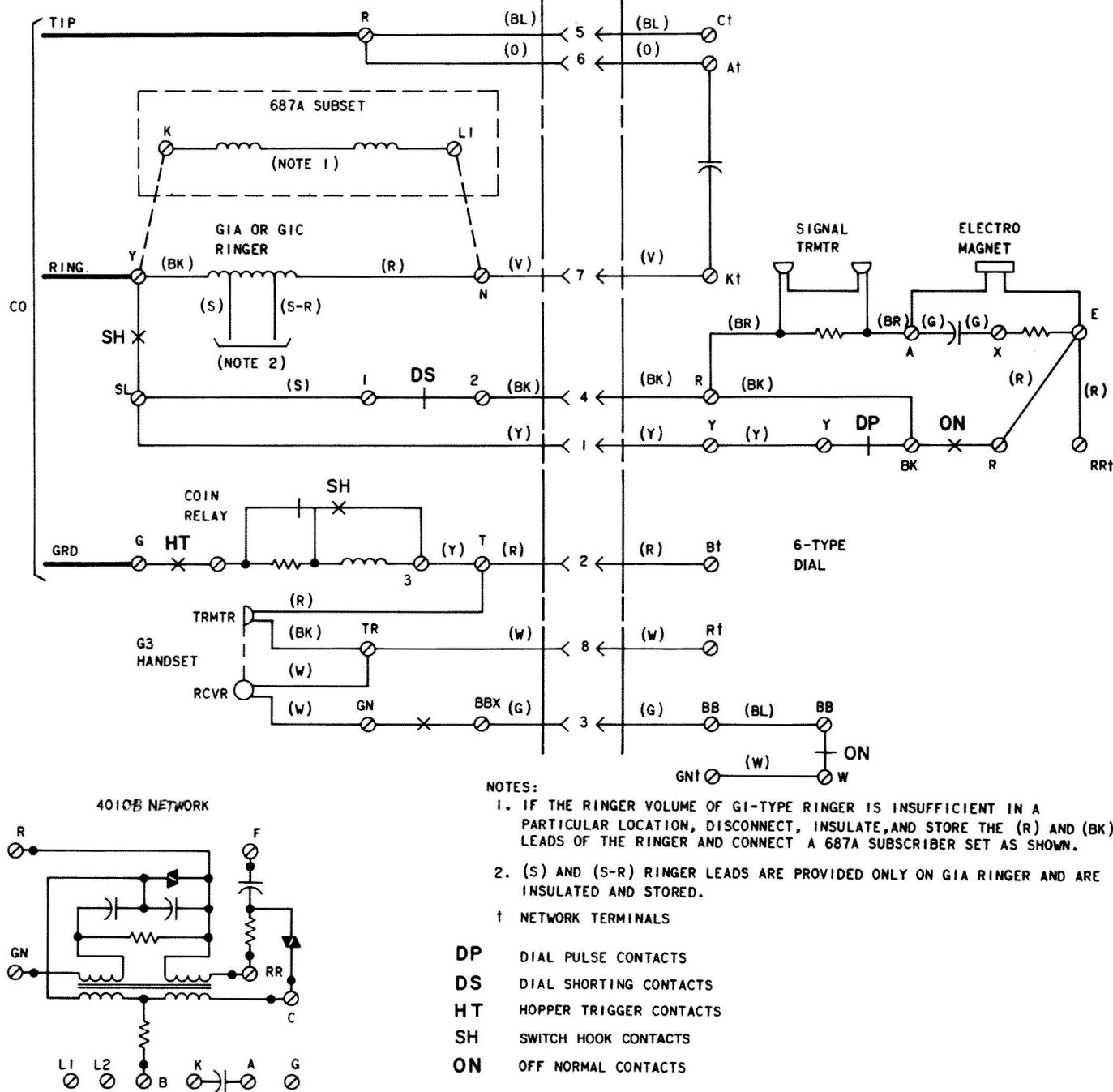
Fig. 1—236G Coin Collector, Connections
