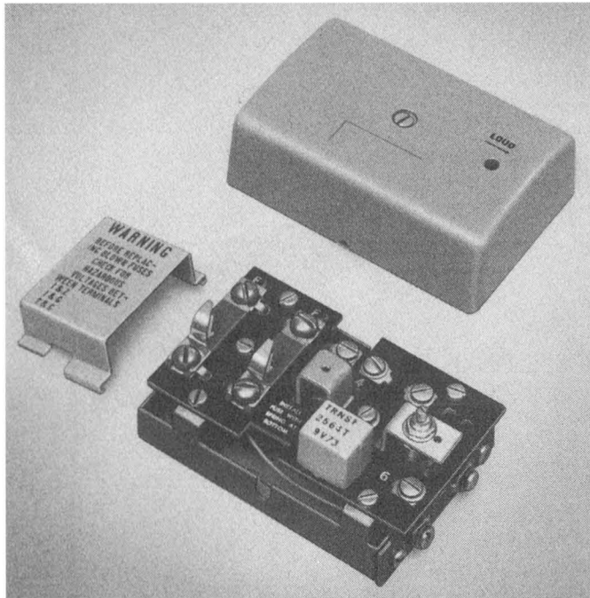
Fig. 12—33A Voice Coupler
