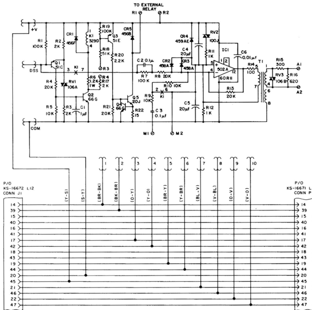
Fig. 32—Schematic, 27A Apparatus Unit
