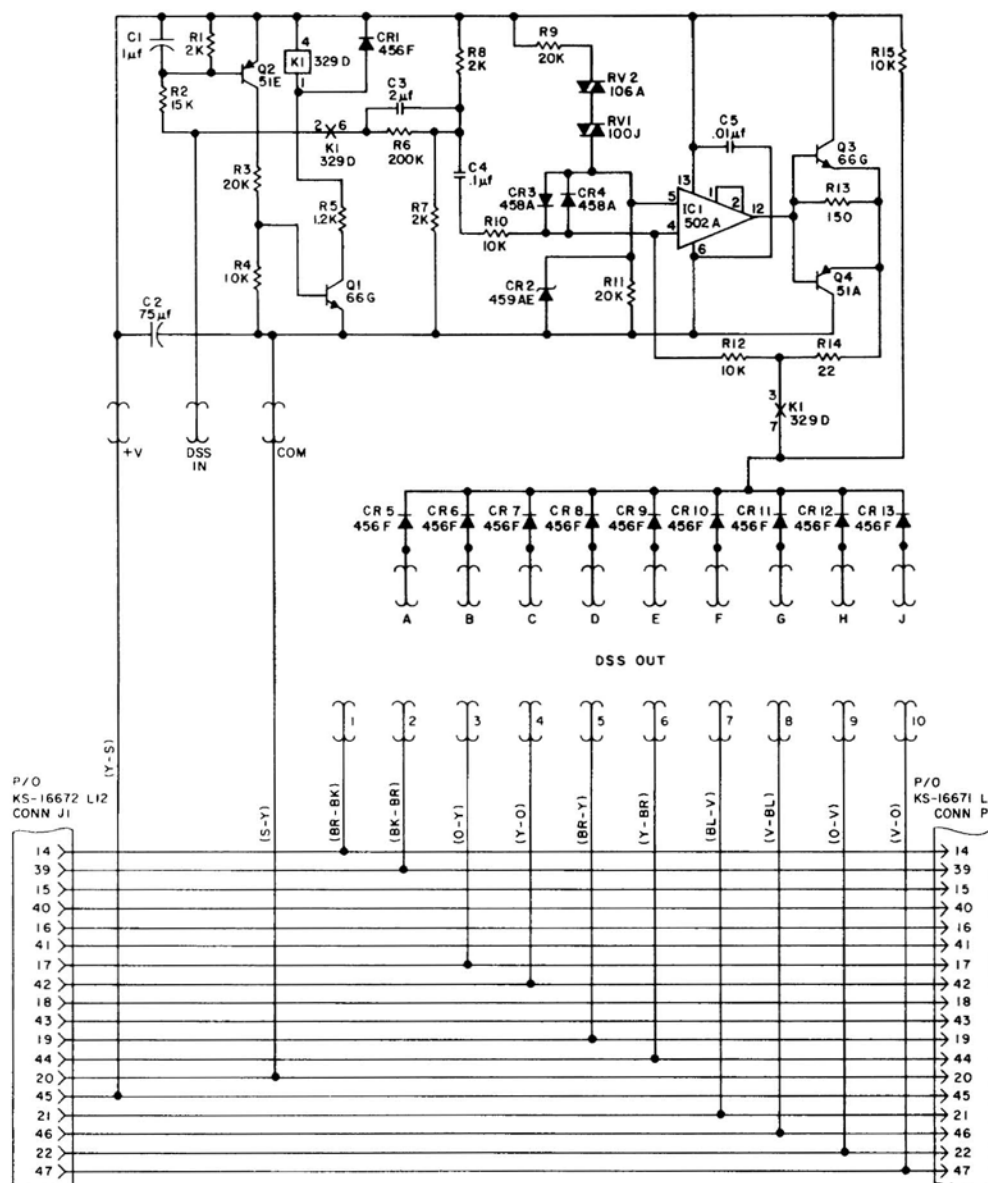
Fig. 31—Schematic, 26A Apparatus Unit
