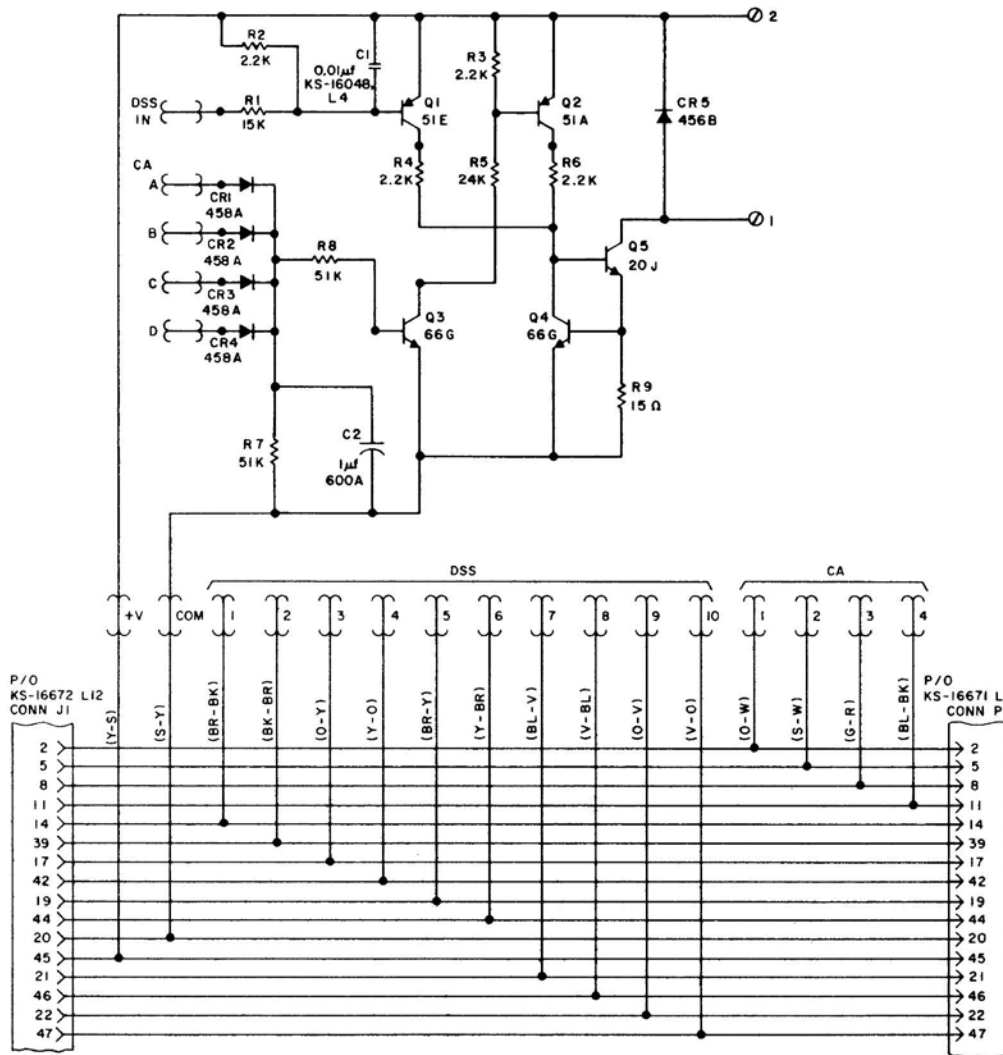
Fig. 30—Schematic, 25A Apparatus Unit
