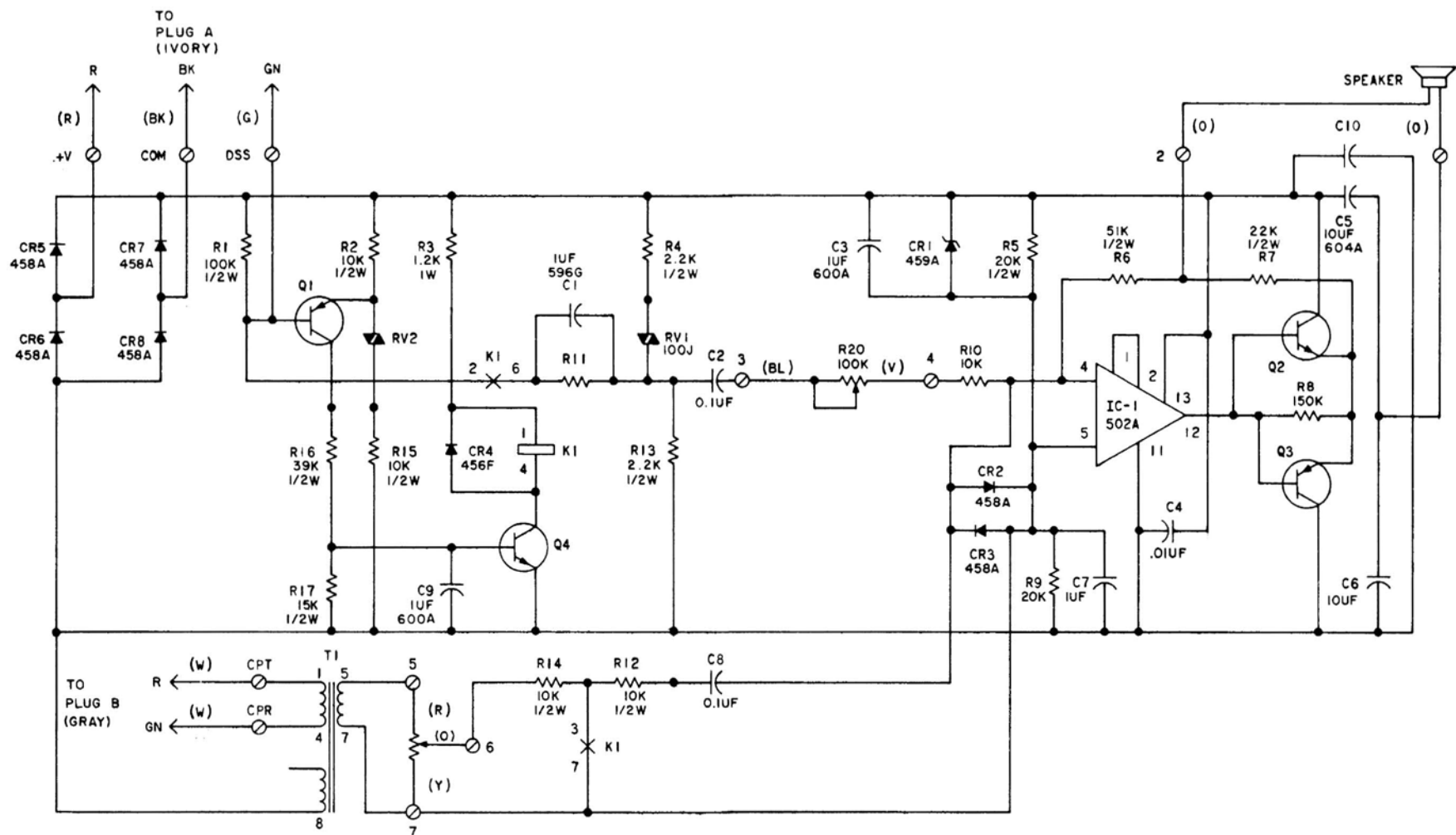
Fig. 33—Schematic, 109A Loudspeaker
