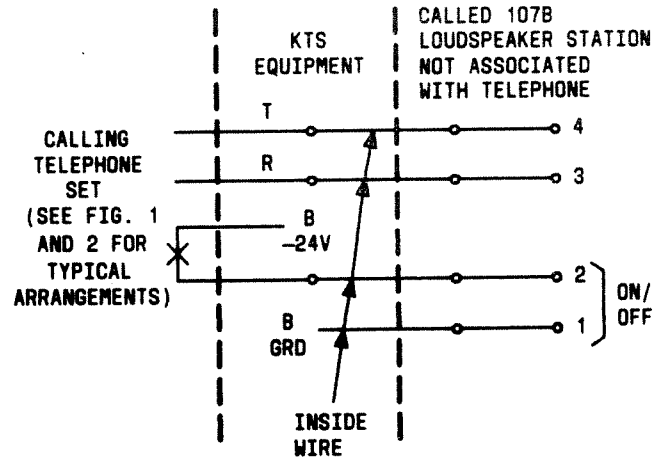
Fig. 3—Example of Standalone Voice-Signaling Arrangement
