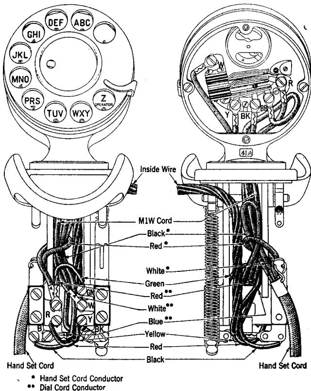
Fig. 7—211B, 211C, 211D Type Hand Telephone Sets.
