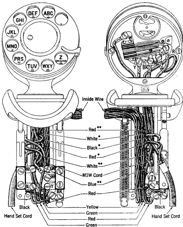
Fig. 10—213A, 213B 213C Type Hand Telephone Sets.
