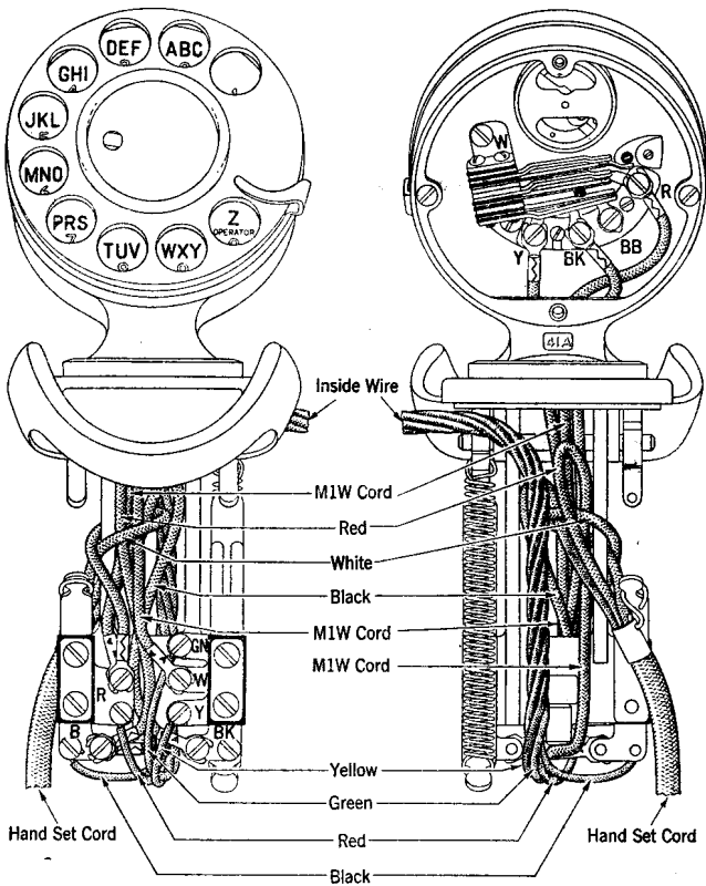
Fig. 8—211F, 211G, 211H Type Hand Telephone Sets.
