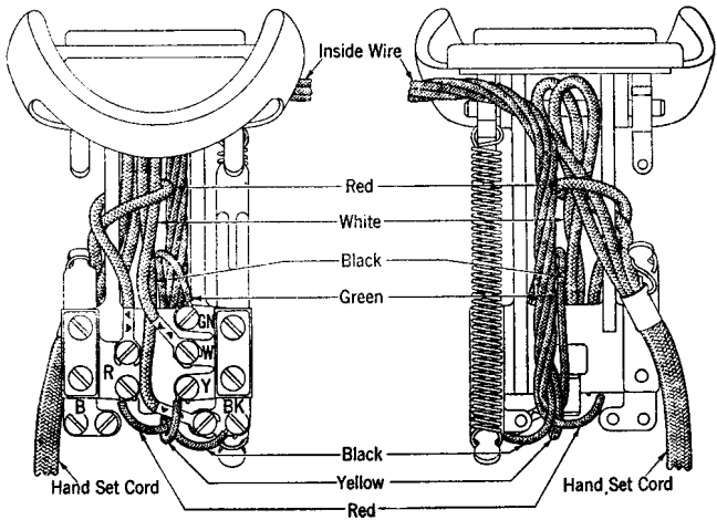
Fig. 2-211A Type Hand Telephone Sets.
