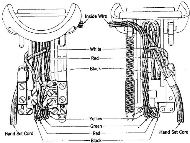
Fig. 3-211E Type Hand Telephone Sets.
