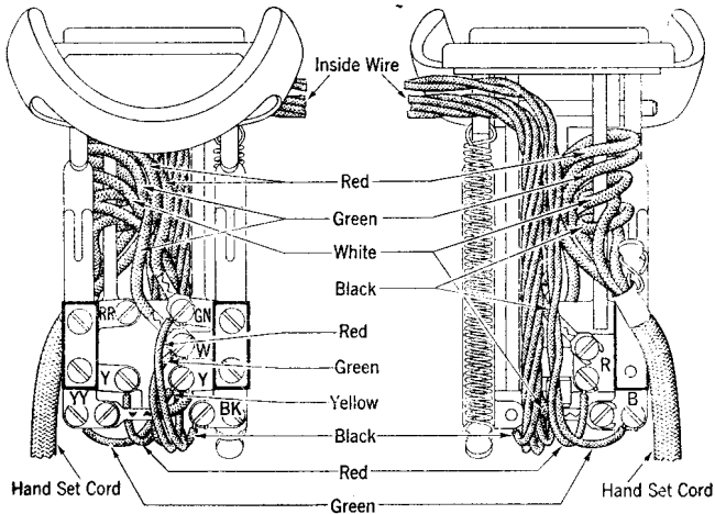
Fig. 5—214A Type Hand Telephone Sets.
