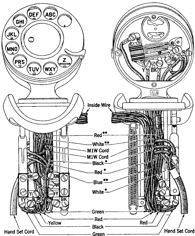
Fig. 9—212A, 212B, 212C Type Hand Telephone Sets.
