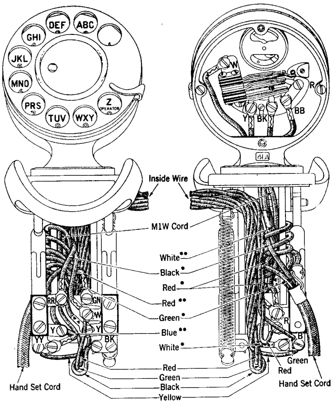
Fig. 11—214B, 214C, 214D Type Hand Telephone Sets.
