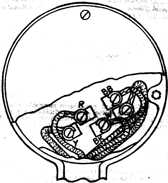
Fig. 13—Dial Cording—6-Type Dials
