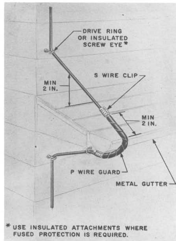
Metal Gutter
