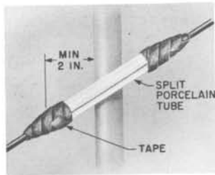
Fig. 1 — Crossing Exposed Steam Pipes
