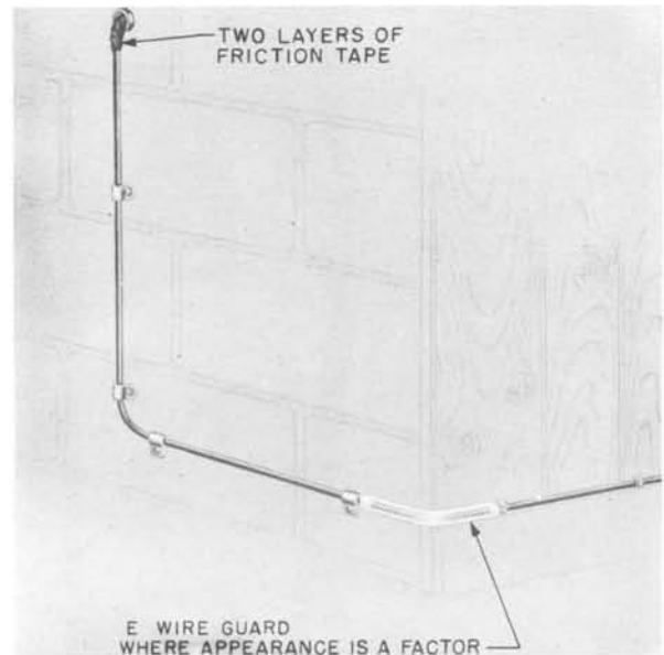
Fig. 4 — Use of Tape or E Wire Guard
