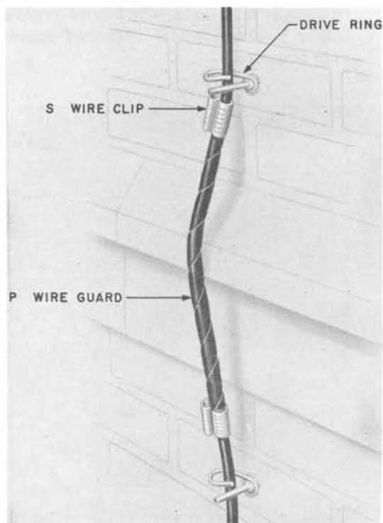
Fig. 5 — Crossing Masonry Building Projection
