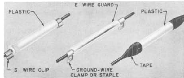
Fig. 3 — Securing Plastic Tubes or E Wire Guard
