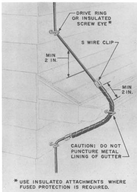
Metal-lined Wooden Box Gutter
