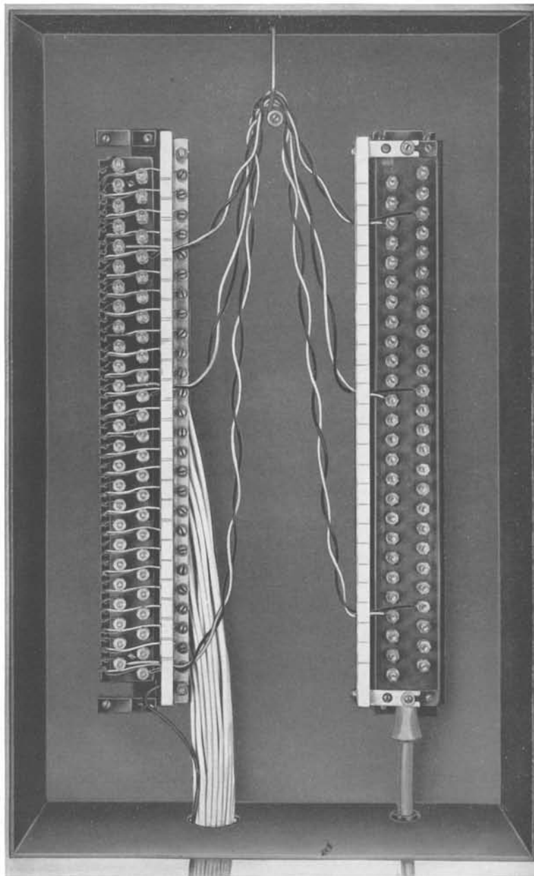
FIG. 10—TYPICAL WIRING OF CUSTOMER-PROVIDED CABINET
