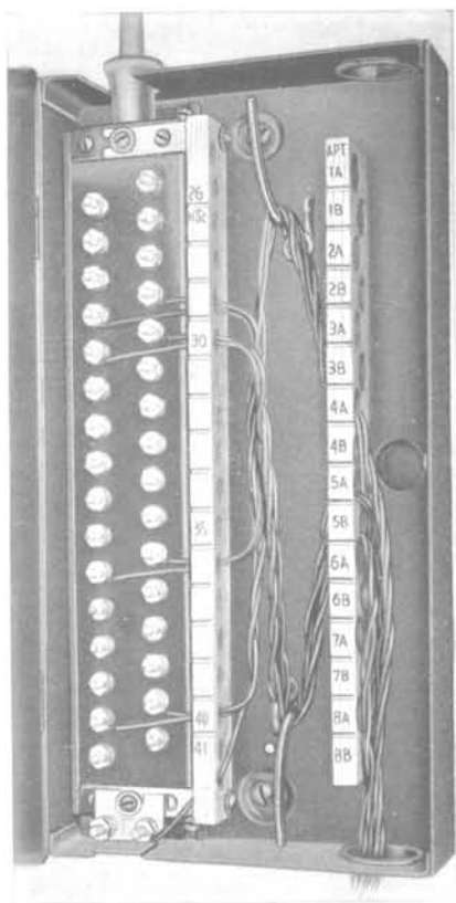
FIG. 2—STATION WIRING OF GB-TYPE TERMINAL
