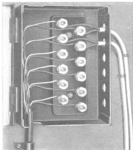
FIG. 3—STATION WIRING OF HS-TYPE TERMINAL
