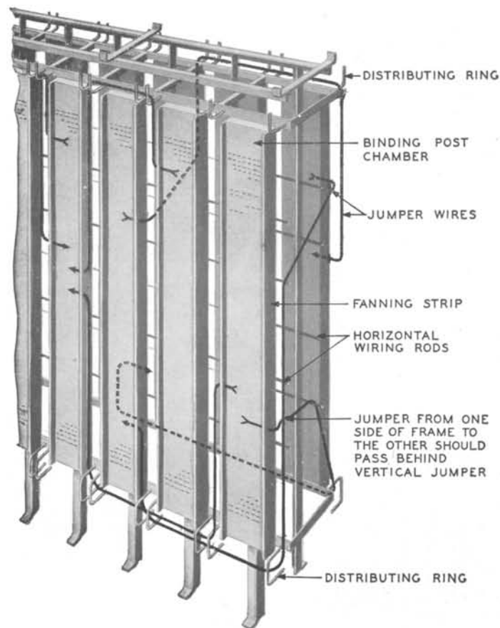
FIG. 5—CROSS-CONNECTION ARRANGEMENT ON A FRAME-TYPE TERMINAL
