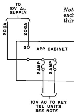
Fig. 1 — Fusing for More Than 36 Lamps
