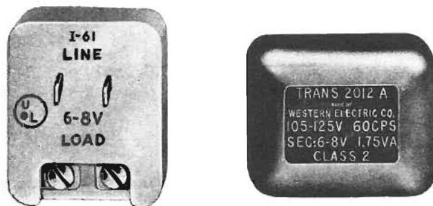
Fig. 2 – 2012A Transformer
