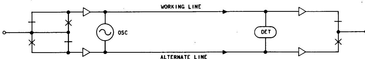
Fig. 3—Line Automatic Sensing and Switching (LASS)—Simplified Application Schematic
