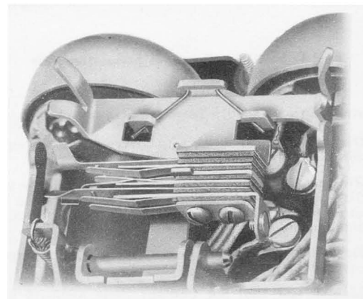
Fig. 2—Exclusion Switch (P-19A410 Switch Assembly)
