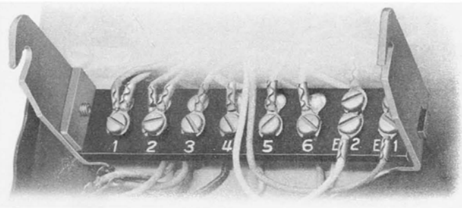
Fig. 4—P-338886 Terminal Strip Assembly
