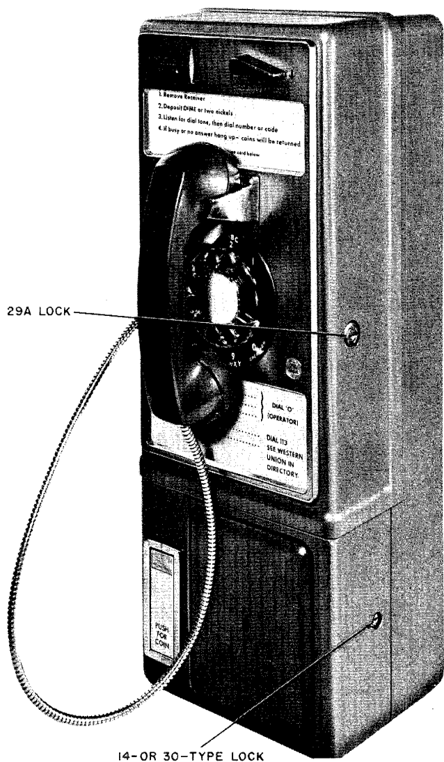
Fig. 4 — Location of Locks
