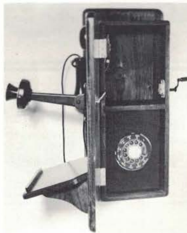
COLONIAL WALL TELEPHONES Side view - Door Open. Dial and interior shown.
