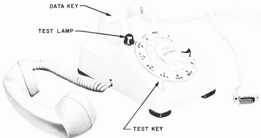
Fig. 1 — 513-Type Telephone Set
