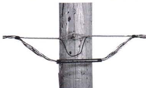
Galvanized Steel Dead-Ends for Galvanized Steel Wire or Messenger
