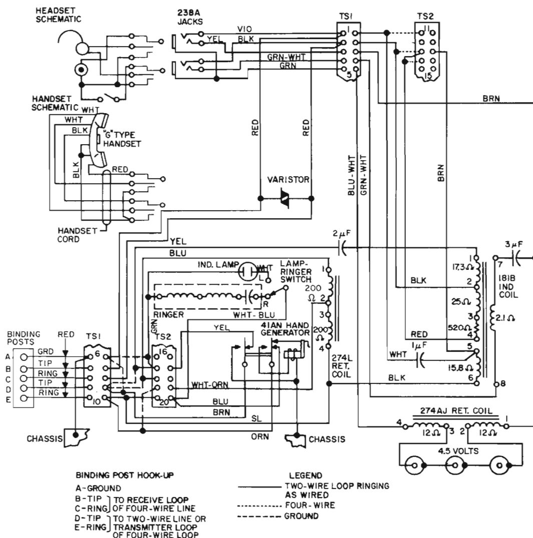
Figure 3. Schematic Diagram of the GB50683-A Portable 2 or 4-Wire Magneto Telephone Set.
