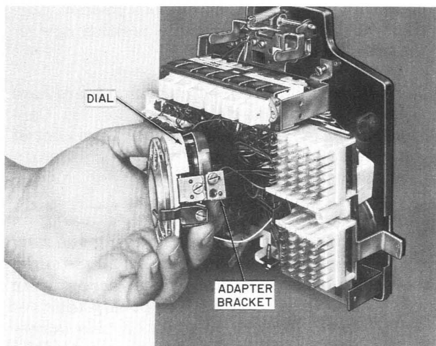
Fig. 17—Dial Adapter Bracket
