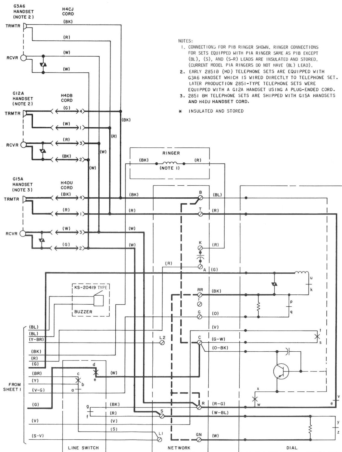
Fig. 32— 2851BT (MD), 2851B (MD), and 2851BM (MD) Telephone Sets, Connections (Sheet 2 of 2)
