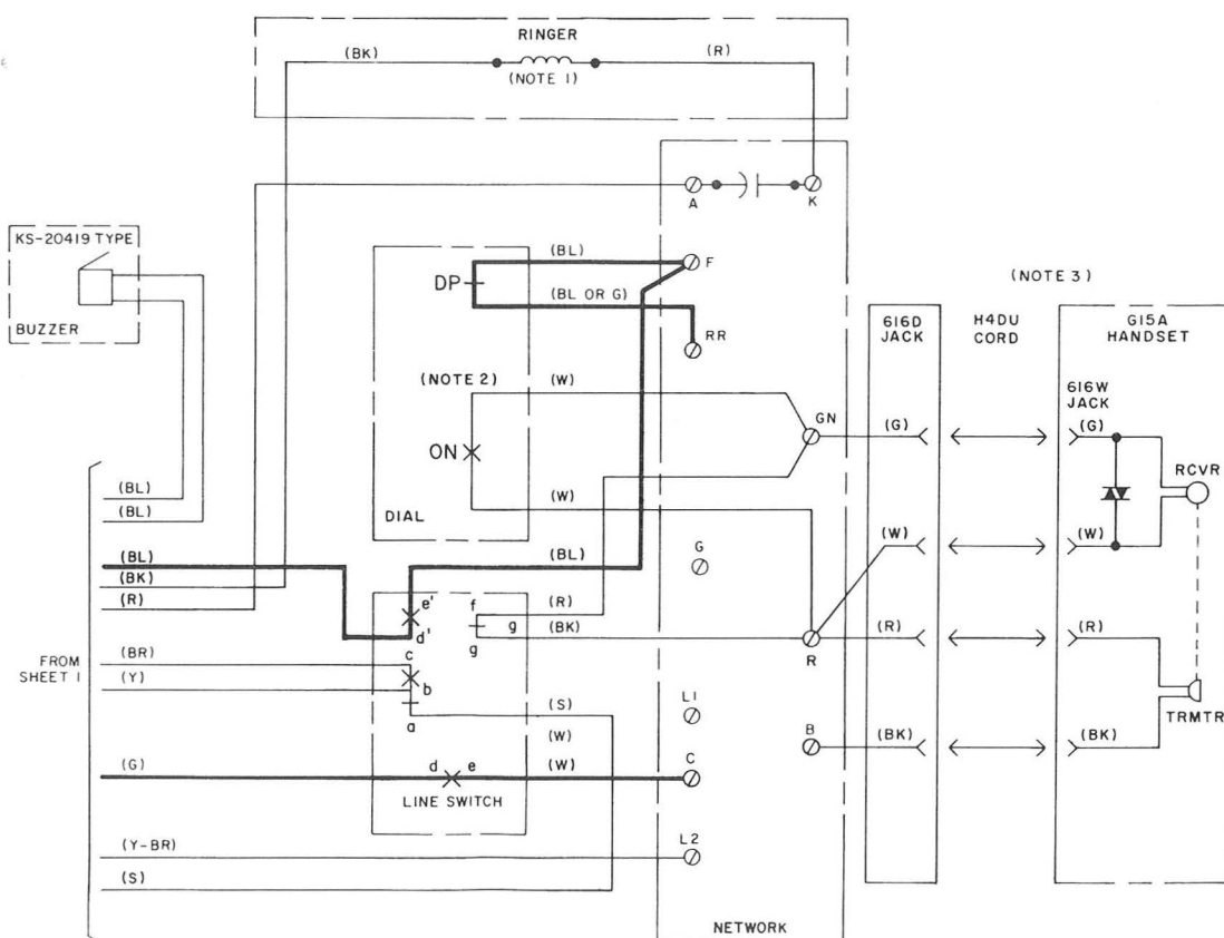
Fig. 33—851CM Telephone Set, Connections (Sheet 2 of 2)
