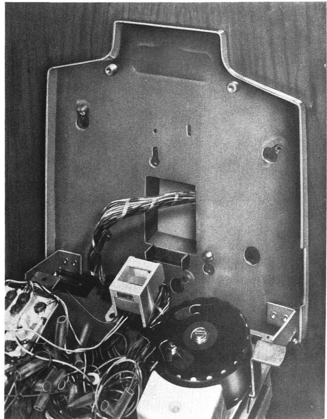
Fig. 9—Inside Wiring Cable, from Outlet Box (Early Version)
