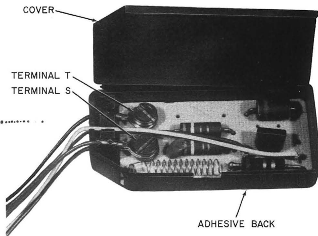
Fig. 15—840364376 Polarity Guard
