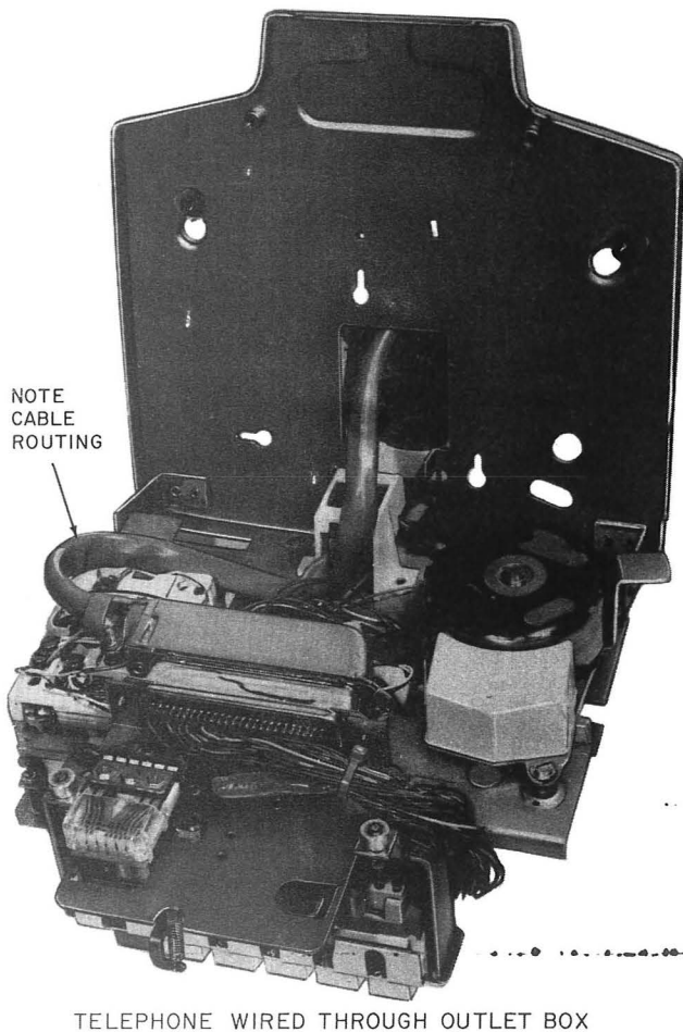
Fig. 12—Cable Routing in Current 851CM and 2851CM Telephone Sets at Prewired Location
