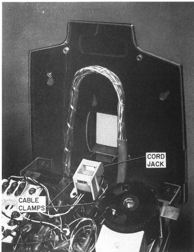
Fig. 8—Inside Wiring Cable, Exposed Wiring (Original Version)
