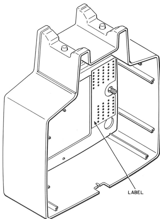
Fig. 21 — Connecting Block Terminal Information
