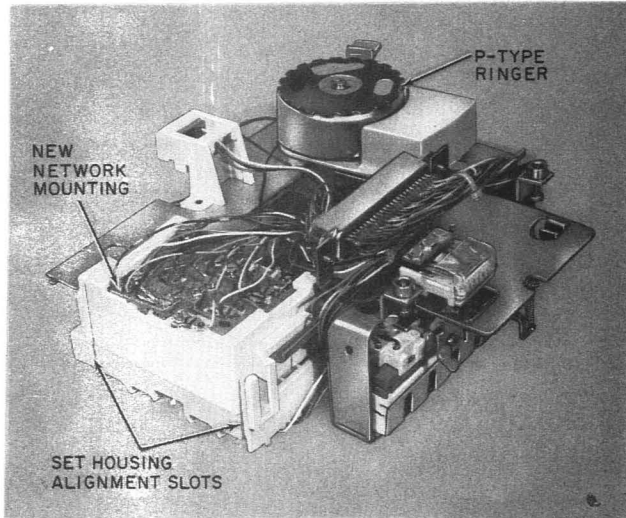
Fig. 7—Rear of 2851-Type Telephone Set Hinged Chassis Assembly With New Network Mounting
