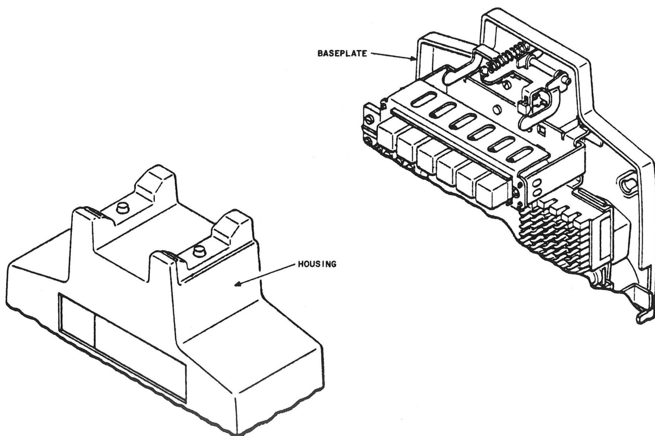
Fig. 22—Original Version Baseplate and Housing
