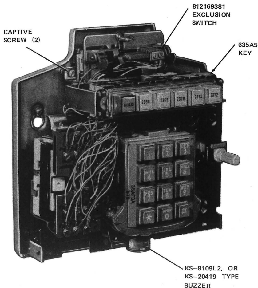
Fig. 5—2851CM Telephone Set With Exclusion (Housing Removed)
