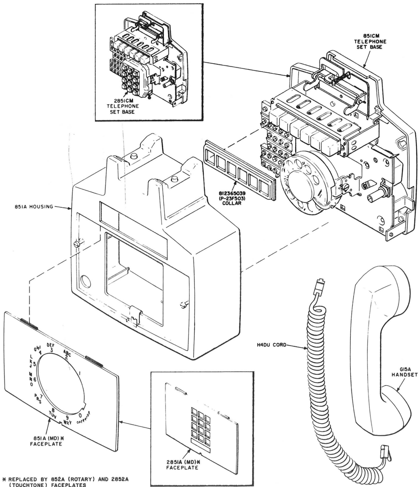
Fig. 25— Station Modular Arrangement 851CM and 2851CM Current Telephone Sets
