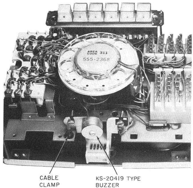
Fig. 18—KS-20419 Type Buzzer Mounted on 851-Type Telephone Set
