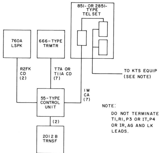
Fig. 26—Block Diagram of 3-Type (MD) Speakerphone Control Unit Located Near Station
