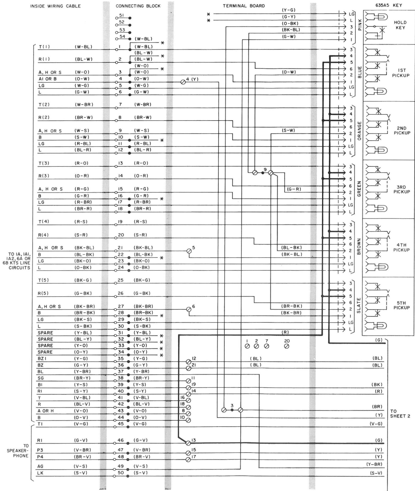
Fig. 31—851BT (MD), 851B (MD), and 851BM (MD) Telephone Sets, Connections (Sheet 1 of 2)
