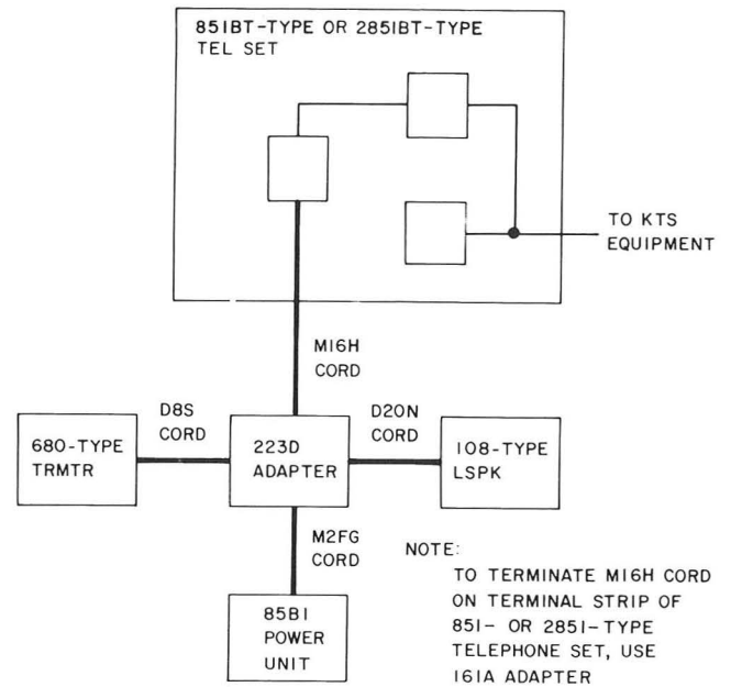
Fig. 28—Block Diagram of 4A Speakerphone Located at Station Using 223D Adapter
