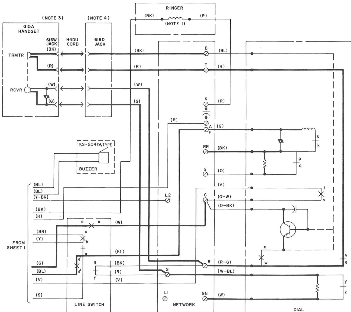
Fig. 34—2851CM Telephone Set, Connections (Sheet 2 of 2)
