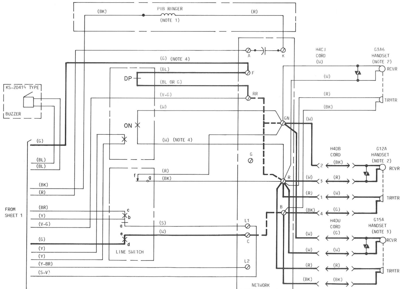
Fig. 31—851BT (MD), 851B (MD), and 851BM (MD) Telephone Sets, Connections (Sheet 2 of 2)
