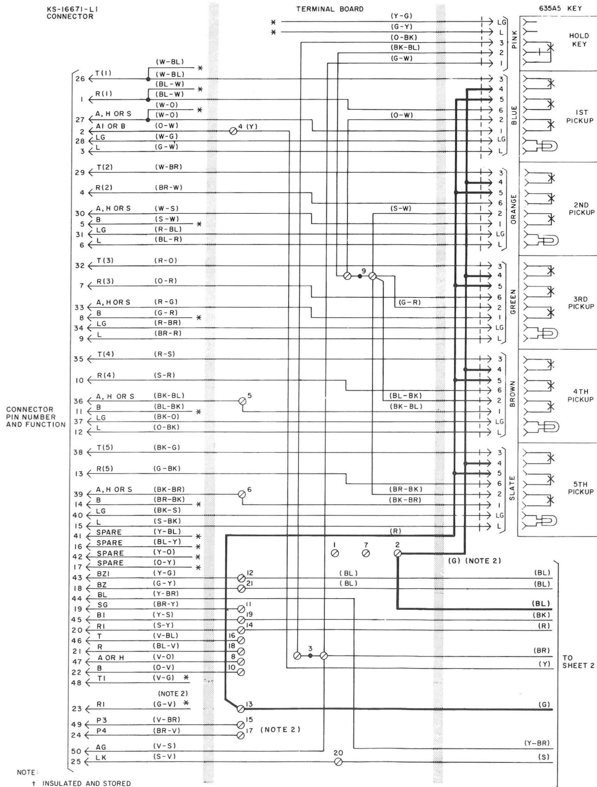
Fig. 33—851CM Telephone Set, Connections (Sheet 1 of 2)
