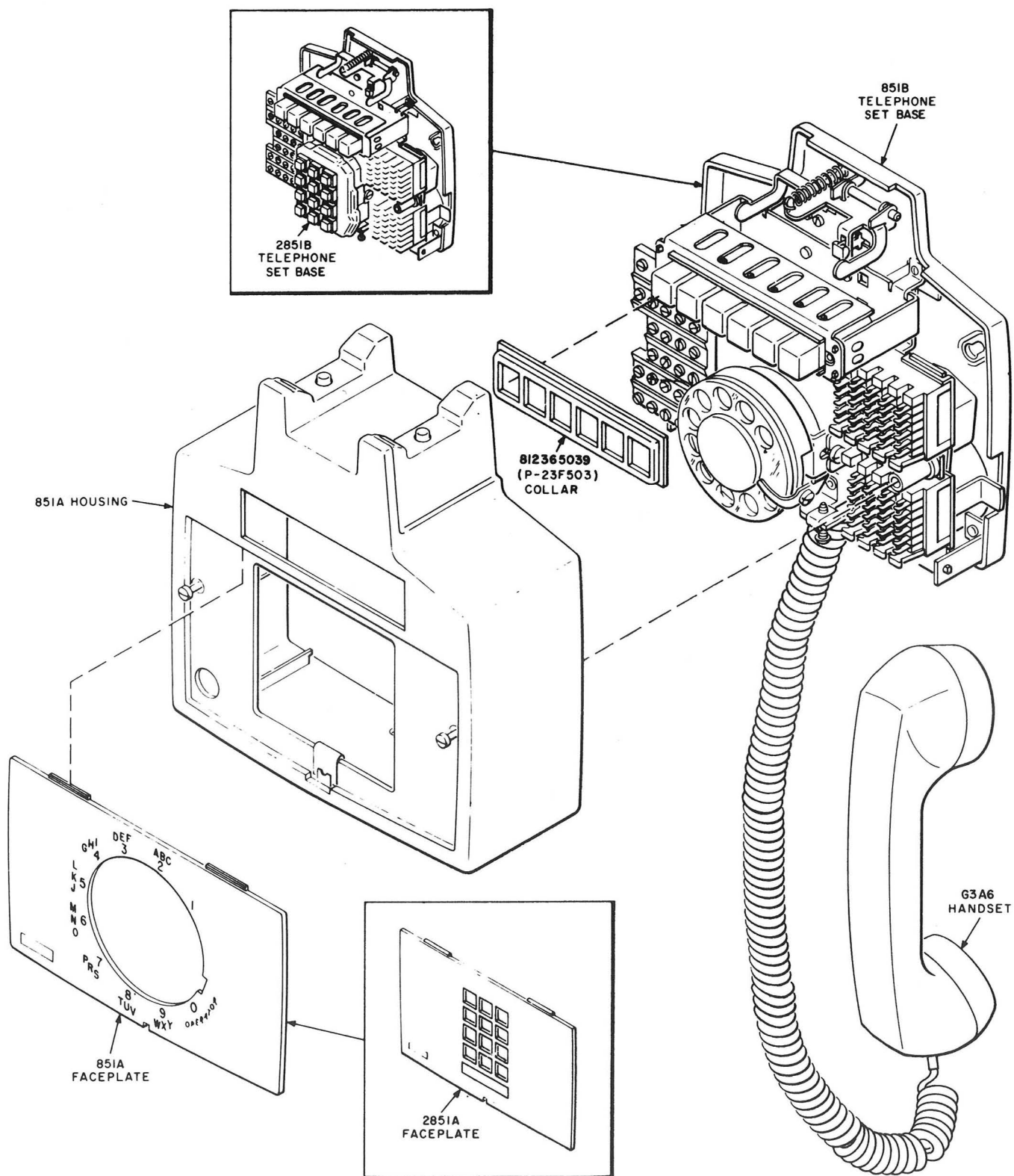
Fig. 23—851B (MD) and 2851B (MD) Telephone Sets, Early Version, Showing Baseplate and 851A Housing
