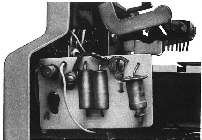
Fig. 14—819041971 (MD) Polarity Guard Position
