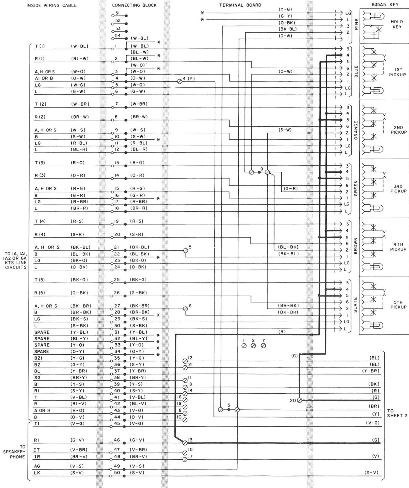
Fig. 32—2851BT (MD), 2851B (MD), and 2851BM (MD), Telephone Sets, Connections (Sheet 1 of 2)
