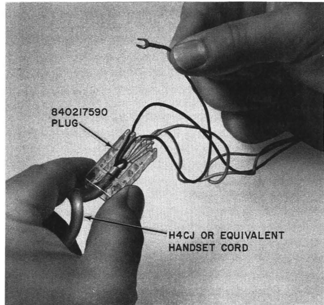
Fig. 19—Installing Spade-Tipped Handset Cords in Early Production 851- and 2851-Type Telephone Sets with G12A Handset
