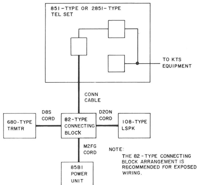
Fig. 27—Block Diagram of 4A Speakerphone Located at Station Using 82-Type Connecting Block
