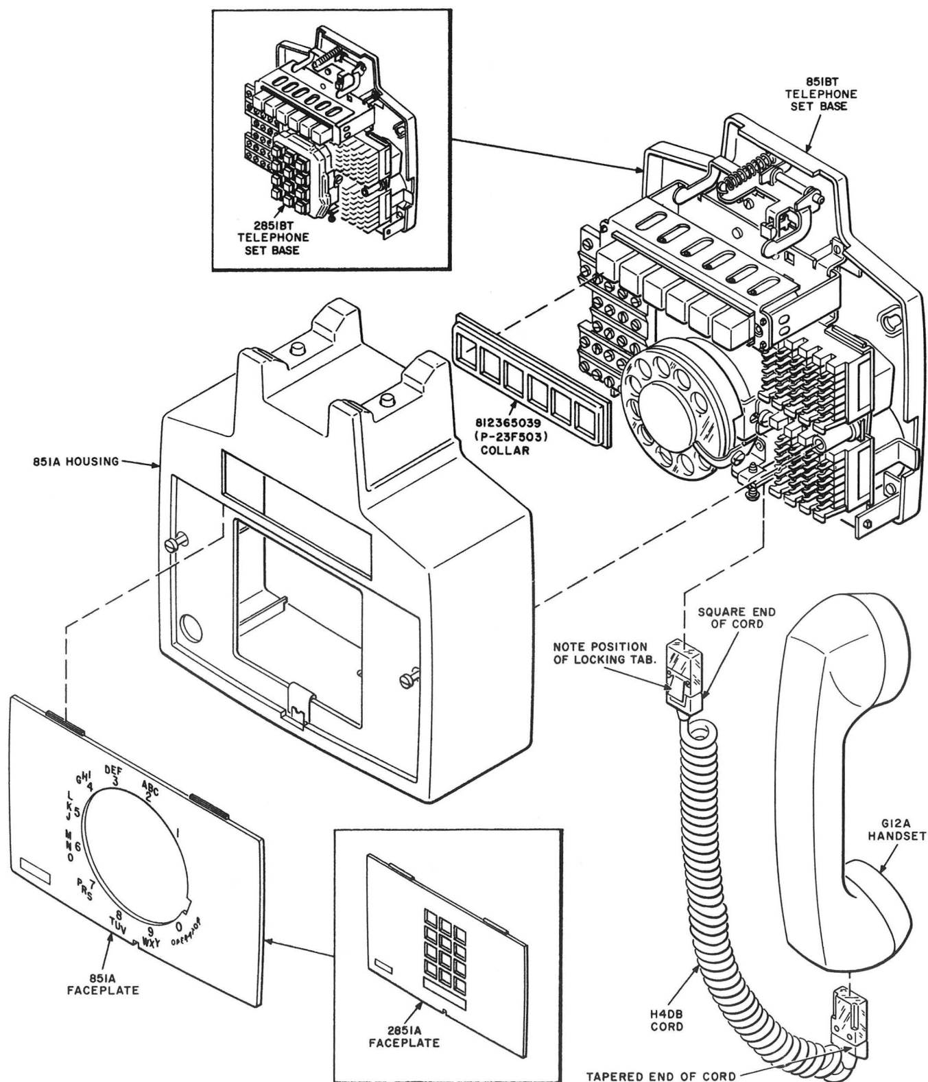
Fig. 24—Station Modular Arrangement, 851BT (MD) and 2851BT (MD) Telephone Sets Showing Later Baseplate and 851A Housing
