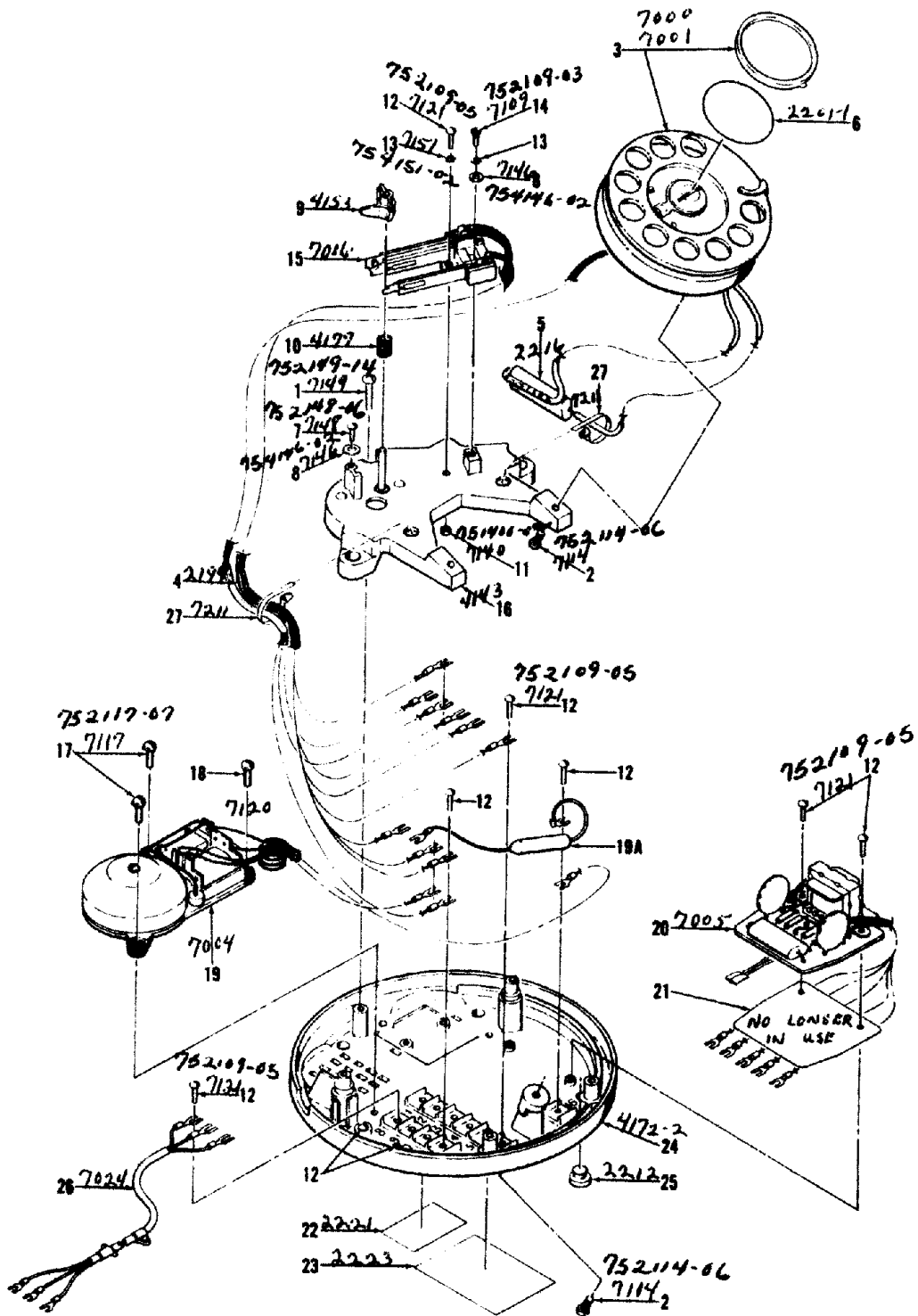
CANDLESTICK BASE ASSEMBLY, PART NO. 4125-1
