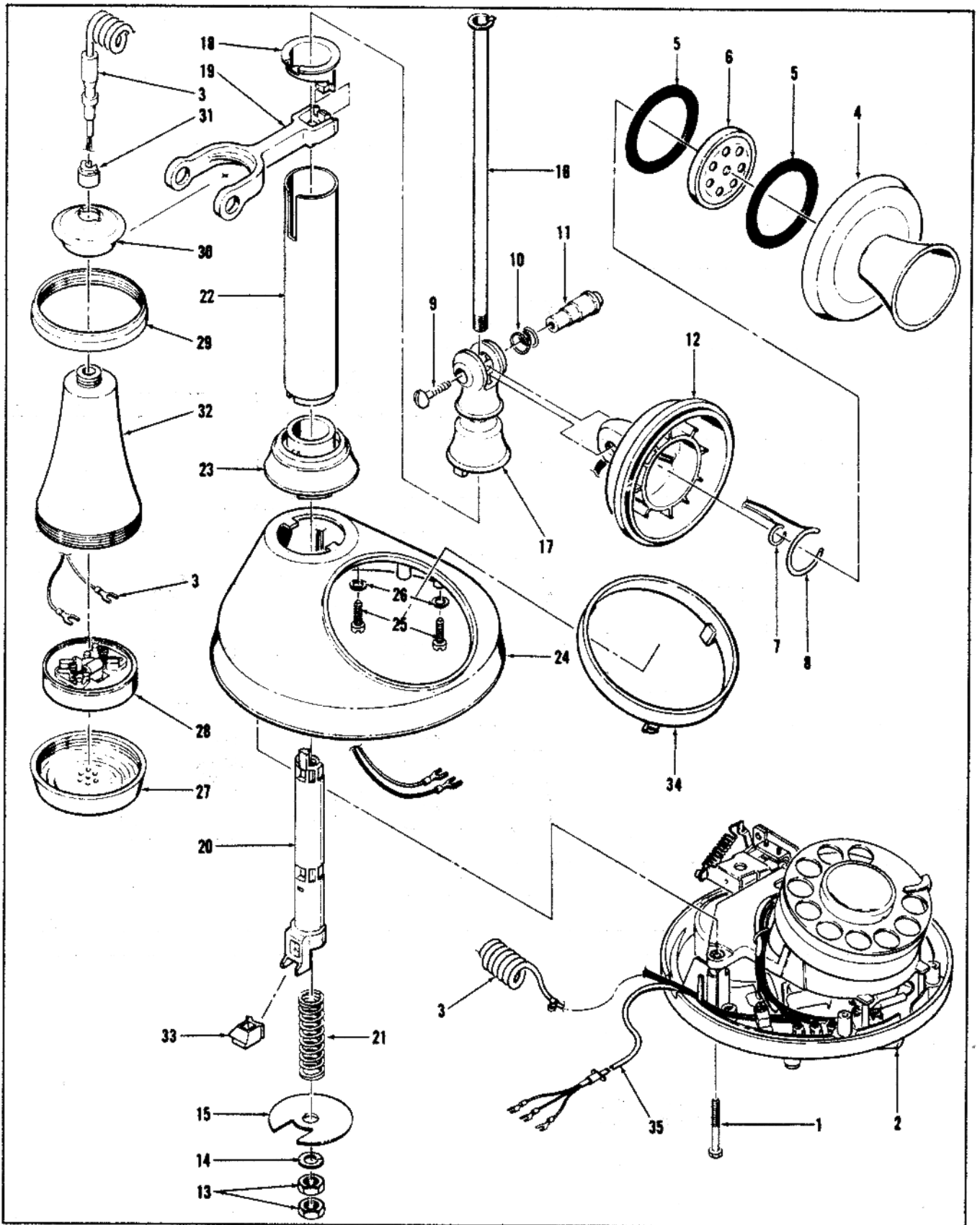
Candlestick Telephone Assembly
