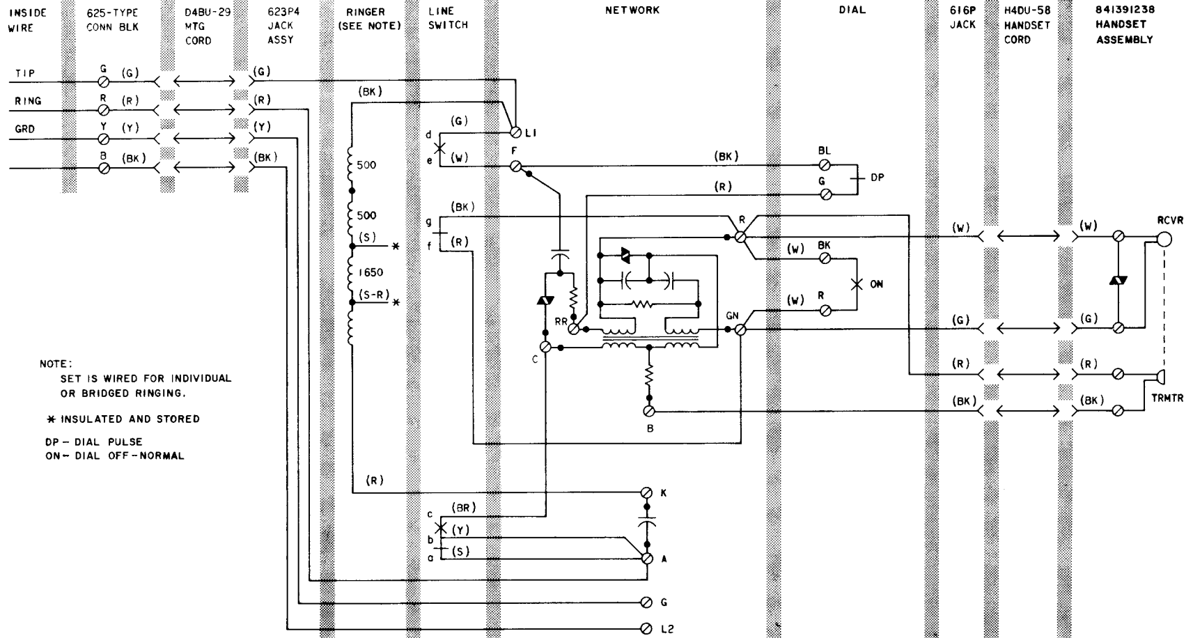
881B109 (MD) Telephone Set, Connections
