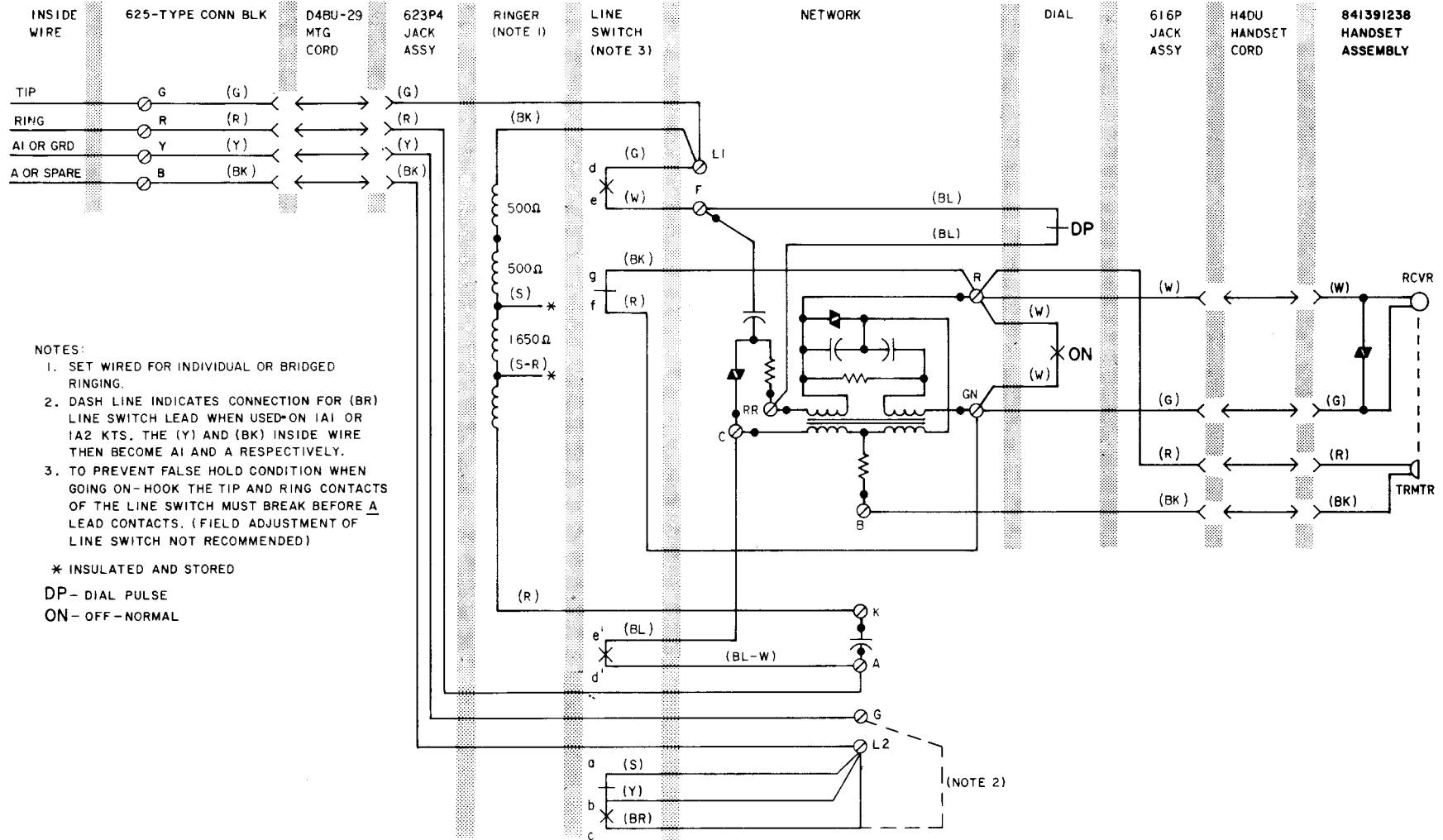
881C109 Telephone Set, Connections
