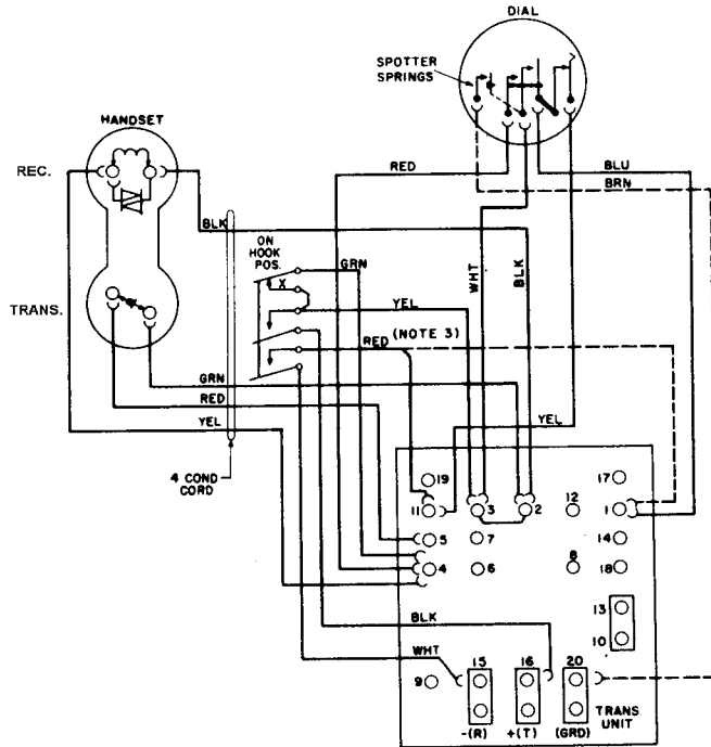
Schematic and Wiring Diagram for the Self-Compensating Type 183 Telephone.
