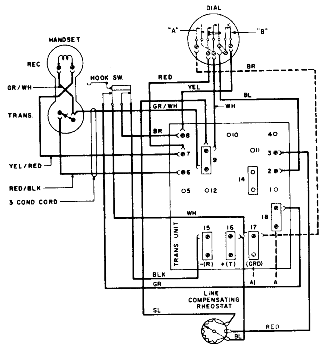
Schematic and Wiring Diagram for the Manually Adjusted Type 183 Telephone.
