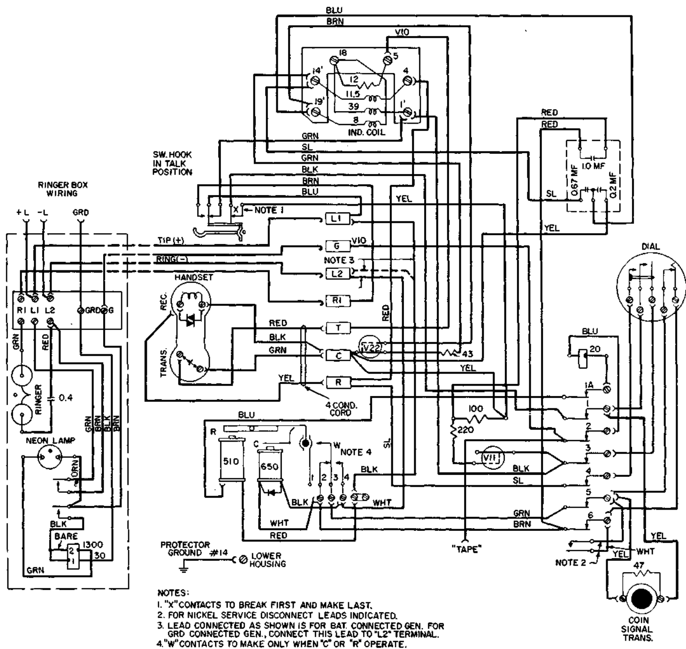
Figure 16. Type LPB 89-55 Local Prepay Paystation Wiring Diagram
