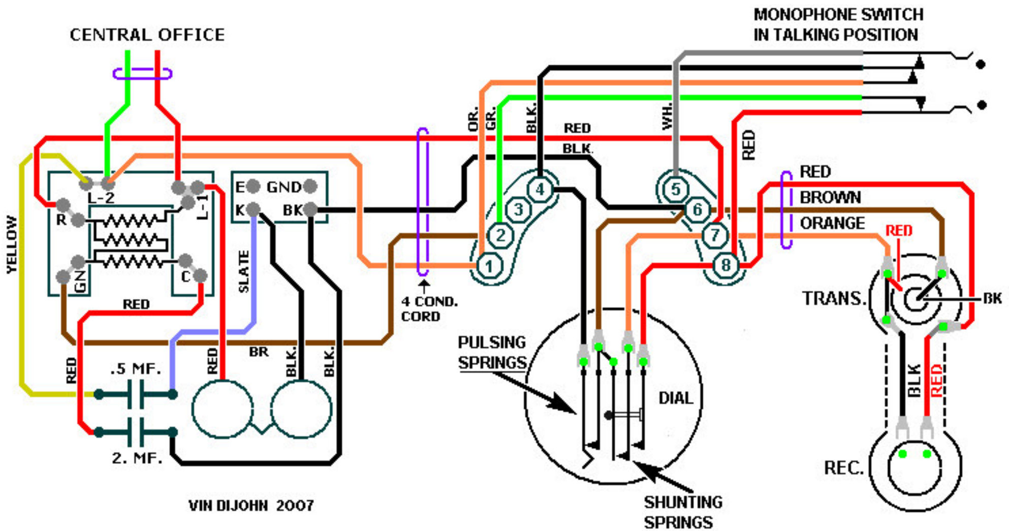
AUTOMATIC ELECTRIC A1 MONOPHONE WITH 5-LEAF SWITCH WIRED TO A WESTERN ELECTRIC 302 AS A SUBSET
