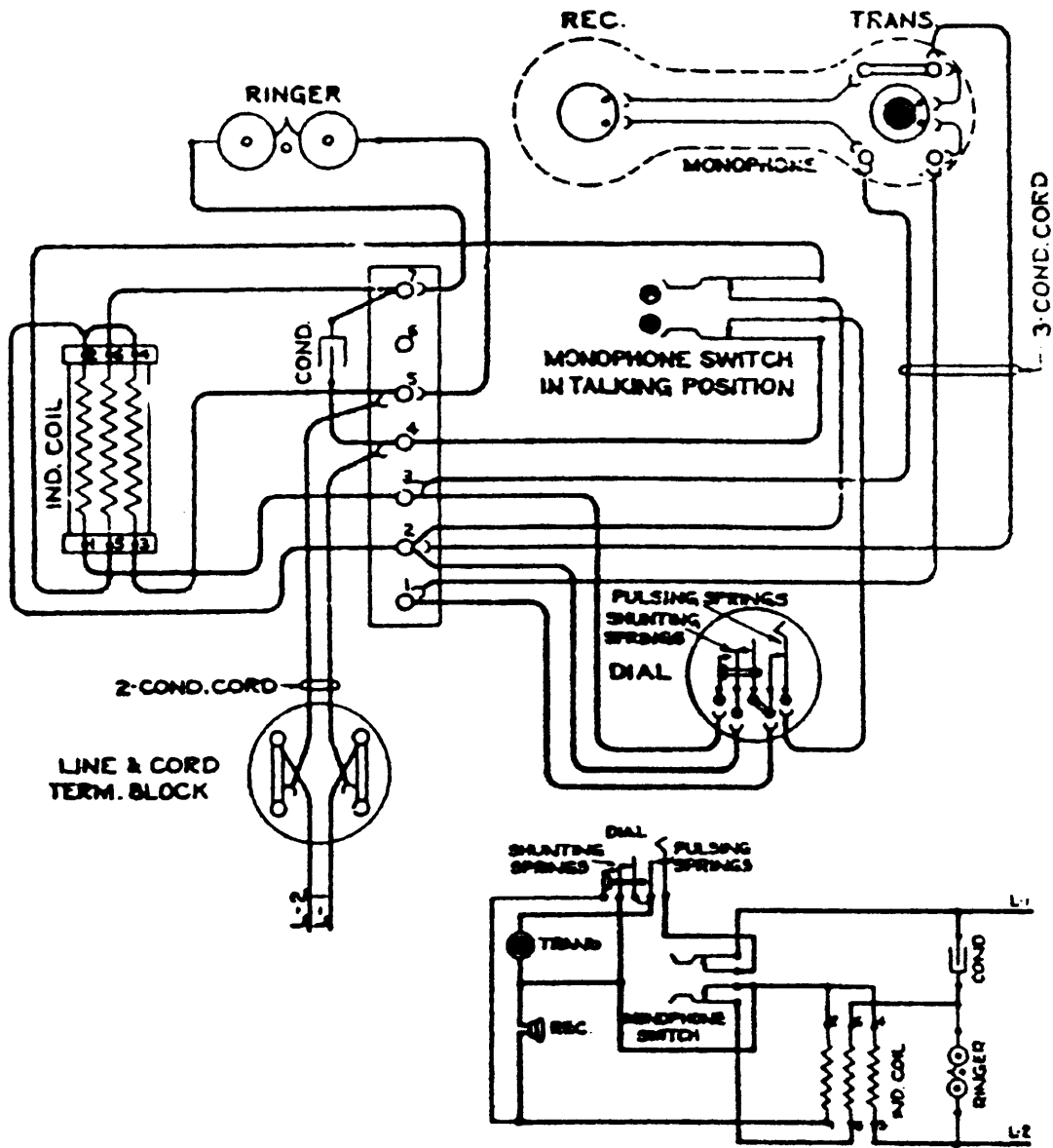
Automatic Monophone Desk Set No. 2
