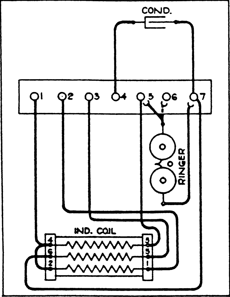
Ringer Box for Type 1 Monophone
