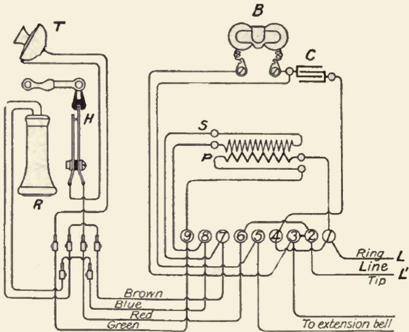
CIRCUITS OF N. E. CO. COMMON BATTERY DESK TELEPHONE
