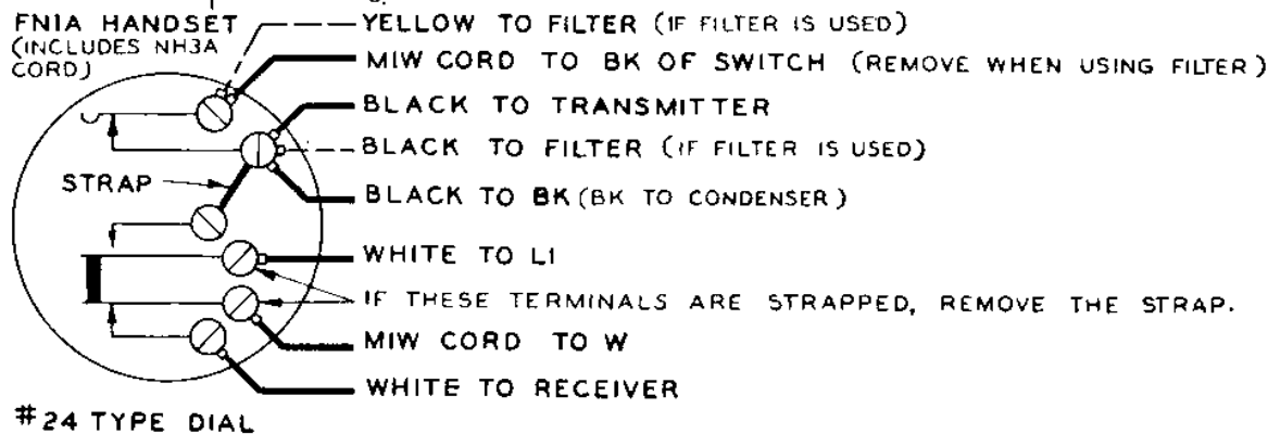
Wiring Diagram for No. 2 Type Uniphone Equipped with No. 5 Type or No. 24 Type Dial with No. 29AK Spring Assembly
