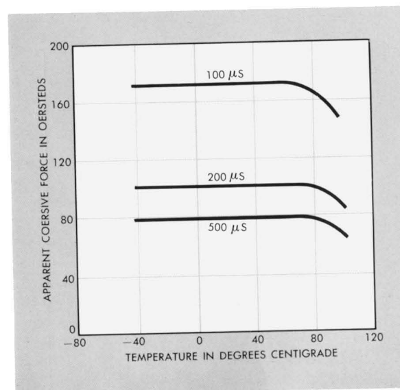
A graph of coercive force versus temperature in the Remendur developed for the parallel ferreed. Measurements are at three different pulse lengths.
