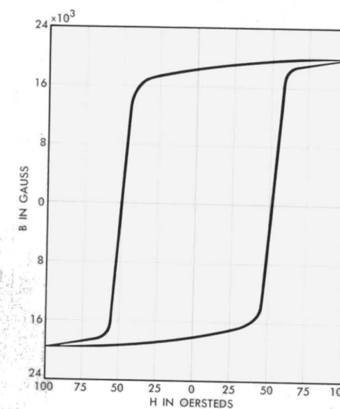
A typical dc hysteresis loop of Remendur composition developed for the series ferreed. The squareness ratio is 0.9. Illustrating the isotropic qualities of the alloy, this loop was measured at 90 degrees to the rolling direction of the processed strip.
