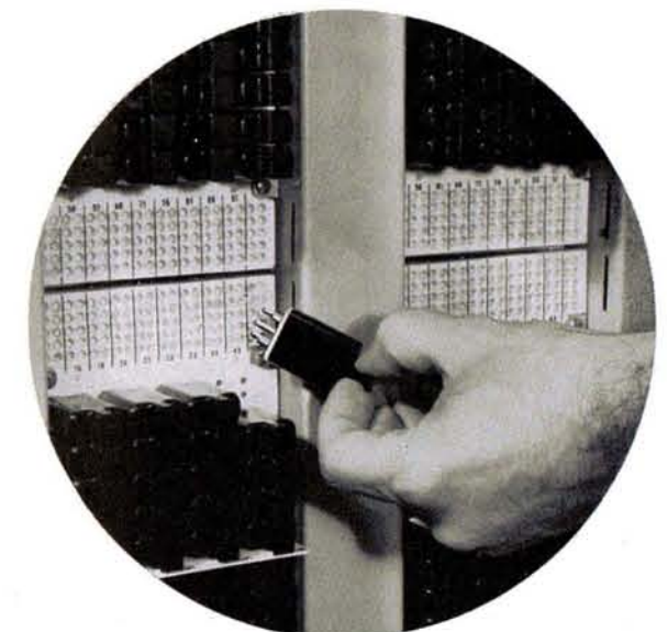
Central office equipment can be disconnected from the protector frame merely by pulling the protector forward to a detent position. This action disconnects only the central office equipment and not the outside cable pair which remains protected.
