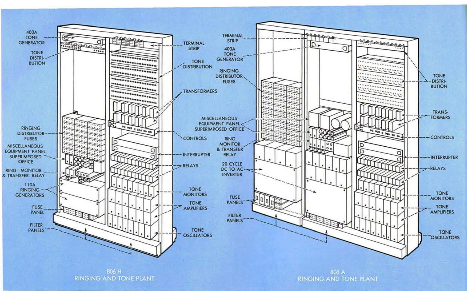
Equipment arrangements of the small and large ringing and tone plants. The tone bay is the right panel in each framework, the ringing bay is the left panel. The empty areas in each plant are reserved for the additional ringing fuses and tone splitting resistance panels, added as an office grows.
