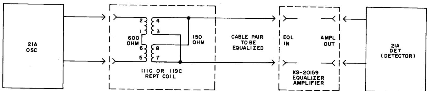
Fig. 3—Test Setup for Equalizing a Single Section Using the KS-20159 Equalizer-Amplifier
