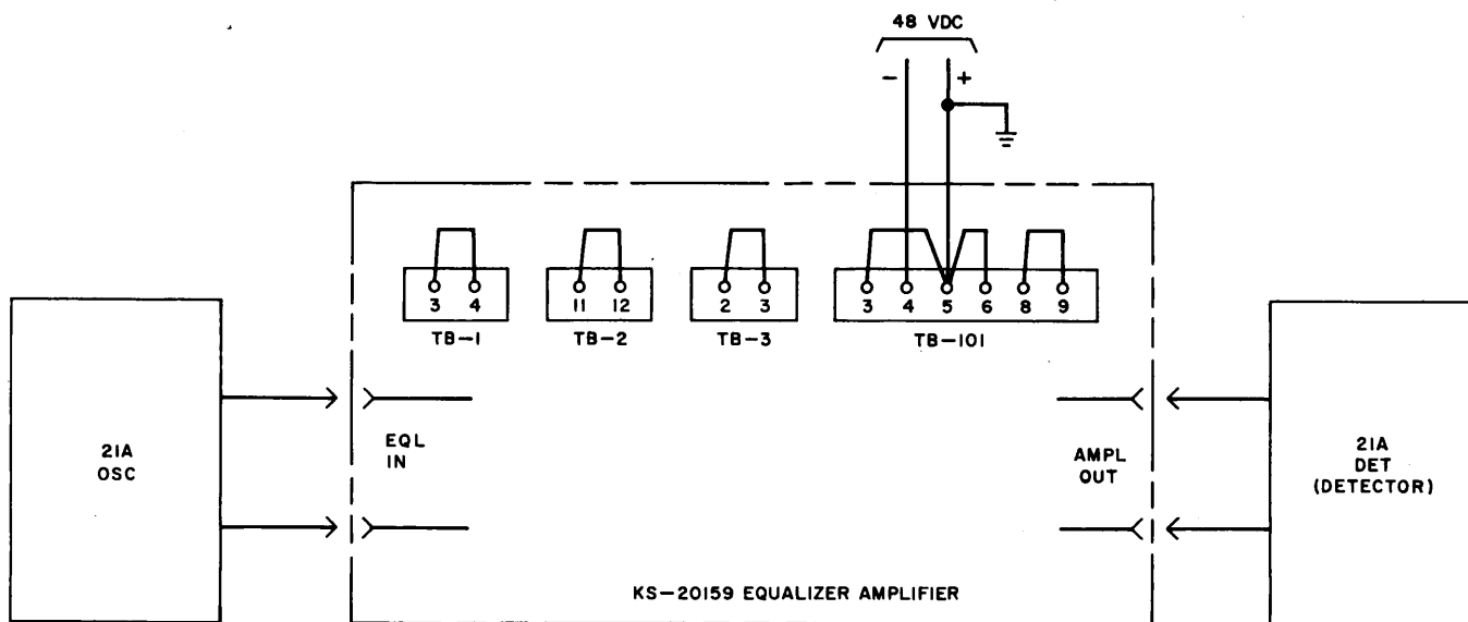
Fig. 1—Setup for Gain-Frequency Test for KS-20159 Equalizer-Amplifier
