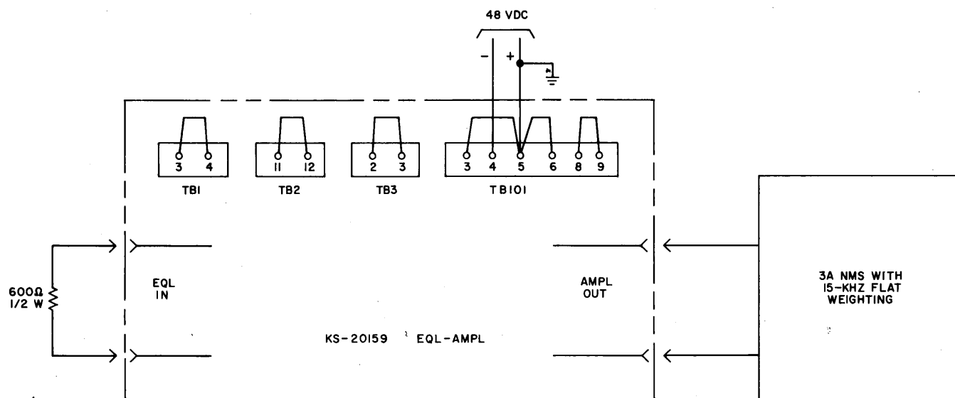
Fig. 2—Setup for Noise Test for KS-20159 Equalizer-Amplifier
