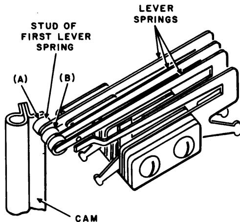
Fig. 9—Relation of Cam Spring Assembly to Cam
