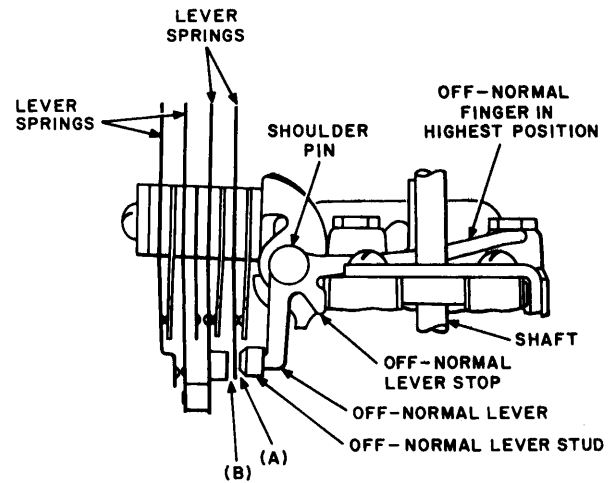
Fig. 6—Vertical Off-Normal Spring Assembly Having Pin-Mounted Off-Normal Lever
