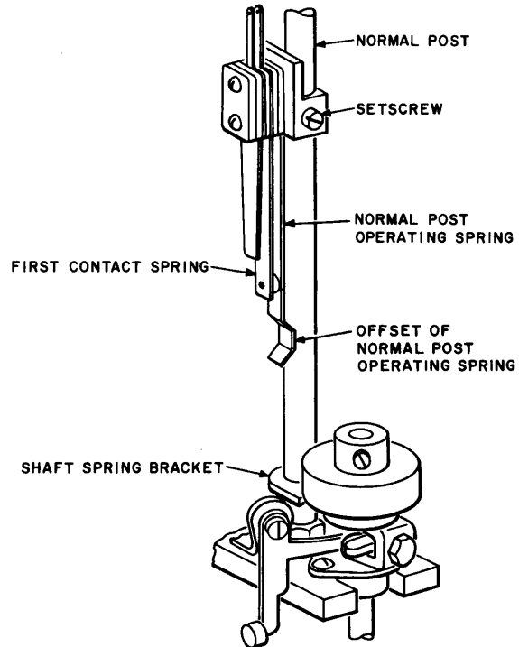
Fig. 32—Normal Post Spring Assembly Operated by Straight Shaft Spring Bracket
