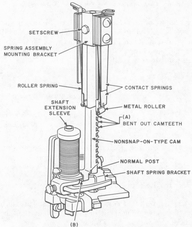
Fig. 13—Normal Post Spring Having Metal Rollers Operated by Nonsnap-On-Type Cam
