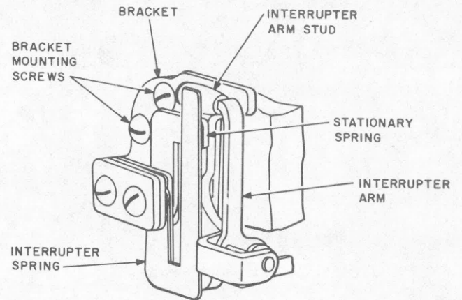
Fig. 19—Bell-Crank-Type Vertical Interrupter Spring Assembly
