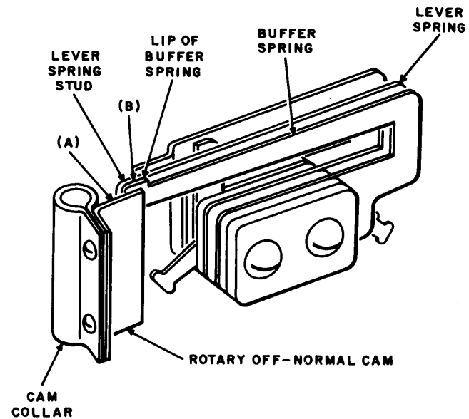
Fig. 10—Illustrating Rotary Off-Normal Spring Requirements
