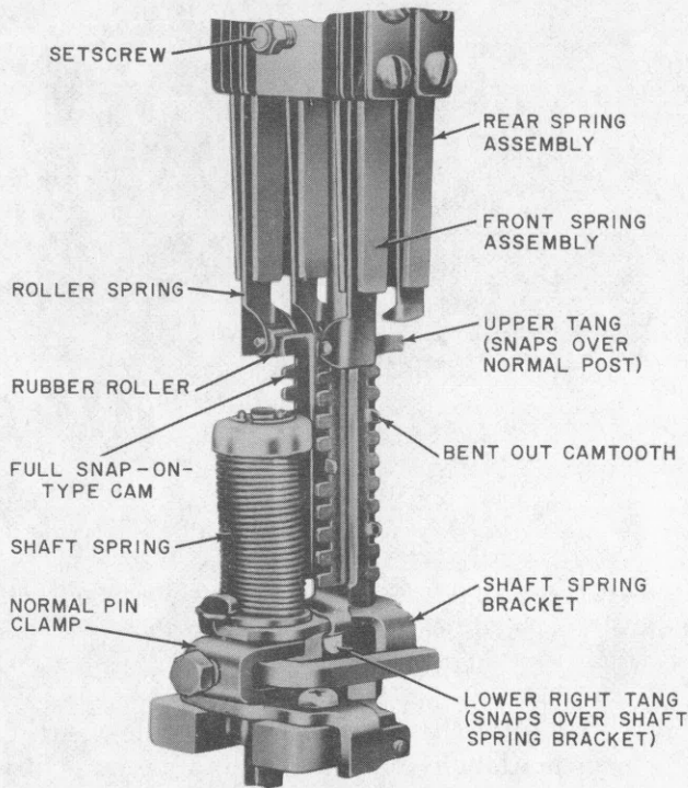
Fig. 26—Normal Post Spring Assembly Having Rubber Rollers Operated by Full Snap-On-Type Cam
