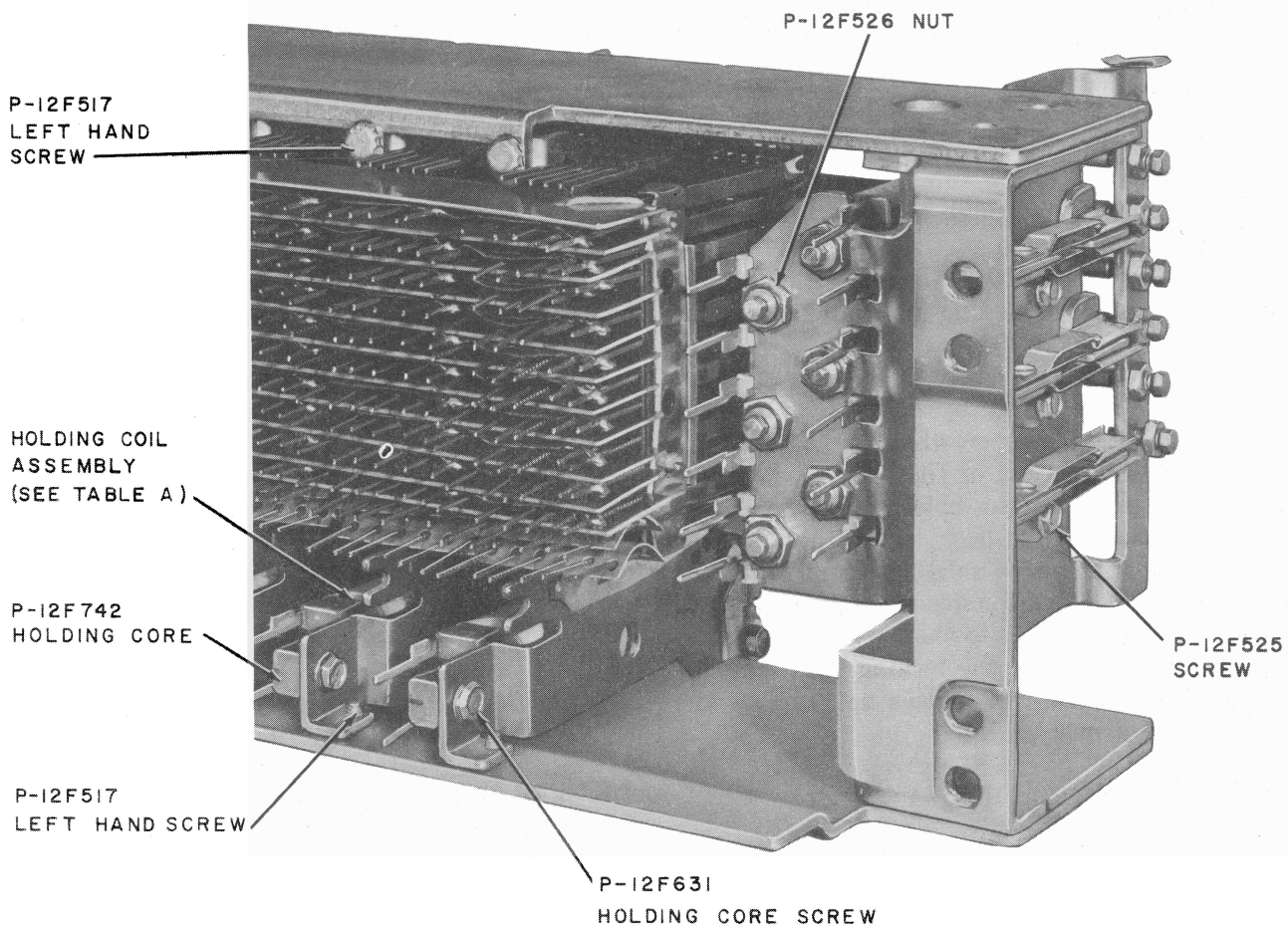
Fig. 3—Partial Rear View of Switch
