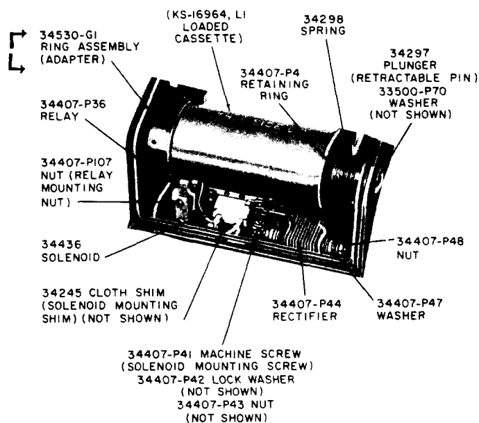
Fig. 5 — KS-14593 L2 Message Register Camera — Partial View Showing Relay, Solenoid, Rectifier, and Adapter
