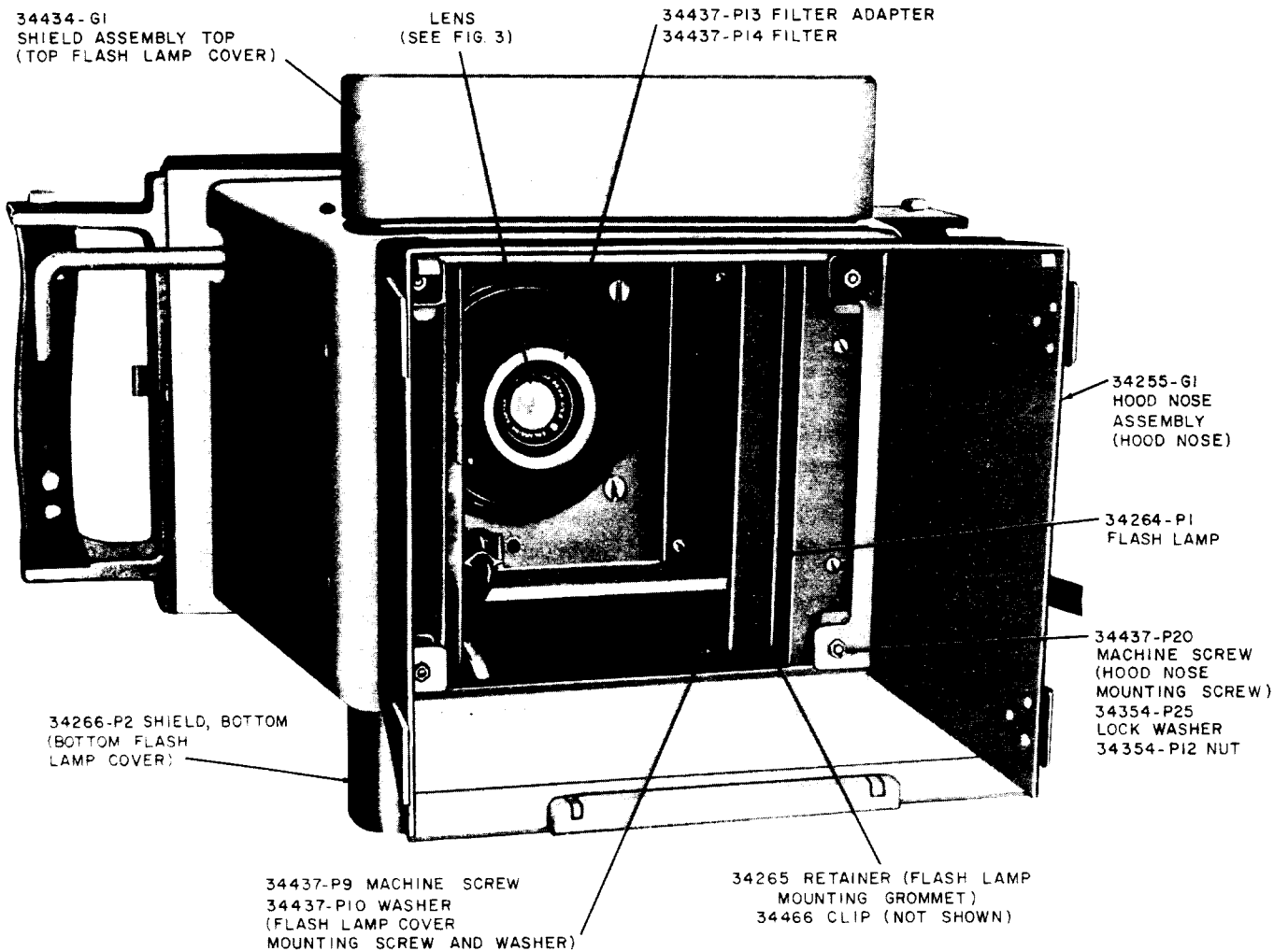
Fig. 2 — KS-14593 I2 Message Register Camera Showing Hood Nose Assembly, Filter, and Flash Lamp Covers
