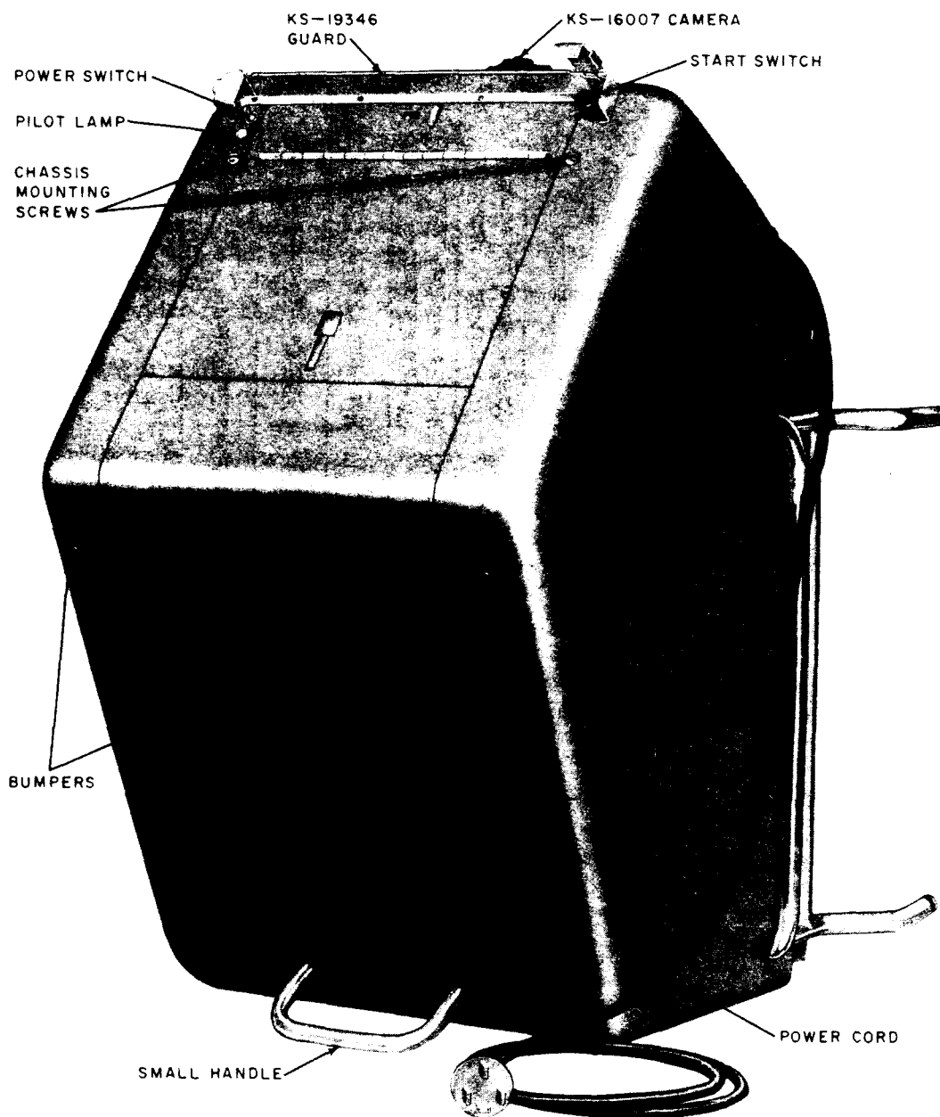
Fig. 10—KS-14776 Camera—General View
