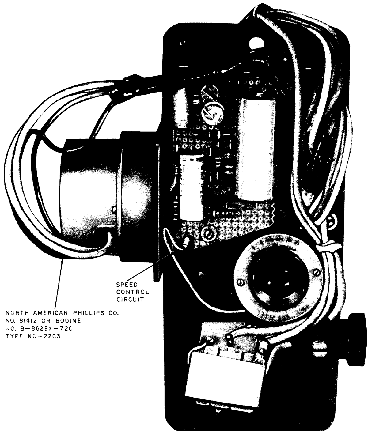
Fig. 11—♦KS-16007 Camera With KS-19438 L3 Shutter♦
