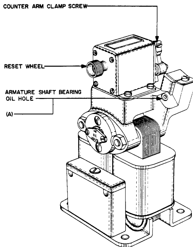
Fig. 3 — KS-7495 Magnetic Counter
