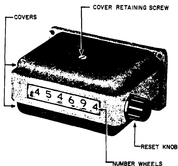
Fig. 1 - KS-14359 Magnetic Counter
