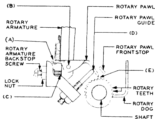
Fig. 3—Rotary Armature and Associated Parts
