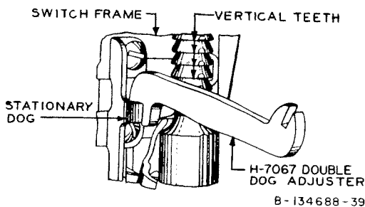
Fig. 39—Method of Adjusting the Stationary Dog Toward or Away from the Switch Frame for Horizontal Alignment
