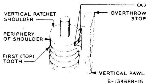
Fig. 15—Position of Vertical Pawl and Method of Checking Vertical Pawl Position
