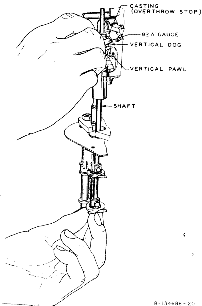
Fig. 20—Method of Checking Vertical Magnet Position
