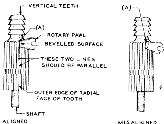
Fig. 4—Illustrating Rotary Pawl Aligned and Misaligned with Respect to the Outer Edge of the Radial Face of the Tooth
