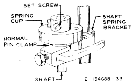
Fig. 33—Spiral-Type Shaft Spring
