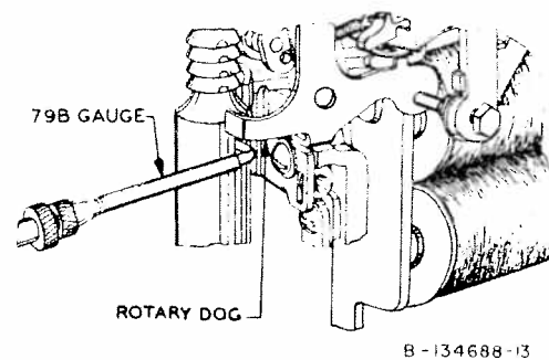
Fig. 13—Method of Measuring Shaft Spring Tension with the 79B Gauge
