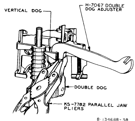
Fig. 38—Method of Adjusting the Vertical Dog Upward or Downward for Vertical Alignment or Toward or Away from the Shaft for Depth of Engagement
