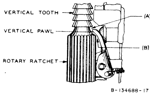
Fig. 17—Clearance Between Vertical Pawl and Vertical Teeth
