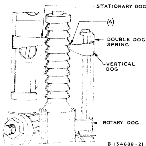
Fig. 21—Depth of Engagement of Vertical Dog
