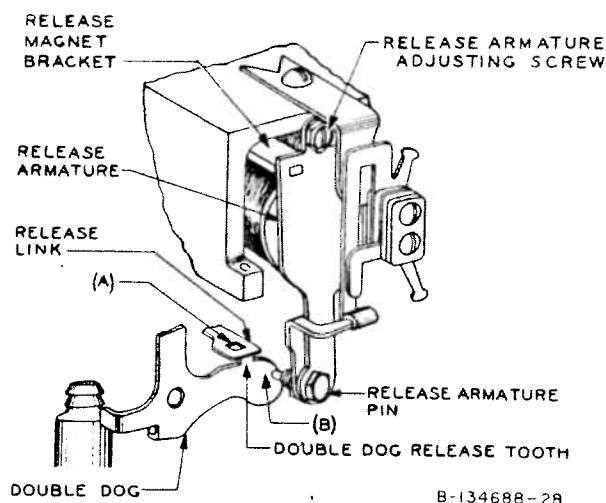
Fig. 28—Release Magnet and Earlier Type Associated Parts
