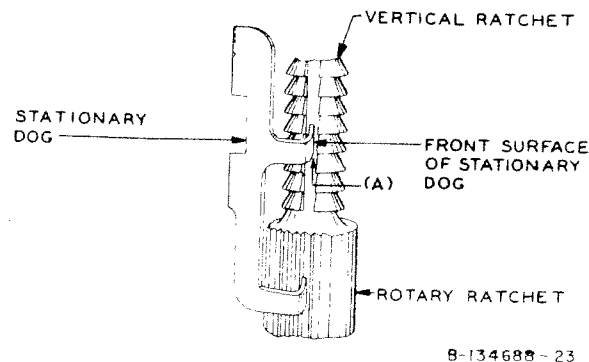
Fig. 23—Horizontal Alignment of Stationary Dog
