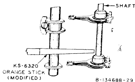
Fig. 29—Method of Checking for Bent Shaft
