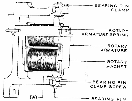
Fig. 2—Parts Associated with Rotary Magnet
