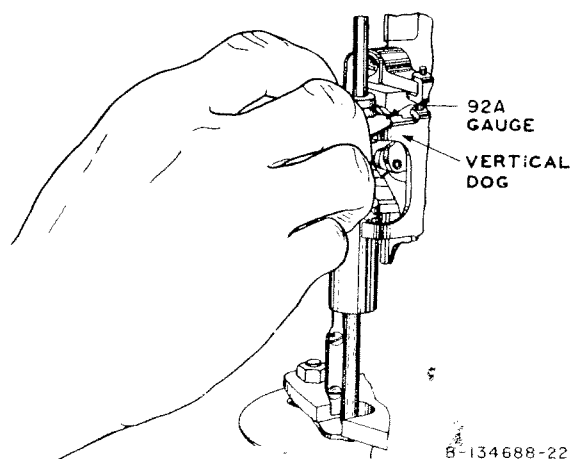
Fig. 21—Depth of Engagement of Vertical Dog
