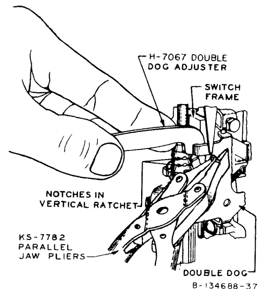
Fig. 37—Method of Adjusting the Vertical Dog to Ride in the Notches in the Vertical Ratchet
