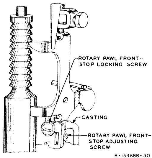
Fig. 30—Rotary Pawl Frontstop Adjustment
