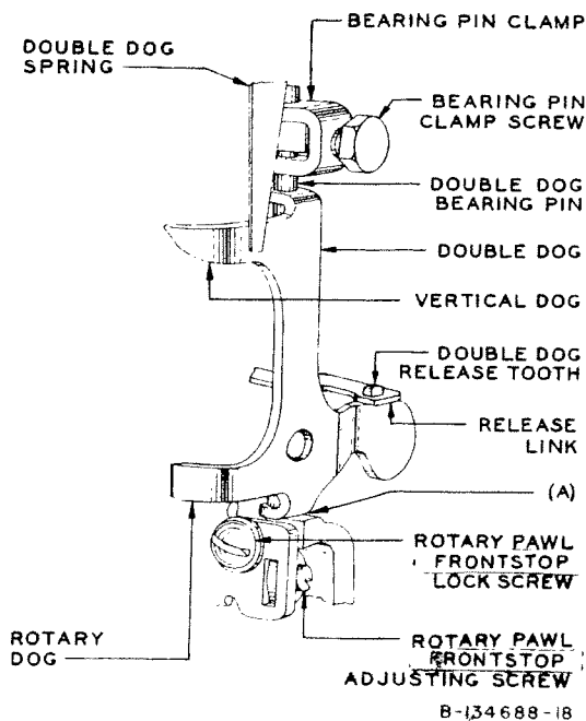
Fig. 18—Double Dog and Associated Parts
