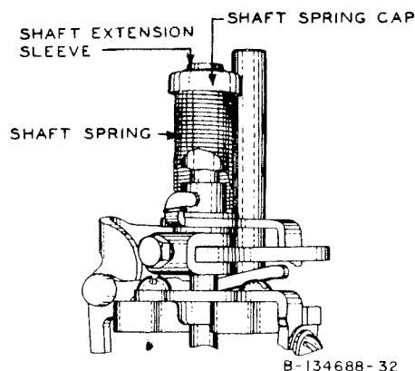
Fig. 32—Helical-Type Shaft Spring
