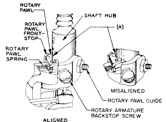
Fig. 5—Illustrating Rotary Pawl Aligned and Misaligned with Cylindrical Part of Shaft Hub
