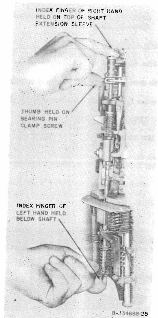
Fig. 25—Method of Raising Shaft
