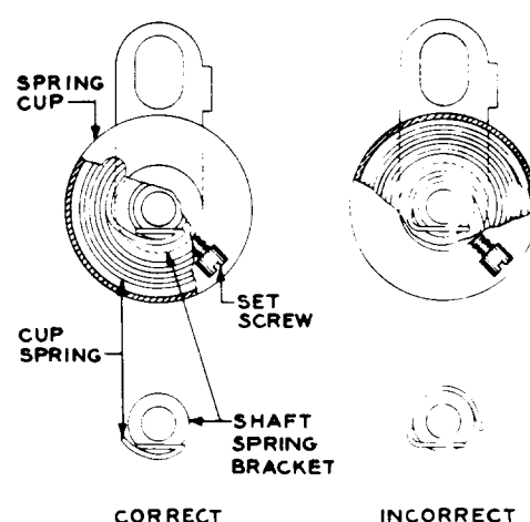
Fig. 35—Correct and Incorrect Methods of Attaching the Spiral-Type Cup Spring to the Shaft Spring Bracket
