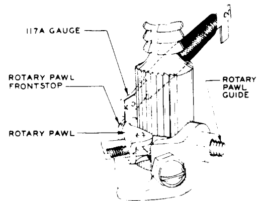
Fig. 8—Method of Measuring the Clearance Between the Rotary Pawl and Rotary Pawl Frontstop
