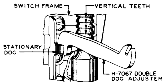
Fig. 40—Method of Adjusting the Stationary Dog Toward or Away from the Switch Frame for Horizontal Alignment
