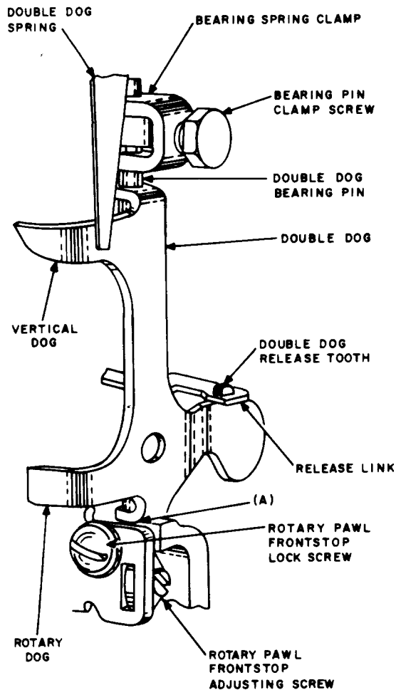
Fig. 23—Horizontal Alignment of Stationary Dog
