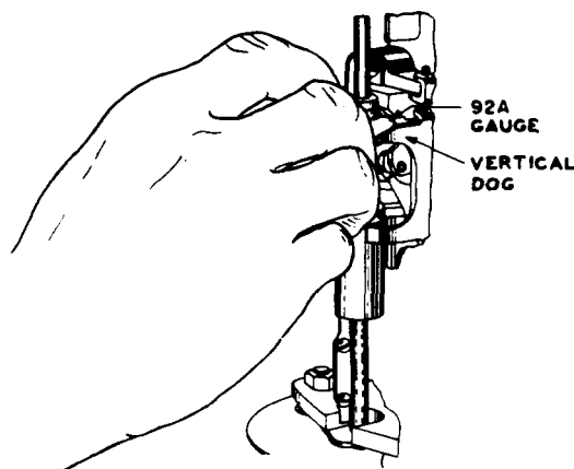
Fig. 22—Method of Checking the Depth of Engagement Between the Beveled Surface of the Vertical Tooth and the Vertical Dog
