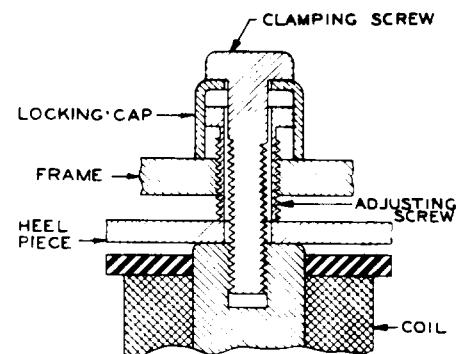
Fig. 37—Vertical Magnet Clamping Screw and Associated Parts
