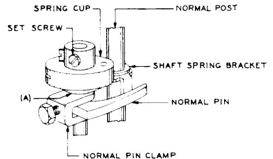
Fig. 11—Spring Cup and Associated Parts
