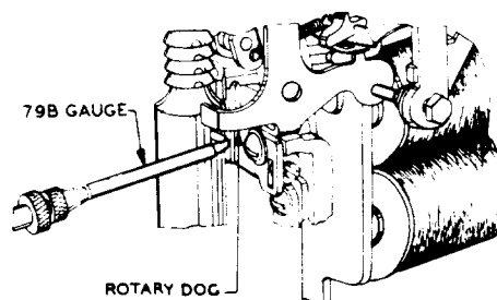
Fig. 13—Method of Measuring Shaft Spring Tension With the 79B Gauge
