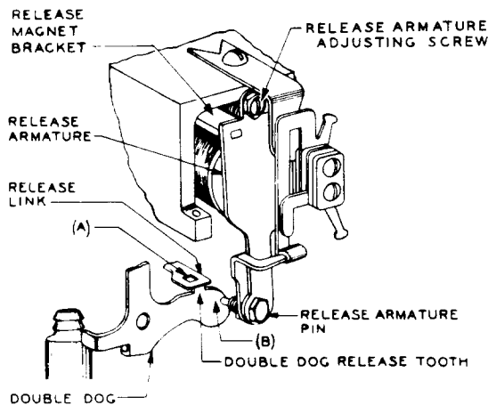
Fig. 28—Release Magnet and Earlier-Type Associated Parts
