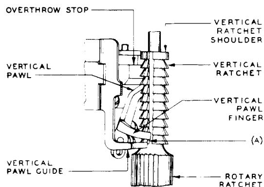
Fig. 16—Relation of Vertical Pawl to Vertical Ratchet
