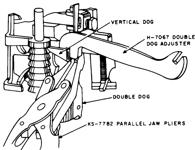
Fig. 39—Method of Adjusting the Vertical Dog Upward or Downward for Vertical Alignment or Toward or Away From the Shaft for Depth of Engagement
