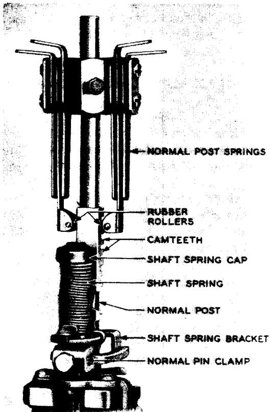
Fig. 10—Normal Post Springs Operated by Normal Post Cam and Rubber Rollers
