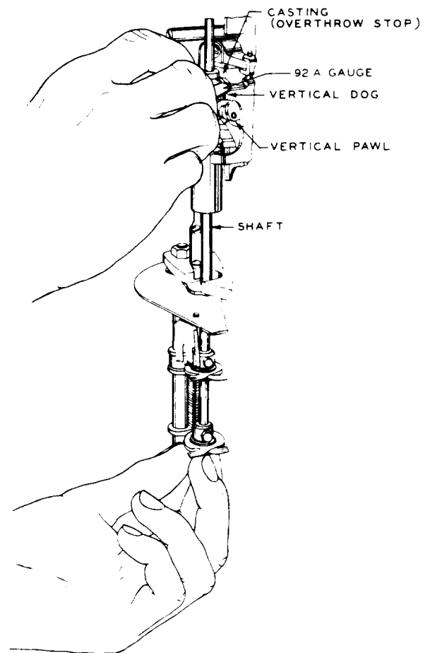
Fig. 20—Method of Checking Vertical Magnet Position
