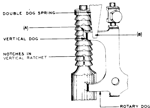
Fig. 19—Horizontal Alignment of Vertical Dog
