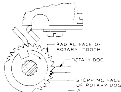
Fig. 1—Rotary Dog Alignment
