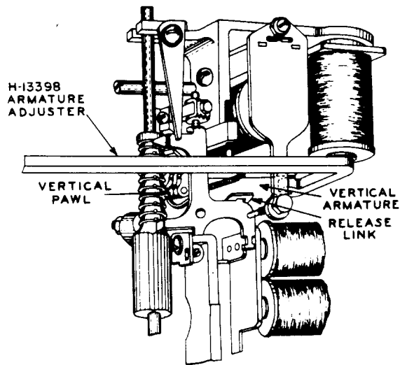
Fig. 36—Method of Adjusting Vertical Armature
