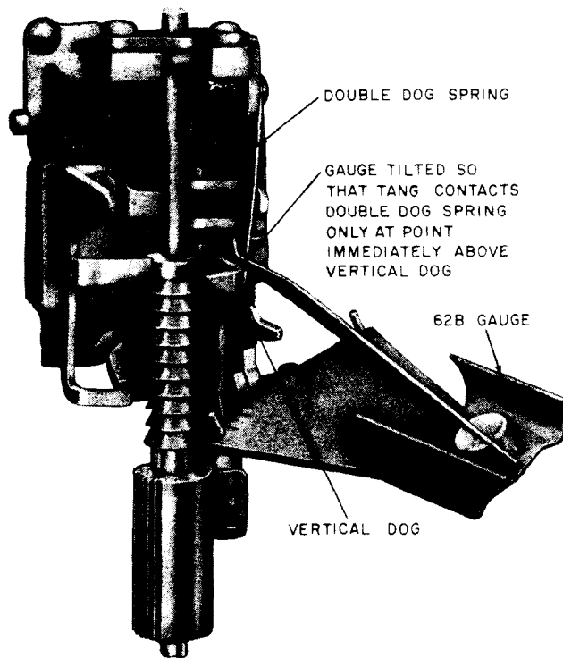
Fig. 26—Measurement of Double-Dog Spring Tension
