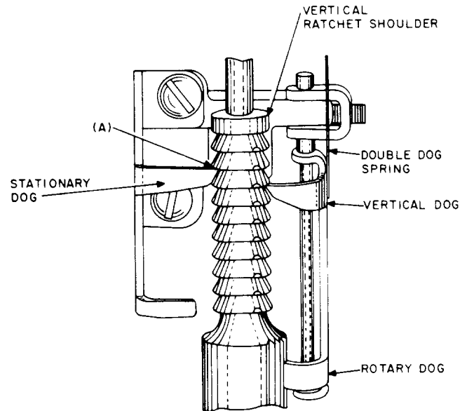
Fig. 24—Relation of Stationary Dog to the Vertical Ratchet
