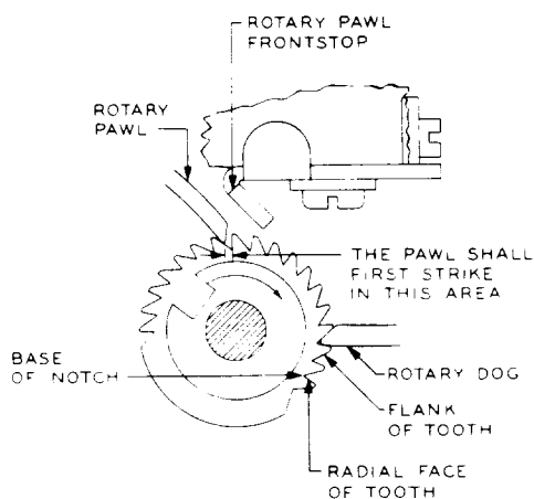
Fig. 32 — Position of Rotary Pawl as It First Strikes Rotary Ratchet
