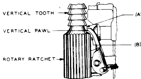
Fig. 17—Clearance Between Vertical Pawl and Vertical Teeth
