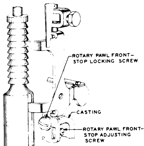
Fig. 31 — Rotary Pawl Frontstop Adjustment
