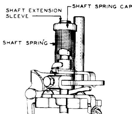
Fig. 33—Helical-Type Shaft Spring
