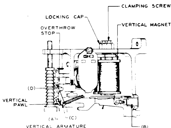
Fig. 14—Vertical Magnets and Associated Parts
