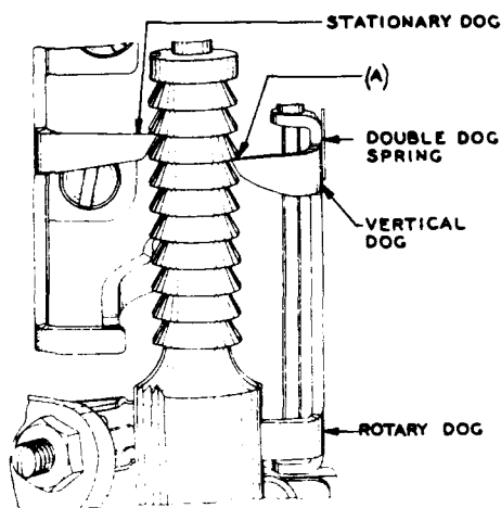
Fig. 21—Depth of Engagement of Vertical Dog
