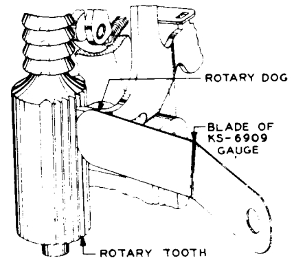
Fig. 7—Method of Checking the Clearance Between the Stopping Face of the Rotary Dog and the Radial Face of the Rotary Tooth
