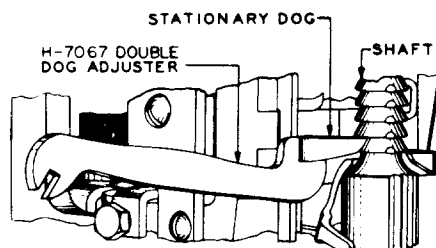
Fig. 41—Method of Adjusting the Stationary Dog Upward or Downward for Vertical Alignment or Toward or Away From the Shaft for Depth of Engagement
