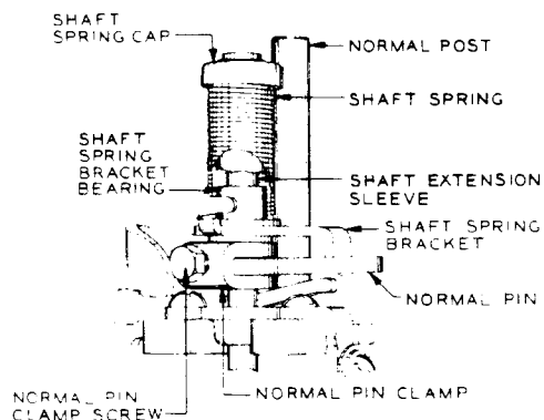
Fig. 12—Helical-Type Shaft Spring and Associated Parts
