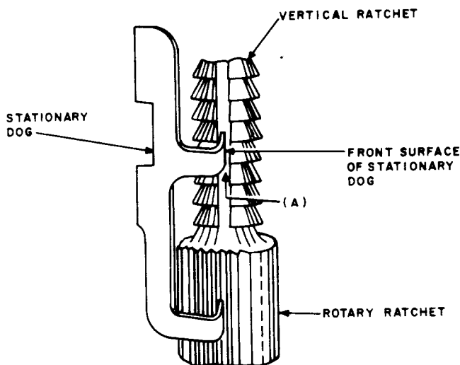
Fig. 18—Double Dog and Associated Parts
