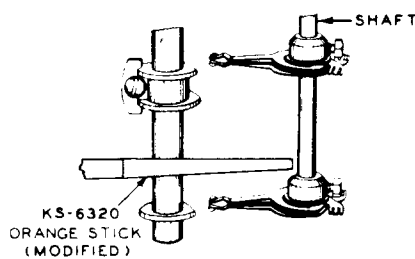
Fig. 30—Method of Checking for Bent Shaft
