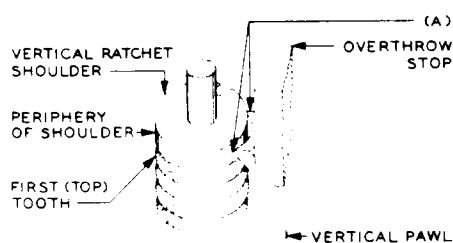
Fig. 15—Position of Vertical Pawl and Method of Checking Vertical Pawl Position
