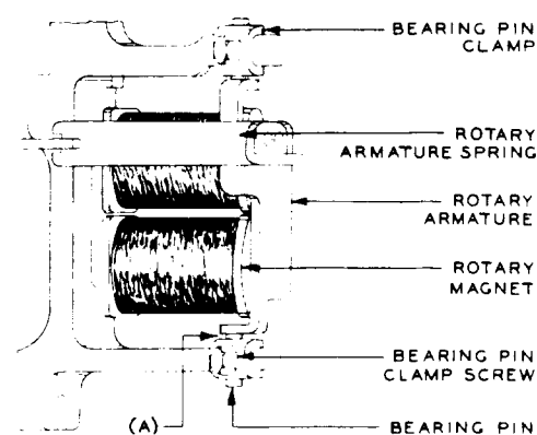
Fig. 2—Parts Associated With Rotary Magnet
