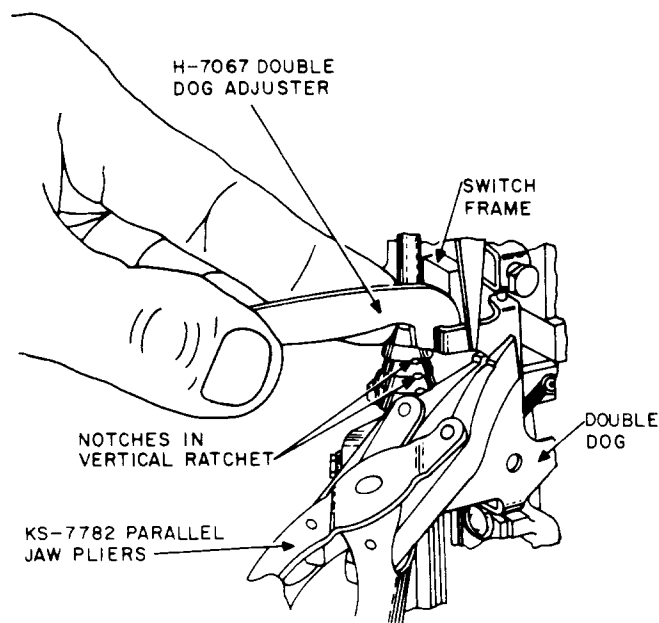
Fig. 38—Method of Adjusting the Vertical Dog to Ride in the Notches in the Vertical Ratchet
