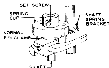
Fig. 34—Spiral-Type Shaft Spring
