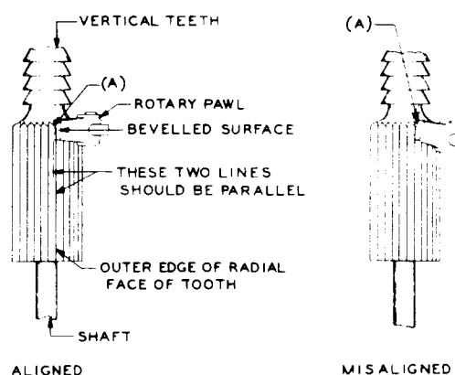
Fig. 4—Illustrating Rotary Pawl Aligned and Misaligned With Respect to the Outer Edge of the Radial Face of the Tooth
