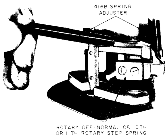
Fig. 24—Method of Adjusting U-Shaped Springs on Rotary Off-Normal or Tenth or Eleventh Rotary Step Spring Assemblies
