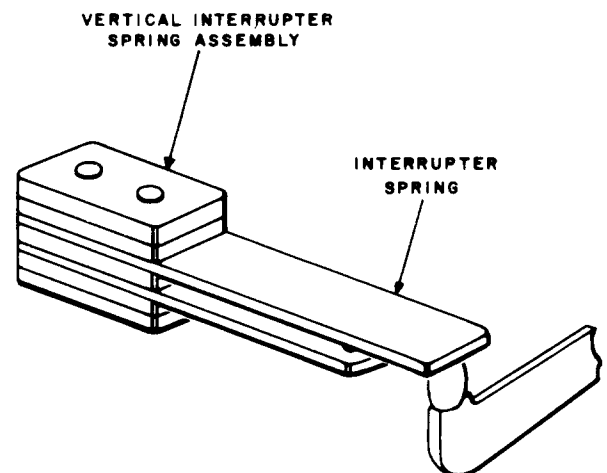
Fig. 4—Vertical Interrupter Spring Assembly of Type Operated by Vertical Armature Arm
