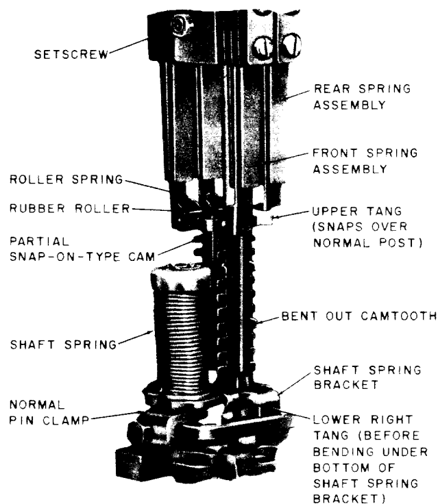
Fig. 27—Normal Post Spring Assembly Having Rubber Rollers Operated by Partial Snap-On-Type Cam
