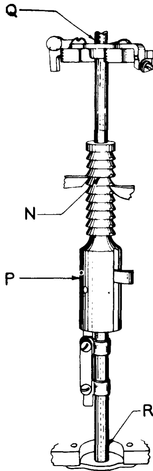
Fig. 14—Lubrication Points for Shaft and Associated Parts of 198-Type Switches Covered in Table A
