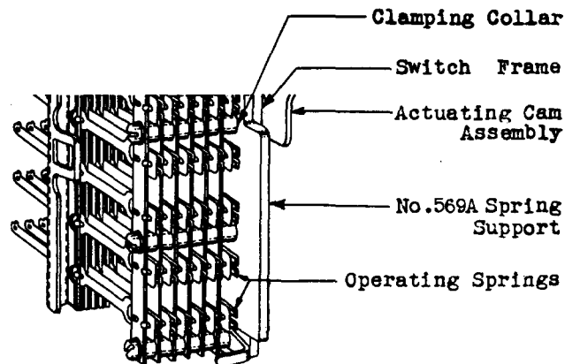
Fig. 2 - Position of Spring Support when Removing and Replacing Actuating Plate
