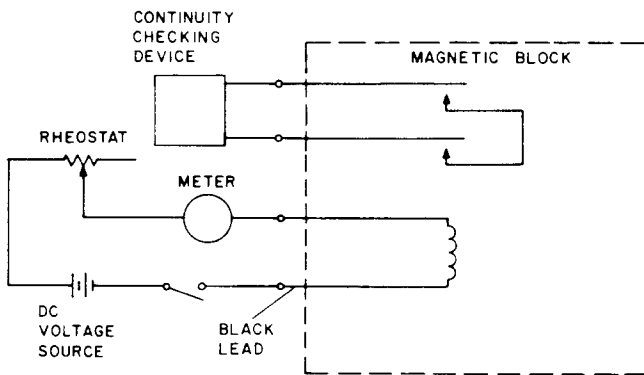
Fig. 18—Indicating Circuit
