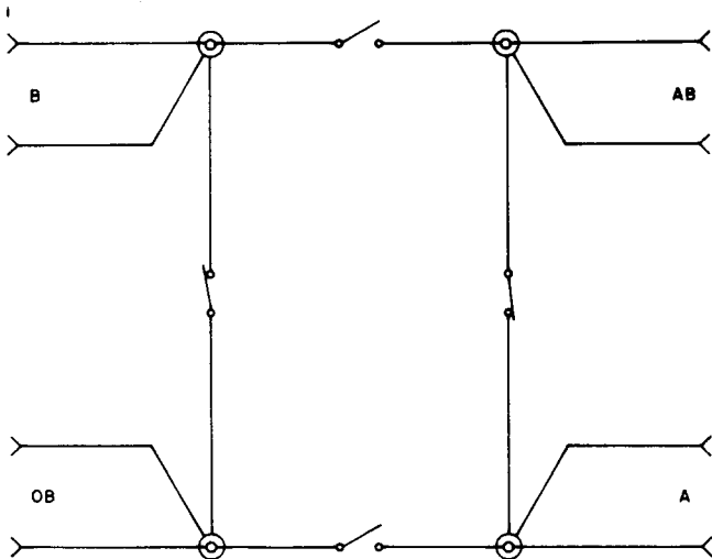
Fig. 6—223E Coaxial Switch Schematic (Shown in Normal Released Condition)
