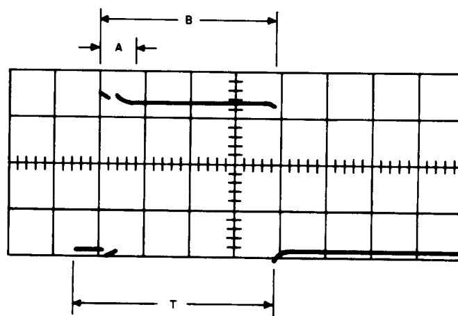
Fig. 23—Timing Chart (S1 to OFF)
