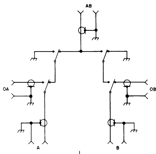
Fig. 5—223A Coaxial Switch Schematic (Shown in Normal Released Condition)
