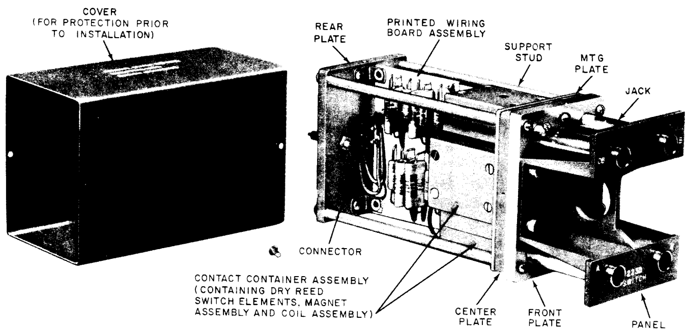
Fig. 4—223D Coaxial Switch, Cover Removed
