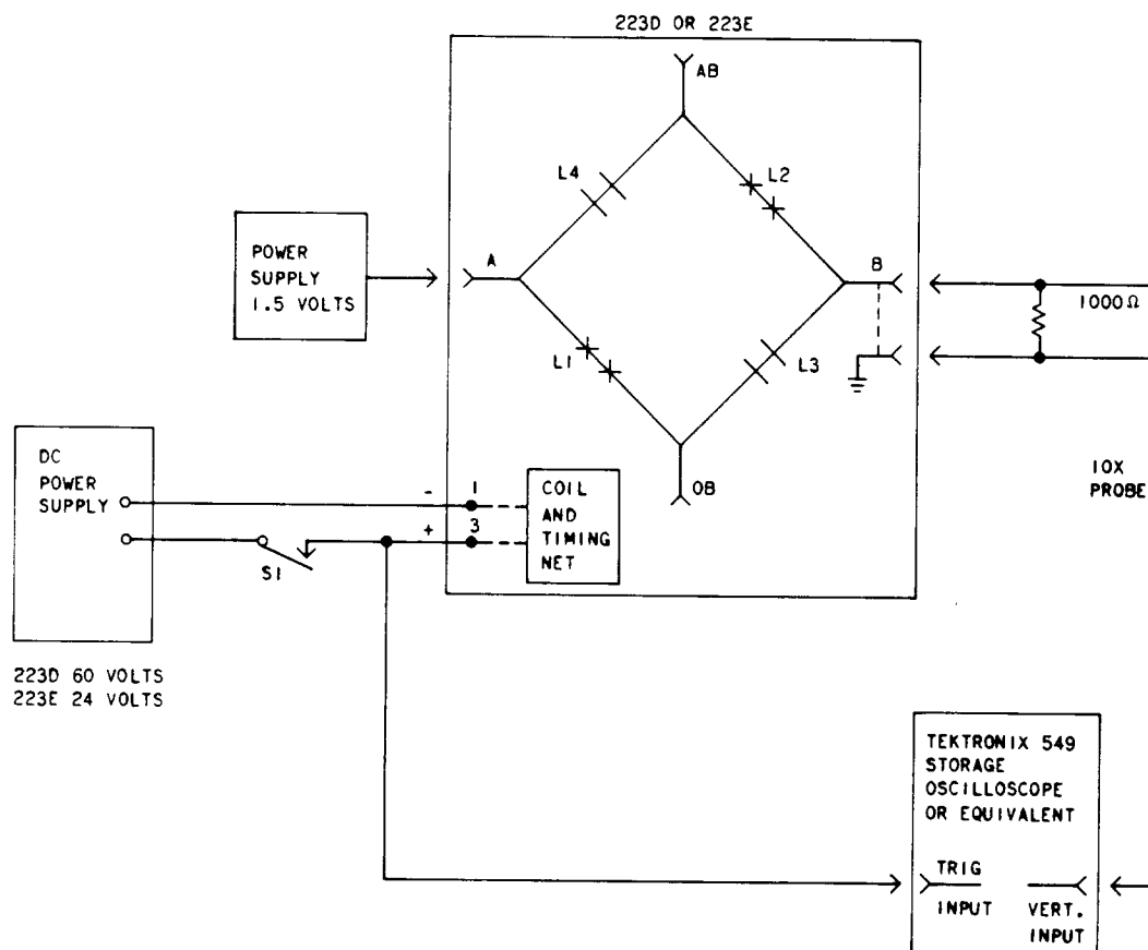
Fig. 21—Bridging Time Check Test Circuit
