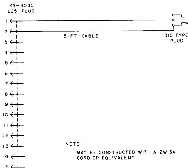
Fig. 7—Power Cable to Connect 35-Type Test Set to J68333 Test Bench
