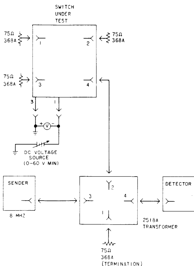
Fig. 20—Return Loss Test Circuit
