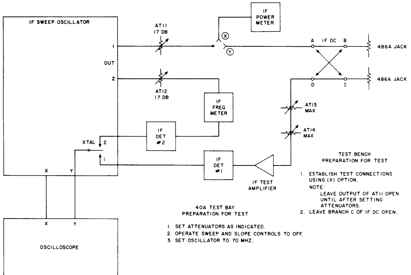
Fig. 11—Test Arrangement for Return Loss Measurement of the 223-Type Switch Using 40A Test Bay
