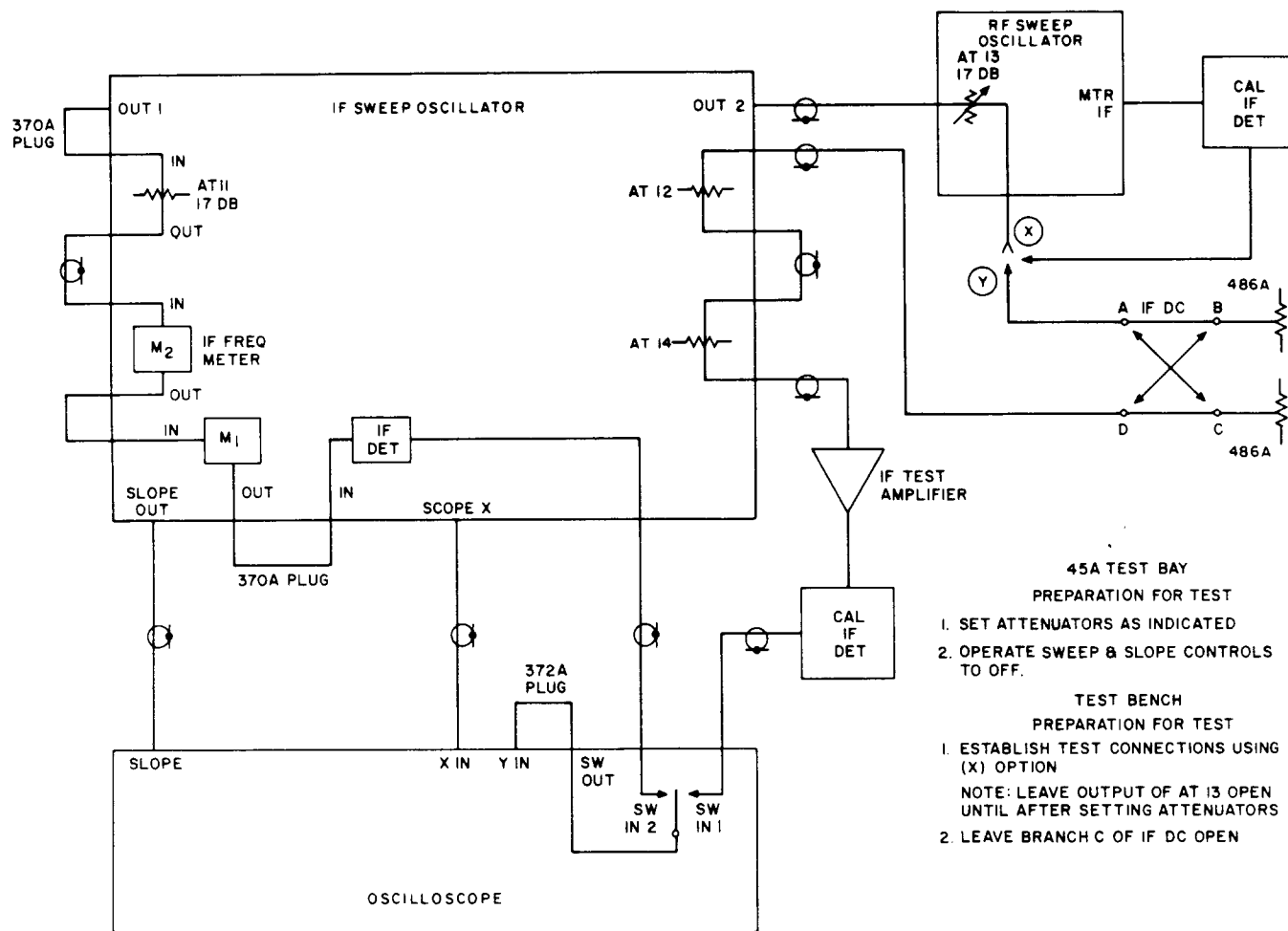
Fig. 12—Test Arrangement for Return Loss Measurement of the 223-Type Switch Using 45A Test Bay
