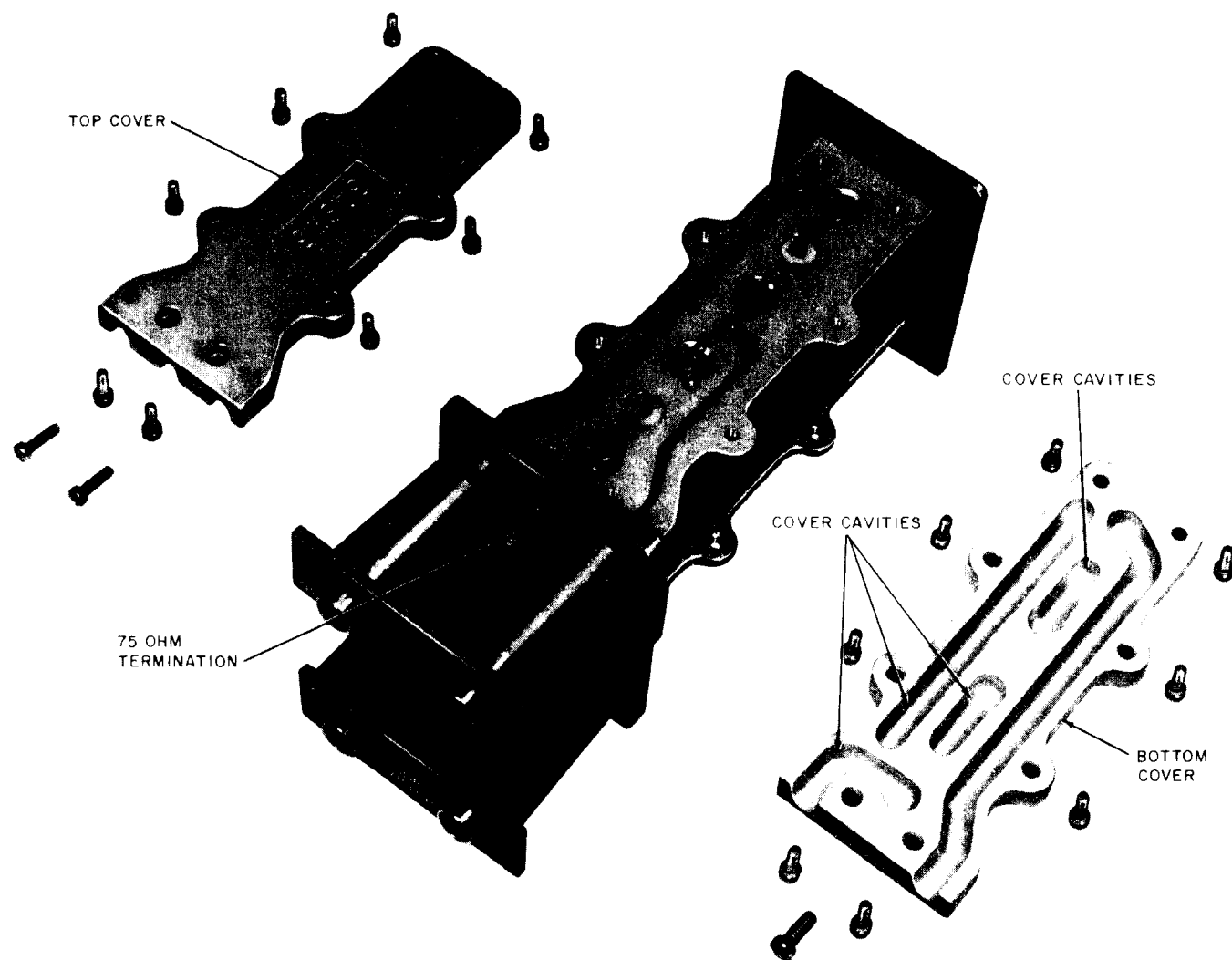
Fig. 2—223B Coaxial Switch, Disassembled, Top View
