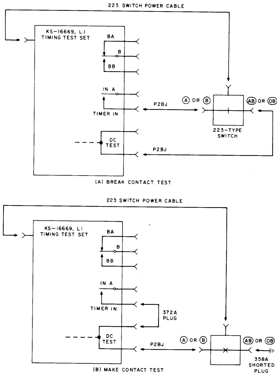
Fig. 16—Test Arrangement for 223-Type Switch Timing Tests
