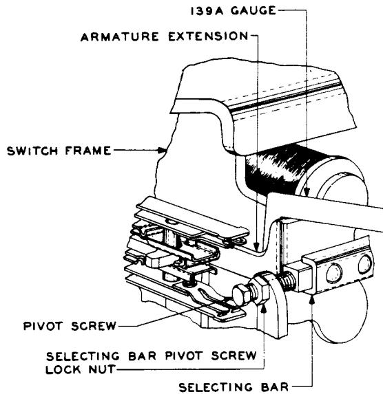
Fig. D — Method of Checking Clearance Between Wide Portion of Selecting Armature Extension and Switch Frame
