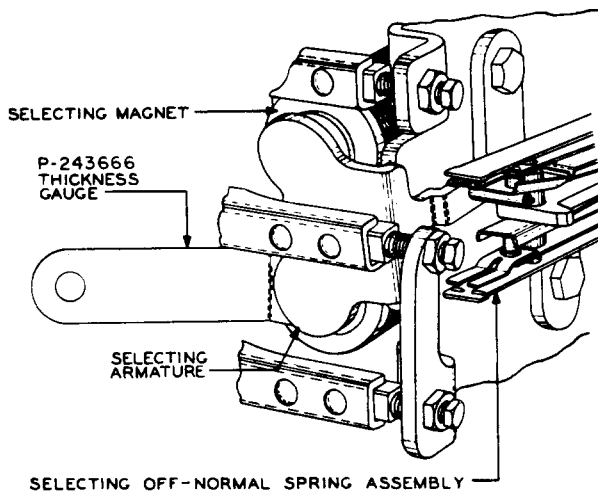
Fig. O — Method of Checking Front Contact Make on Selecting Off-Normal Spring Combination Fig. 104
