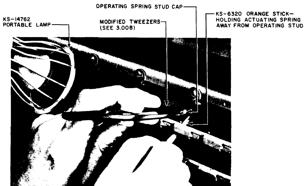
Fig. AC — Method of Mounting Operating Stud Cap
