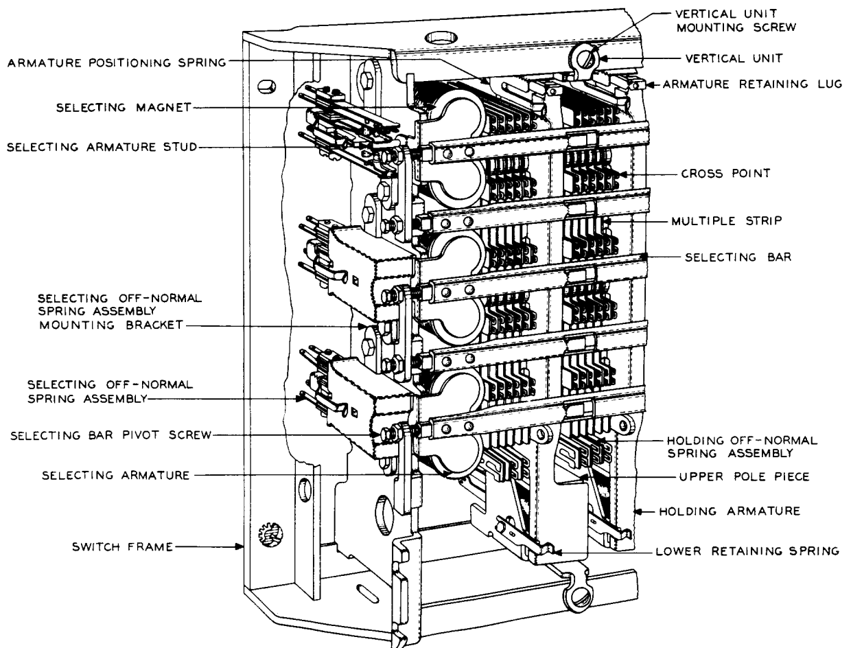
Fig. B – General View of Switch Equipped With Vertical Units Having Armature Retaining Lug
