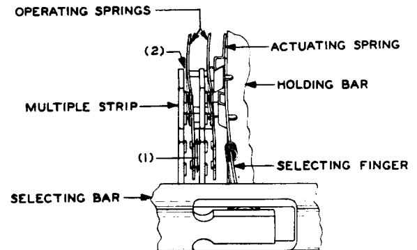
Fig. Q - Spring Clearance Requirements
