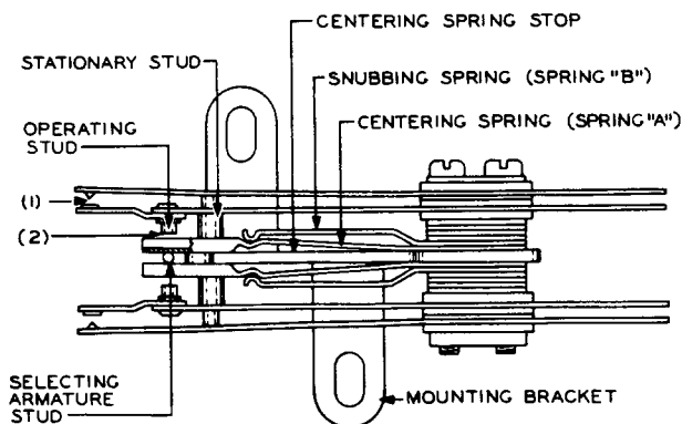
Fig. N — Selecting Off-Normal Spring Assembly With Selecting Unit Normal
