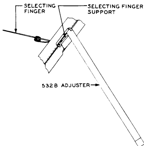
Fig. Y – Method of Adjusting Selecting Finger to Left
