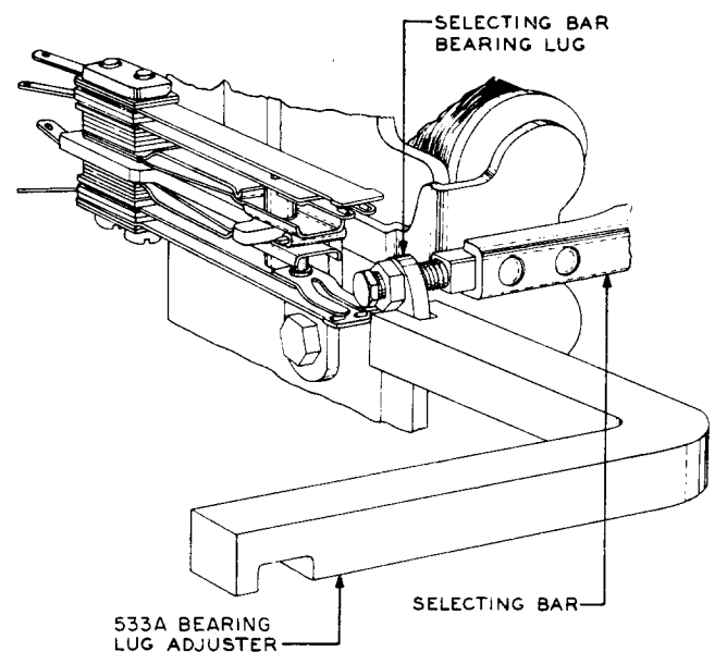
Fig. U – Method of Adjusting Selecting Bar Bearing Lug to Eliminate Bind
