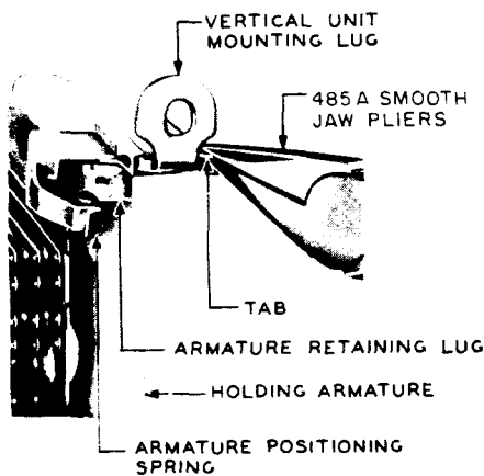
Fig. AG – Method of Removing Armature Positioning Spring
