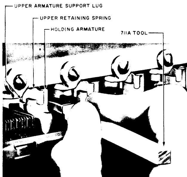
Fig. AD – Method of Adjusting Upper Armature Support Lug
