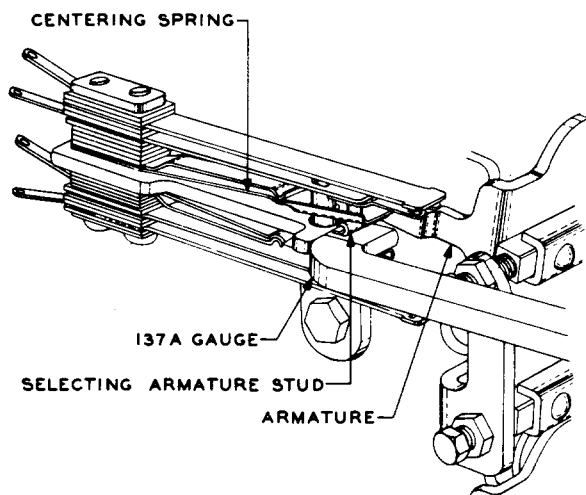
Fig. G - Method of Gauging Armature Travel
