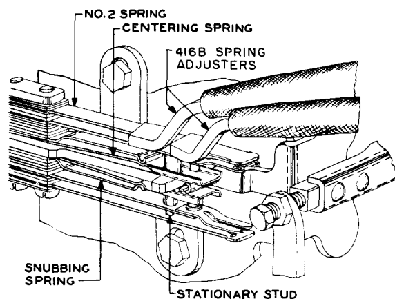
Fig. AA – Method of Adjusting No. 2 Spring for Contact Separation and Front Contact Make
