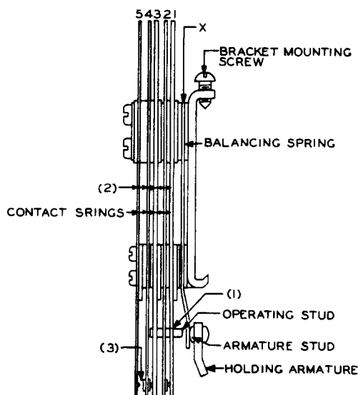
Fig. 5 - Clamp-Type Holding Off-Normal Spring Assembly
