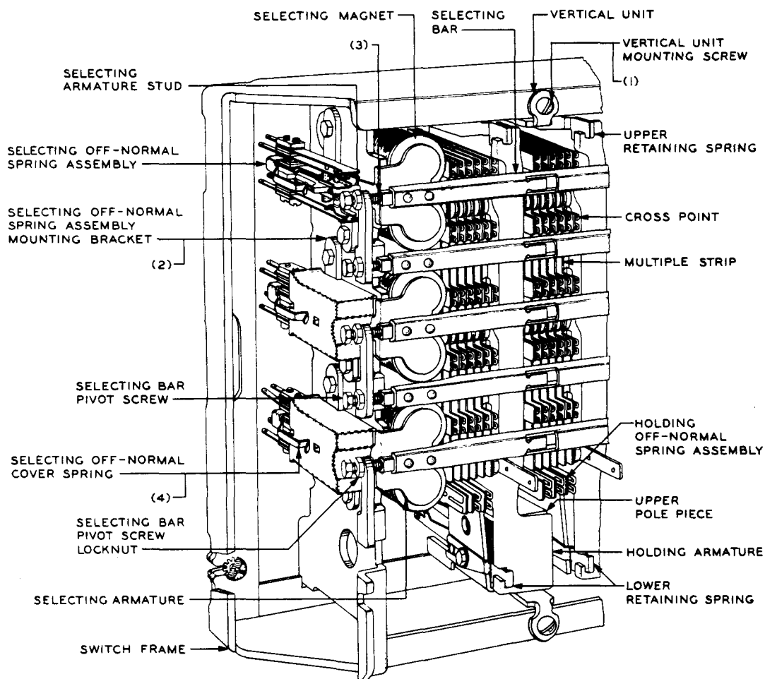
Fig. A - General View of Switch Equipped With Vertical Units Having Upper and Lower Retaining Springs
