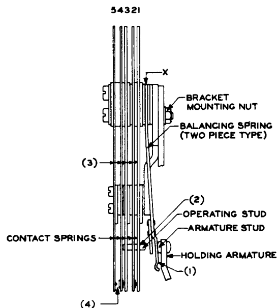
Fig. R — Bracket-Type Holding Off-Normal Spring Assembly
