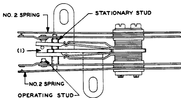
Fig. F - Selecting Off-Normal Spring Assembly With Selecting Unit Operated
