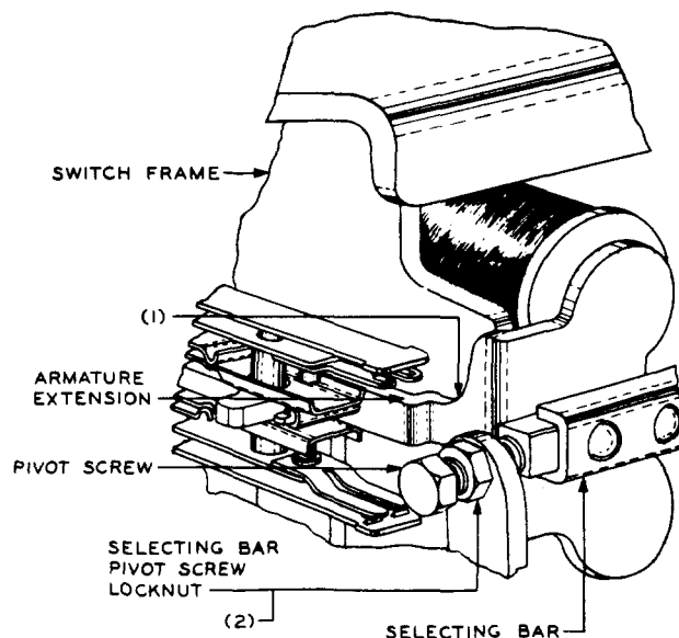
Fig. C — Clearance Between Selecting Armature Extension and Switch Frame
