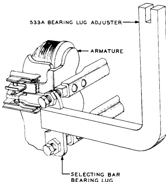
Fig. W – Method of Adjusting Selecting Bar Bearing Lug for Armature Travel
