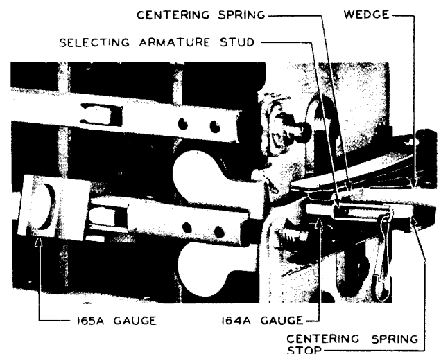
Fig. J - Method of Checking Position of Selecting Finger Using the 164A and 165A Gauges
