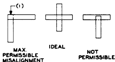
Fig. K — Alignment of Standard Contacts — Plan View of Contact Surfaces
