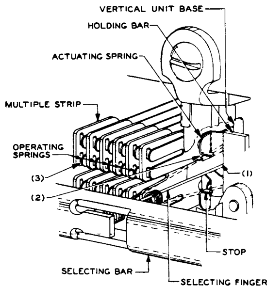
Fig. H - Position of Selecting Finger
