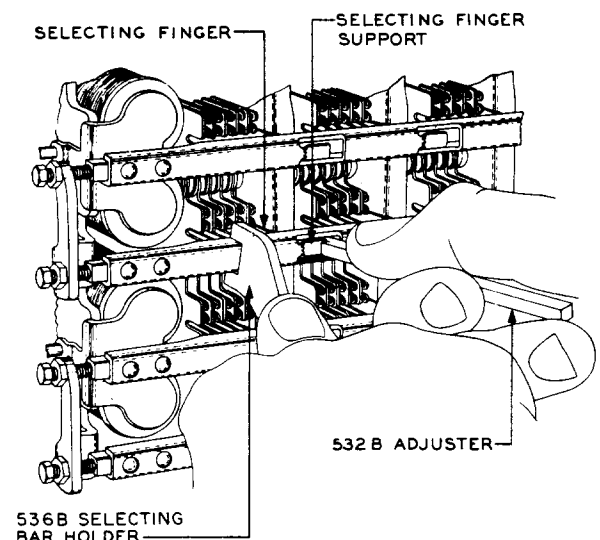
Fig. X – Method of Adjusting Selecting Finger Support
