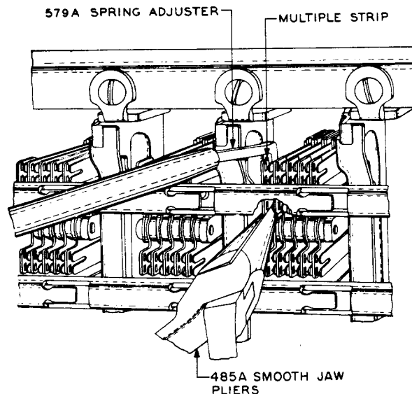
Fig. AB – Method of Adjusting Contact Multiple
