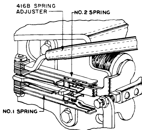
Fig. Z – Method of Adjusting Springs for Straightness and Clearance
