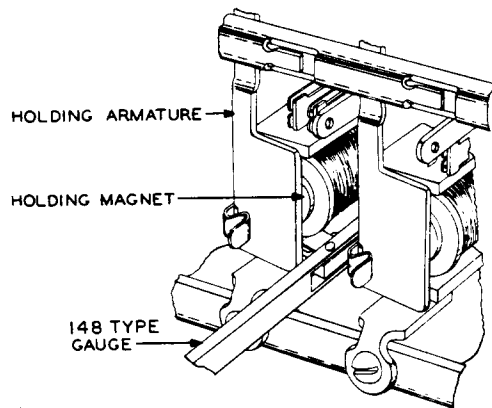
Fig. P - Thickness Gauge in Position at Standard Point of Measurement
