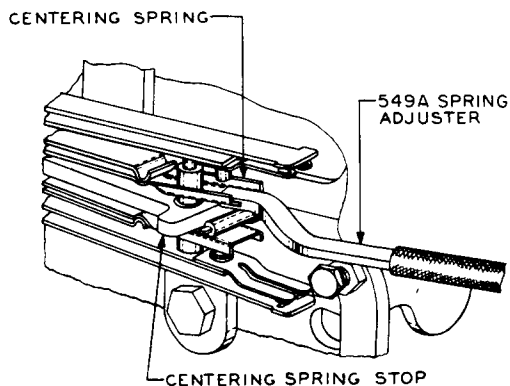
Fig. V – Method of Adjusting Centering Spring
