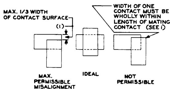
Fig. L — Alignment of Heavy Contacts — Plan View of Contact Surfaces
