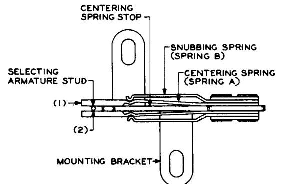
Fig. E — Centering Unit in Normal Position
