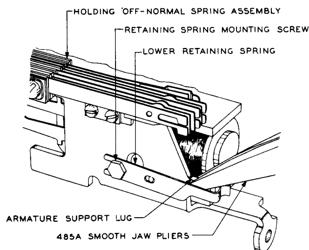
Fig. AF – Method of Adjusting Lower Armature Support Lug
