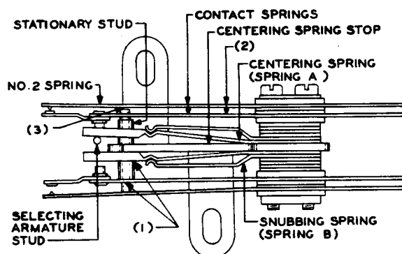
Fig. M — Selecting Off-Normal Spring Assembly With Selecting Unit Operated
