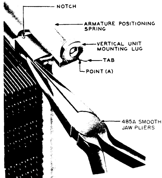
Fig. AH – Method of Mounting Armature Positioning Spring
