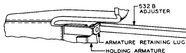
Fig. AE – Method of Adjusting Armature Retaining Lug of Vertical Units Having Lower Retaining Springs Only
