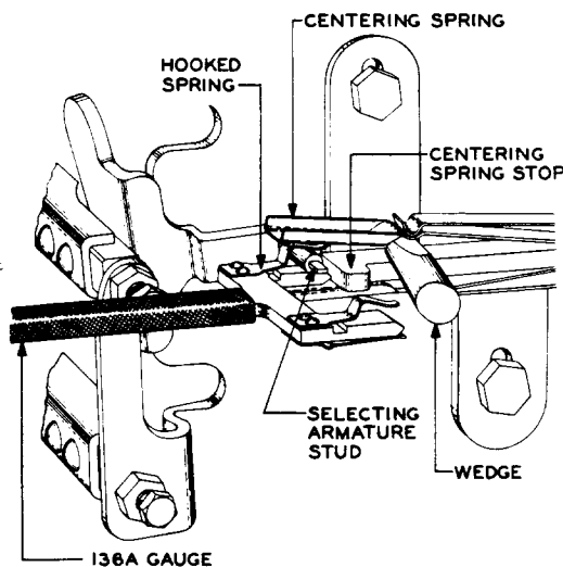
Fig. I - Method of Checking Position of Selecting Finger
